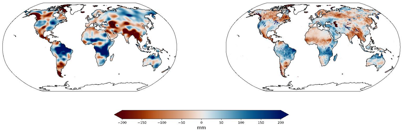
85 Figure 1. Terrestrial water storage anomalies (TWSA) for the example of May 2023. Left figure: TWSA based on postprocessed Level-3 data from GRACE with VDK filtering, GravIS Version 5. Right figure: Storage anomaly as the sum of the observation- and model-based WSC data sets used in this study (root-zone soil moisture, snow water equivalent, surface water storage, glacier mass change), aggregated to a common 0.5^\circ resolution, see Chapter 2 for details in the data sets.
