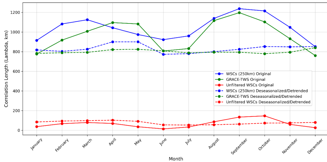
350 Figure 6. Mean monthly spatial autocorrelation lengths (based on the Weibull model) of 4WSC (unfiltered in red, 250 km Gaussian filtered 355 in blue) and GRACE-based TWSA (in green) for the original (solid lines) and the de-seasonalized/de-trended data (dashed lines).
