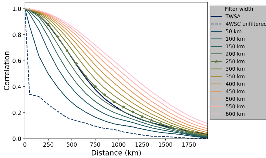
400 Figure 9: Empirical global autocorrelation functions of 4WSC after Gaussian filtering with different filter widths, compared to the GRACE- based TWSA autocorrelation function.
