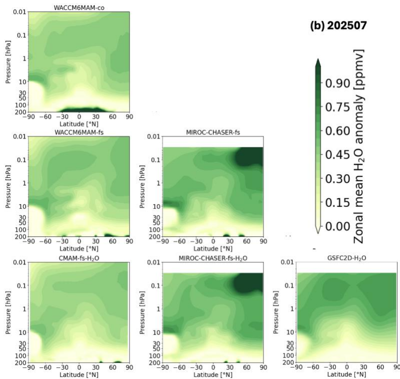
Figure A3: Latitude–pressure distribution of simulated zonal-mean water vapor anomalies in the upper atmosphere following the Hunga eruption, shown for (a) January 2025 and (b) July 2025. Anomalies are computed as differences between the ensemble mean of the experiment and control simulations.
