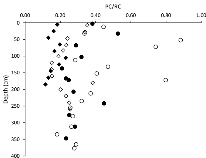
Figure 65: Sediment profiles of the ratio of pyrolysable carbon to refractory carbon (PC/RC). The ratio decreases not only with depth but also with the evolution of the lakes, as organic matter becomes more refractory. The uncertainty of the data is smaller than the symbol (Circles-circles – BTL, Diamonds – GSL, full symbols – Center, Empty symbols – Edge of lakes).
