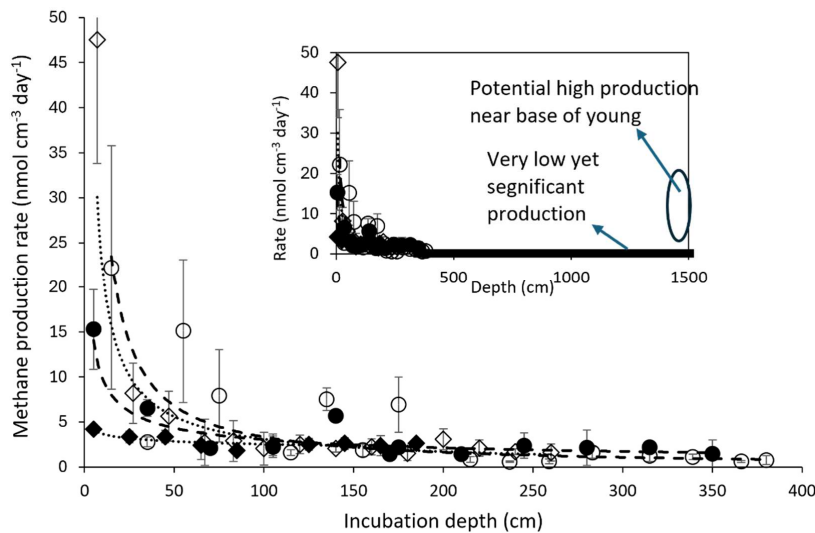
Figure 54: Methane production rates as measured in the different cores (symbols) and power law extrapolation (curves, equations in Table S5) down to 4 meters and 15 meters (upper right side). A constant low rates of less than 1 nmol cm -3 day -1 below 3 meters down to 15 meters is also marked in the upper right side, as well as the potential role of high production of methane near of the base of the young talik.
