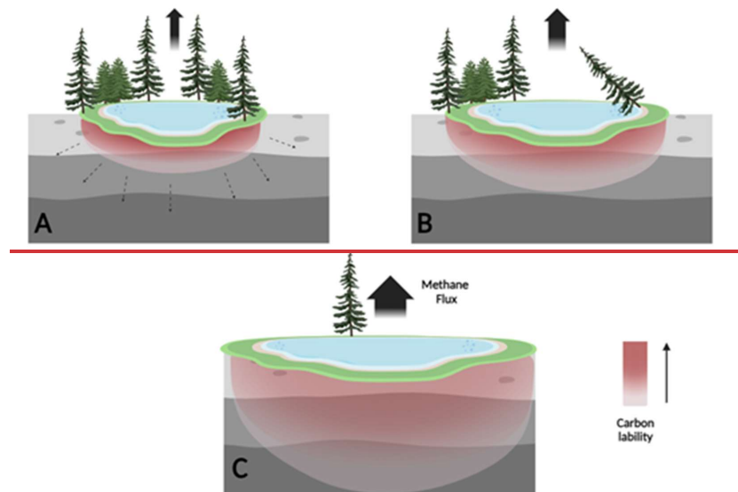
Figure 9: Laboratory incubations support the conceptual and numerical models of decreasing carbon lability leading to lower methane production as yedoma thermokarst lakes mature. The gray sediment denotes yedoma permafrost soil. Red scale color denotes organic-matter lability with talik expansion into in-situ thawed yedoma (taberites). (A) Young active lake: Labile carbon results in high methane production rates with methane production in taberites proportional to the talik thickness. (B) Expanding
