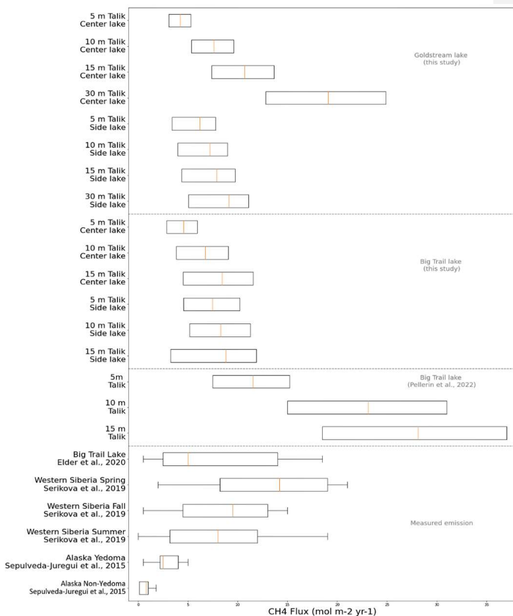
Figure 76: Total talik methane production fluxes from sediments to water column in BTL and GSL ( \text{mol m}^{-2} \text{year}^{-1} ), obtained by integrating the methane production rates over the potential range of thawed talik depths in the sediments (from surface to the marked depth) using a power law extrapolation. The middle of the box corresponds to the mean estimate and the uncertainty is the length of the boxes.
