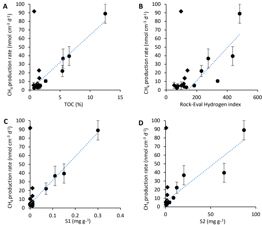
Figure 87: Methane production rates (including its uncertainty) as measured in the top upper 100 cm from both center and edge cores, and their correlation compared with TOC content (aA), hydrogen index (bB, R 2 =0.67) and the most labile organic matter compounds: S1, S2 (cC, dD), as measured on Rock-Eval. A positive relationship (R 2 0.67- to 0.98) is evident in the upper 100 cm for BTL (circles) but not for GSL (diamonds).
