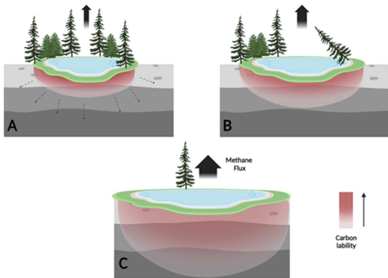
Figure 98: Laboratory incubations support the conceptual and numerical models of decreasing carbon lability leading to lower methane production as Yedoma thermokarst lakes mature. The gray sediment denotes Yedoma permafrost soil. Red scale color denotes organic matter lability with talik expansion into in-situ thawed Yedoma (taberites). (A) Young active lake: Labile carbon results in high methane production rates with methane production in taberites proportional to the talik thickness. (B) Expanding lake: Over decades new organic matter from surrounding soils and plants is added to surface lake sediments and to freshly thawed taberites at the base of the talik, while the availability of labile organic matter attenuates in formerly thawed taberites. (C) Mature lake: Over centuries the talik deepens (into bedrock) beyond the depth of taberites, while taberite organic carbon becomes refractory. Methane emissions may still be significant, depending on exogenous (non-taberite) inputs of organic matter. At later stages (as suggested by Walter Anthony et al. , 2014), the organic matter becomes no longer
