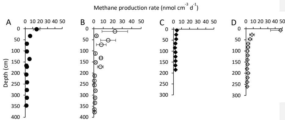
Figure 3: Methane production rates (nmol CH 4 cm -3 day -1 ) from incubation experiments of BTL sediments: Center (A) and Edge (B) cores. A steep decrease in rates with depth is observed in both the edge and center sites. Depth to permafrost beneath Big Trail Lake is thought to be 10 to 15 meters (Walter Anthony et al., 2020). Methane production rates (nmol CH 4 cm -3 day -1 ) in GSL from incubation experiments of Center (C) and Edge (D) cores. A noticeable decrease in rates with depth is observed at both center and edge of the lake. The talik depth in GSL is estimated in the center to be between 15 to 40 m (see below).
