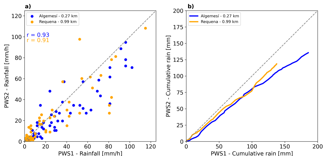
Figure 4. a) Scatter plot of 5-min rainfall between two pairs of PWSs (in Requena and Algemesi, indicated with B and E in Fig. 1c), with an inter-gauge distance of less than 1 km. The correlation coefficient ( r ) quantifies the relation between the stations. b) Cumulative rainfall between two pairs. Only intervals where both stations contain measurements are included. Legend indicates in which town the PWSs were located and the inter-gauge distance.
