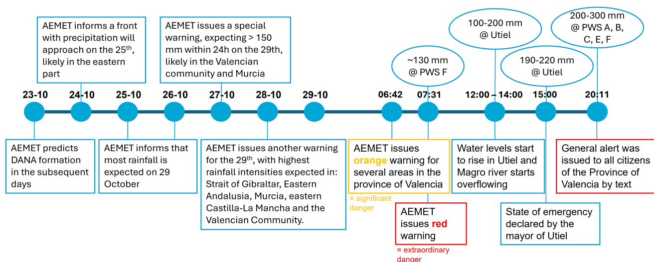
Figure 9. A posteriori timeline reconstruction (hours in local time) of the warnings and relevant processes preceding and during the 29 October 2024 Valencia floods, based on Maldita.es (2024), Bubola (2024) and AEMET (2024b, c, d, e). Rainfall measured by PWSs corresponds to the PWSs indicated in Figs. 1c and 5.
