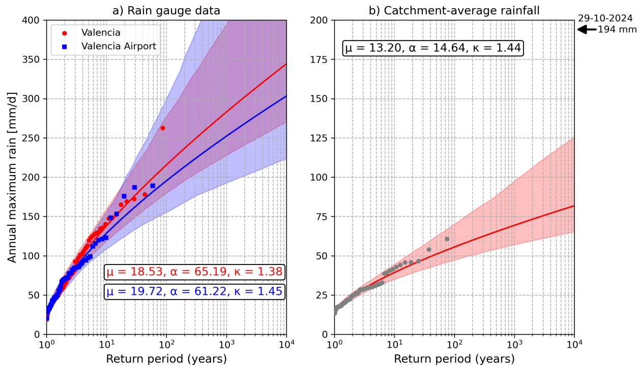
Figure 7. Return periods of annual daily maximum rainfall modelled using a GEV distribution, with \mu the location, \alpha the scale and \kappa the shape parameter. a) Estimated return periods for two rain gauges in the municipality of Valencia based on 87 and 58 years of data for Valencia and Valencia airport, respectively. b) Estimated return period of catchment-average daily rainfall for catchment ID2 in Fig. 1b based on 74 years of data. The arrow on the right indicates the estimated catchment-average rainfall on 29 October 2024 using AEMET rain gauge data. The red and blue shaded area indicates the 95% confidence interval derived from bootstrapping by sampling with replacement.
