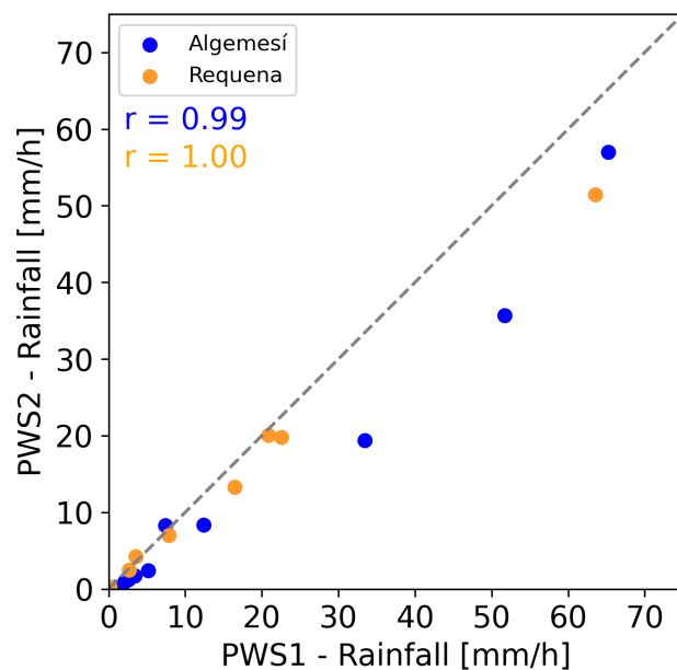
Figure A1. a) Scatter plot of hourly rainfall between two pairs of PWSs (in Requena and Algemés, indicated with B and E in Fig. 1c), with an inter-gauge distance of less than 1 km. The correlation coefficient ( r ) quantifies the relation between the stations.
