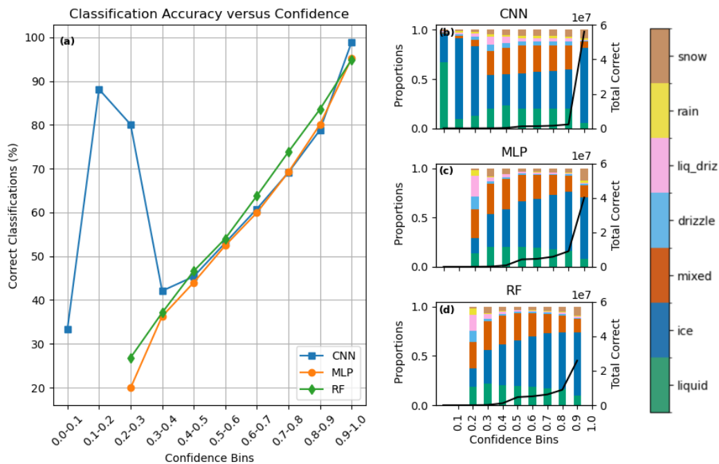
Figure S2. Distribution of accurate classifications with confidence score for test data from NSA in 2021. (a) percent of correct classifications with respect to confidence score binned by 10% intervals, (b-d) proportion of correctly classified pixels per confidence score bin, black line shows how many pixels in each bin.
