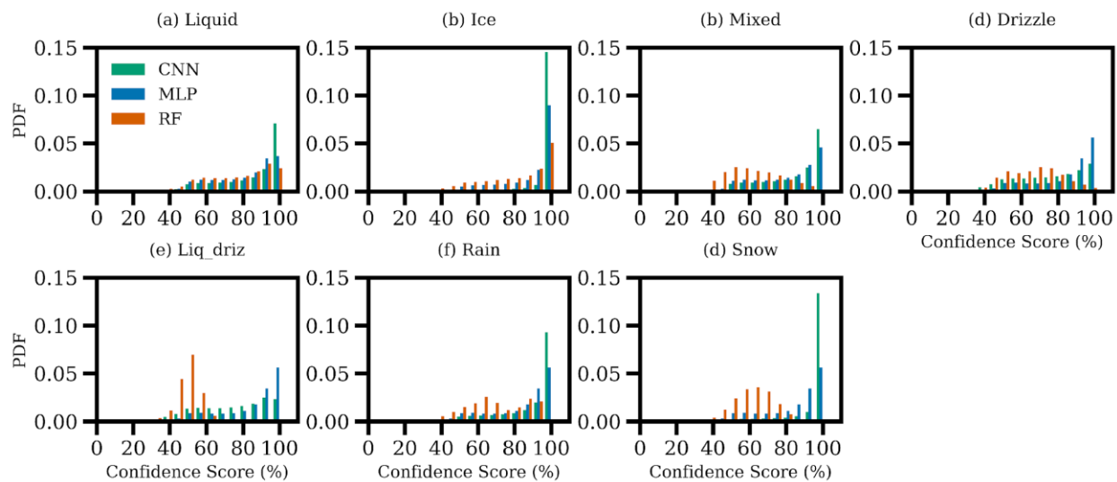
Figure S5. Probability Density Functions (PDFs) of confidence scores for thermodynamic cloud phase predictions from the three ML models using approximately 4 months of data in 2020 at the ANX site.
