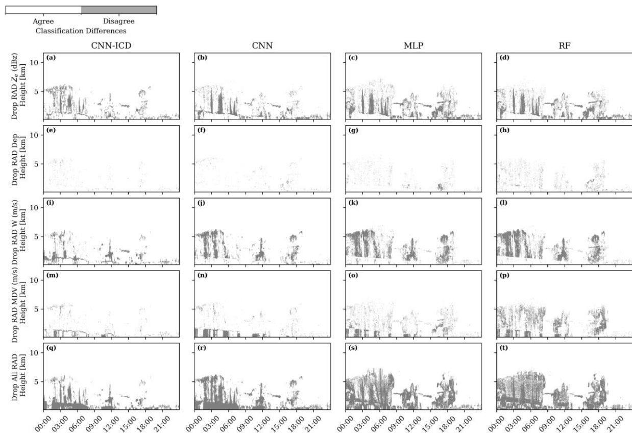
Figure S8. Differences in thermodynamic cloud phase classifications between model predictions with and without the corresponding dropout variable data for the four ML models on August 15, 2021, at the NSA site. (a-d) dropping out Radar Z_e ; (e-h) dropping out Radar Dep; (i-l) dropping out radar W; (m-p) dropping out radar MDV; (q-t) dropping out all Radar variables.
