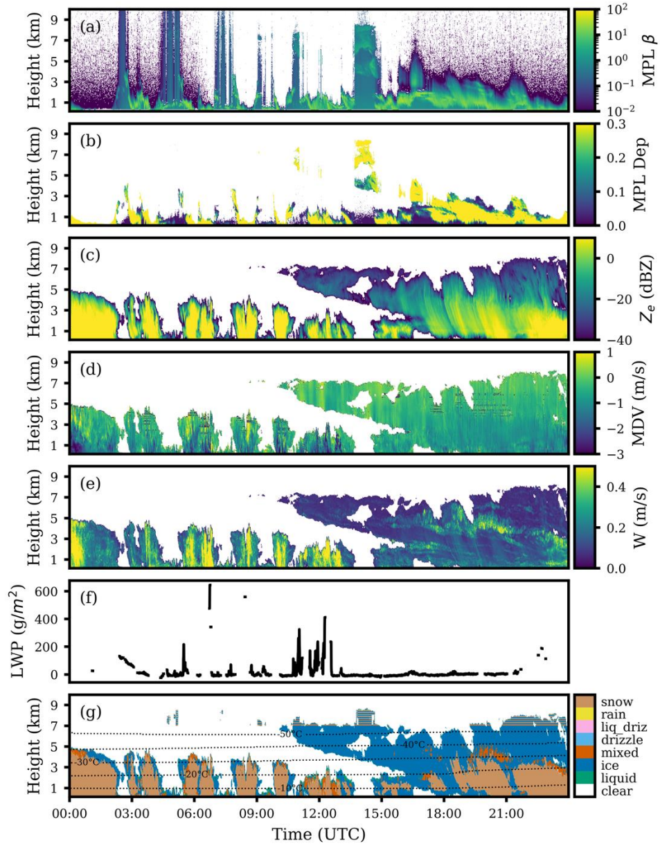
Figure S4. Multi-sensor remote sensing measurements of clouds and the thermodynamic cloud phase classification from the THERMOCLDPHASE VAP on February 25, 2020, at the ARM ANX site. Panels from top to bottom are: a) MPL attenuated backscatter (MPL \beta ); b) MPL linear depolarization ratio (MPL LDR); c) Ka-band ARM zenith radar (KAZR) radar equivalent reflectivity factor ( Z_e ); d) KAZR mean Doppler velocity (MDV); e) KAZR Doppler spectral width ( W ), f) liquid water path (LWP) from the MWRRET VAP; and g) the thermodynamic cloud phase classification from the THERMOCLDPHASE VAP. Unknown refers to pixels the THERMOCLDPHASE algorithm was unable to resolve. The dashed lines in g) are isothermal lines based on the ARM Interpolated Sonde (INTERPSONDE) VAP.
