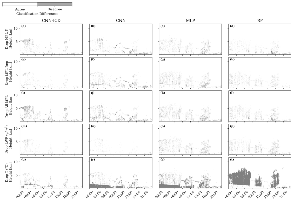
Figure S9. Similar to Figure S7, but for dropping out different variable data. (a-d) dropping out MPL Beta; (e-h) dropping our MPL Dep; (i-l) dropping out all MPL variables; (m-p) dropping out LWP; (q-t) dropping out T.
