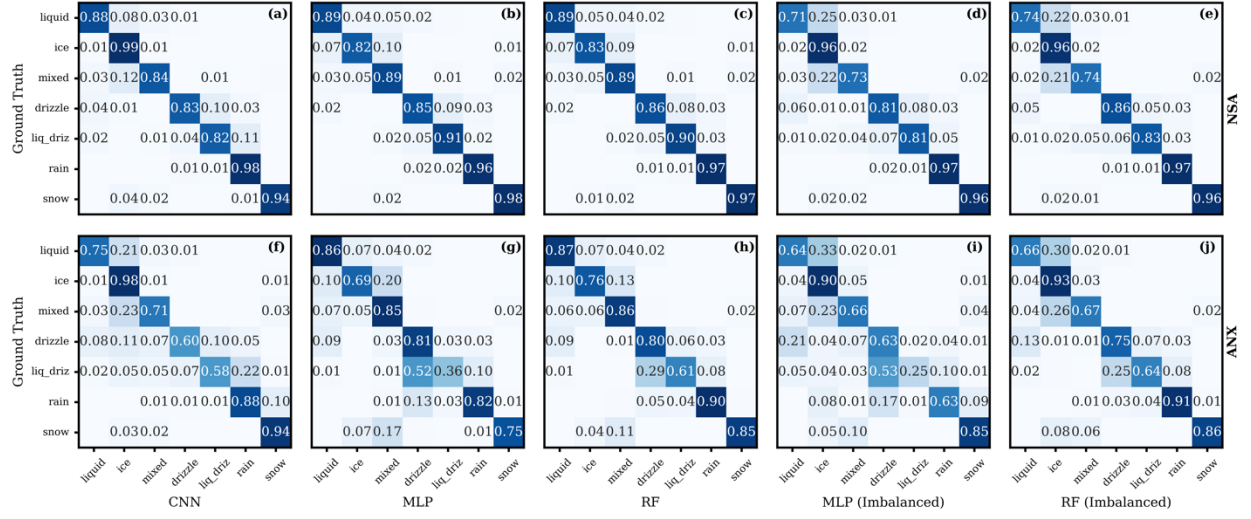
Figure S3. Confusion matrices computed on the 12 months data in 2021 at the NSA site for (a) the CNN U-net model, (b) the MLP model, (c) the RF model, (d-e) and the imbalanced MLP and RF models closest resembling the class fractions present in the CNN training data. Confusion matrices computed on the 4 months data in 2020 at the ANX site for (f) the CNN U-net model, (g) the MLP model, (h) the RF model, (i) the imbalanced MLP model, and (j) the imbalanced RF model. The values are normalized by row, with the main diagonal showing true positive predictions. Within a given row, values off the main diagonal represent false negatives.
