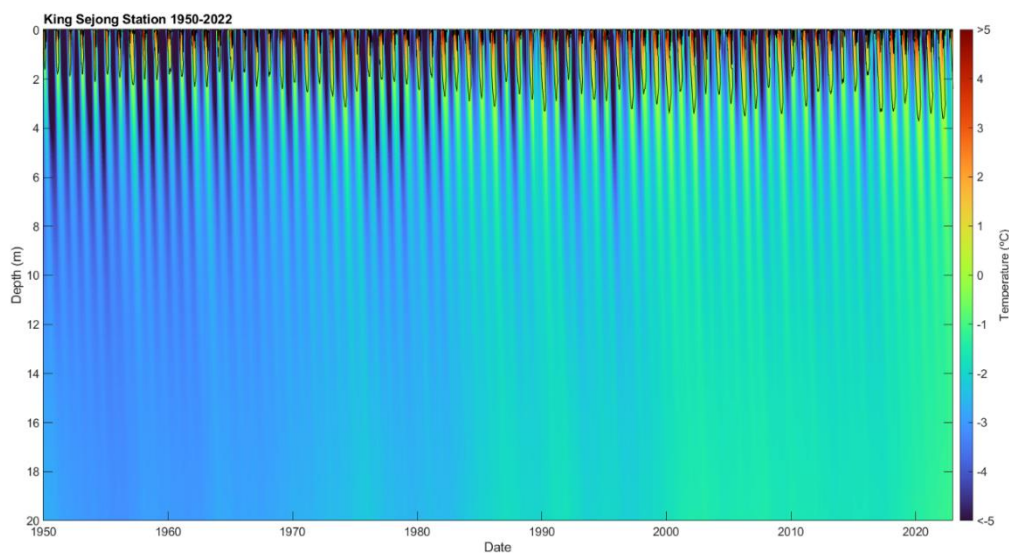
315 Figure 11: Ground temperatures simulated for the KSS borehole between January 1950 and December 2022.
