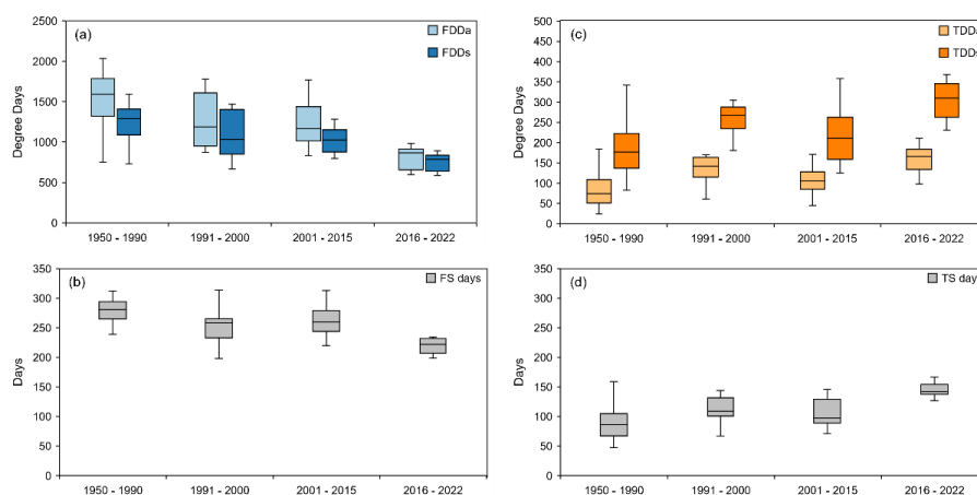
Figure 13: Characterization of the Freezing and Thawing seasons for the four periods from 1950 to 2022: a) Freezing Degree Days of the air (FDDa) and ground surface (FDDs), b) Duration of the Freezing Season (FS) in days, c) Thawing Degree Days of the air (TDDa) and ground surface (TDDs) and d) Duration of the Thawing Season (TS) in days.
