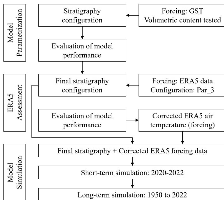
Figure 3: Workflow for the application of the CryoGrid Community Model at 1D for the KSS permafrost observatory.
