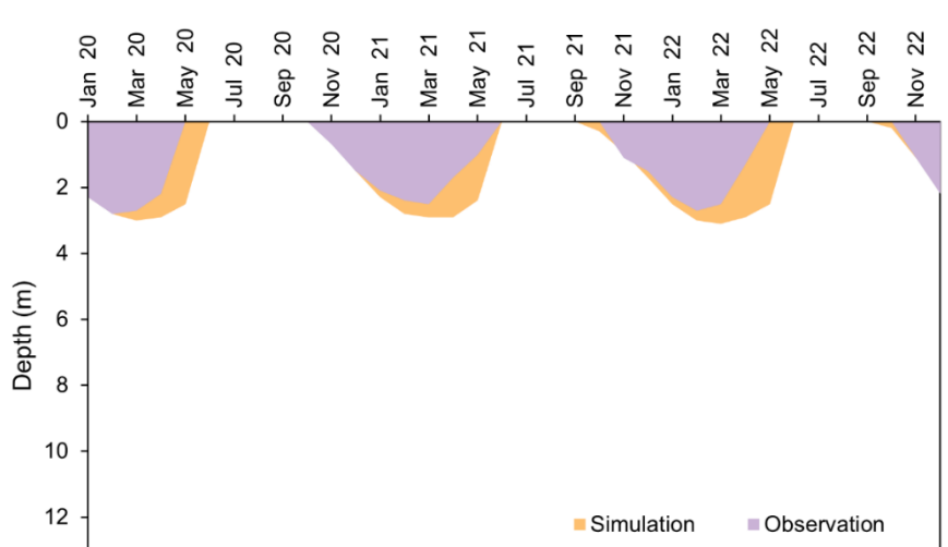
Figure 9: Thaw depth at the King Sejong Station borehole between January 2020 and December 2022. Simulated and observed results.
