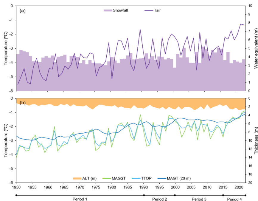
Figure 12: Long-term simulation of ground temperature (January 1950 to December 2022): a) ERA5 variables snowfall (snow factor 0.3) and air temperature; b) Mean annual ground temperatures and active layer depth calculated from the KSS borehole simulations.
