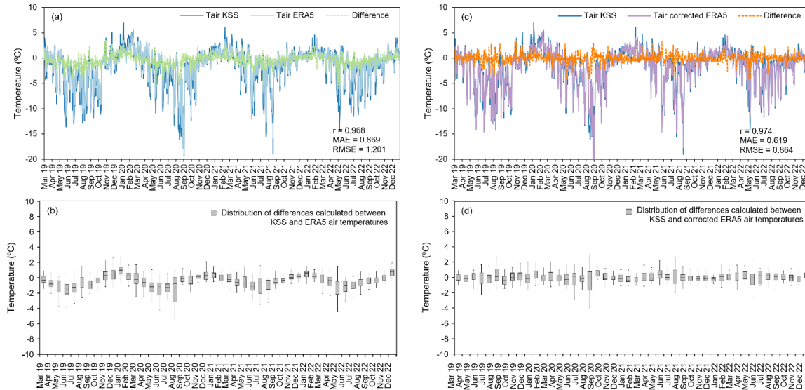
Figure 7: Air temperature recorded on the King Sejong Station Observatory, air temperature obtained from the ERA5 reanalysis product and calculated difference for the period between March 2019 and December 2022: a) KSS air temperature, ERA5 2m temperature and calculated difference; b) distribution of air temperature differences between KSS air temperature and ERA5 2m temperature; c) KSS air temperature, corrected ERA5 2m temperature and calculated difference; d) distribution of air temperature differences between KSS air temperature and corrected ERA5 2m temperature.
