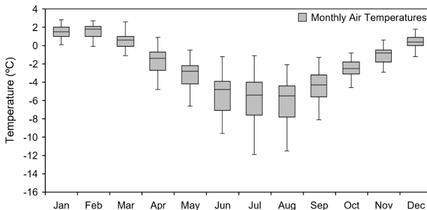
Figure 2: Monthly Air Temperatures in Bellingshausen Station from 1969 to 2022 (MET-READER).
