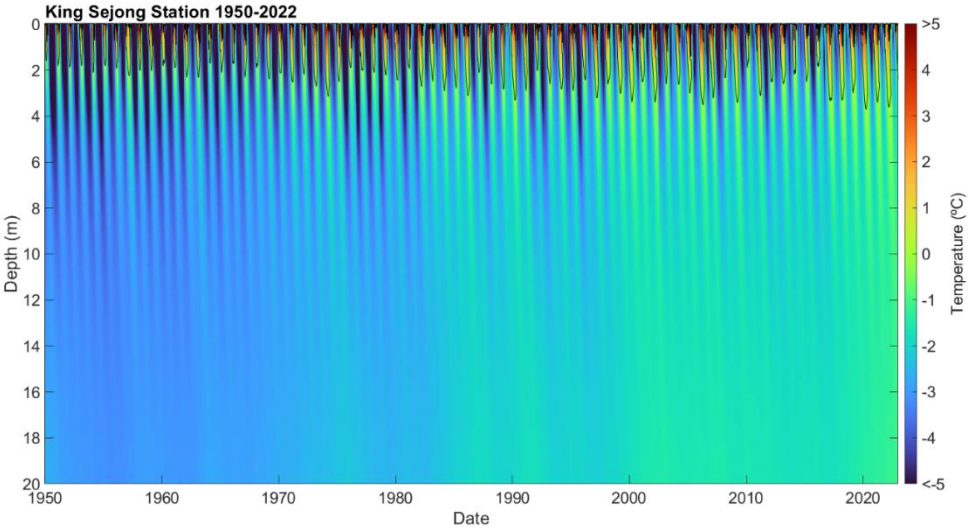
340 Figure 11: Ground temperatures simulated for the KSS borehole between January 1950 and December 2022.
