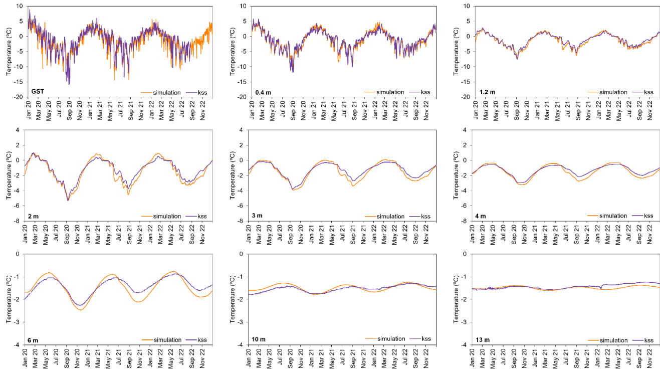
Figure 8: Simulated vs observed ground temperatures for the KSS borehole between January 2020 and December 2022.
