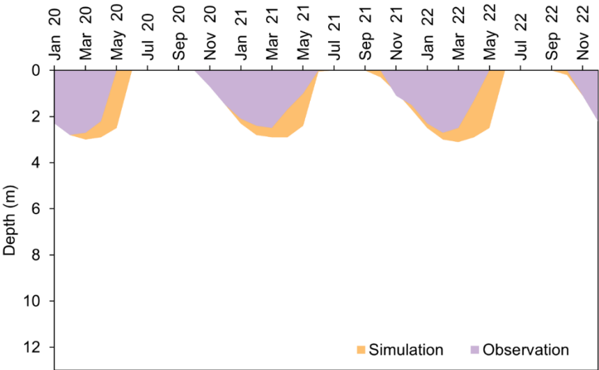
305 Figure 9: Thaw depth at the King Sejong Station borehole between January 2020 and December 2022. Simulated and observed results.
