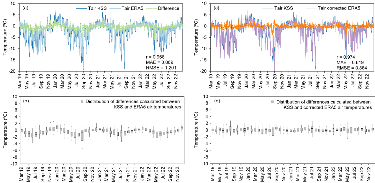
260 Figure 7: Air temperature recorded on the King Sejong Station Observatory, air temperature obtained from the ERA5 reanalysis product and calculated difference for the period between March 2019 and December 2022: a) KSS air temperature, ERA5 2m temperature and calculated difference; b) distribution of air temperature differences between KSS air temperature and ERA5 2m temperature; c) KSS air temperature, corrected ERA5 2m temperature and calculated difference; d) distribution of air temperature differences between KSS air temperature and corrected ERA5 2m temperature.
