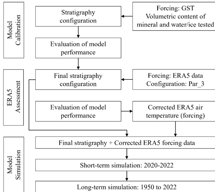
100 Figure 3: Workflow for the application of the CryoGrid Community Model at 1D for the KSS permafrost observatory.
