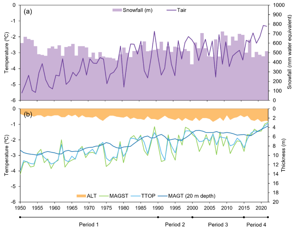
Figure 12: Long-term simulation of ground temperature (January 1950 to December 2022): a) ERA5 variables snowfall (mm water equivalent) and air temperature (°C); b) Mean annual ground temperatures and active layer depth calculated from the KSS borehole simulations.
