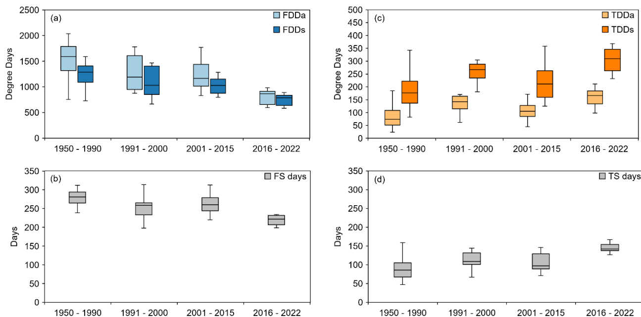
380 Figure 13: Characterization of the Freezing and Thawing seasons for the four periods from 1950 to 2022: a) Freezing Degree Days of the air (FDDa) and ground surface (FDDs), b) Duration of the Freezing Season (FS) in days, c) Thawing Degree Days of the air (TDDa) and ground surface (TDDs) and d) Duration of the Thawing Season (TS) in days.
