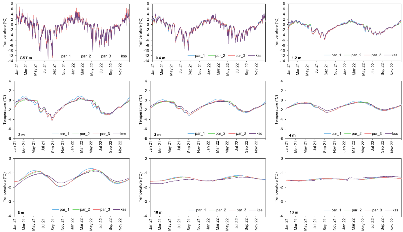
250 Figure 6: Measured and estimated mean daily ground temperatures in the King Sejong Station borehole from January 2021 to December 2022.
