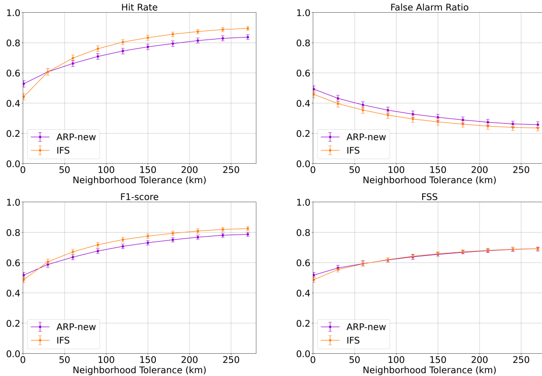
Figure 8. HR, FAR, F_1 -score and FSS score on ISSR events ( RH_{ice} > 100 %) forecasts depending on increasing neighborhood spatial tolerance, for ARP-new (purple) and for IFS (orange) with 95 % confidence intervals. Neighborhood distances range from the nearest to 270 km, with 30 km increments. Verification dataset from the 1st July 2022 to the 30th June 2023 within the aerial boundary of 80^\circ W– 40^\circ E and 30^\circ – 75^\circ N, covering North Atlantic and Europe.
