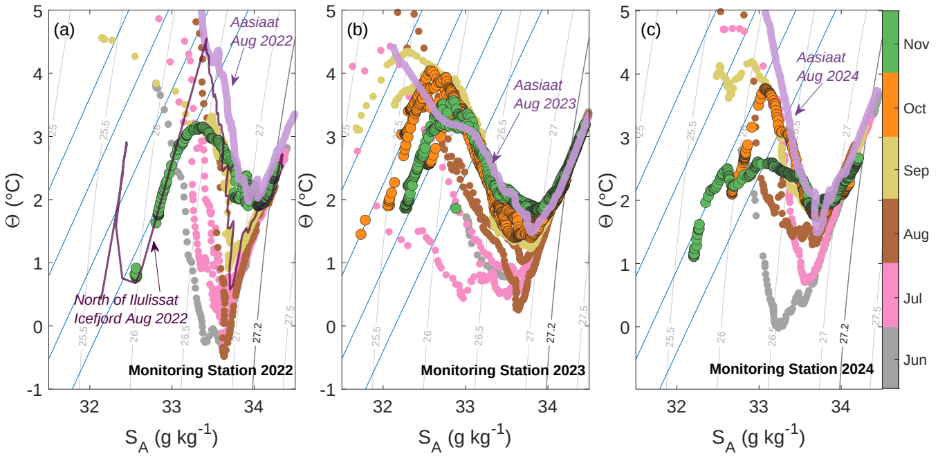
Figure 7. Temperature - Salinity ( \Theta - S_A ) diagrams for the Monitoring Station for (a) 2022, (b) 2023, and (c) 2024, covering June–November. Circle markers are observations coloured by month; October–November are shown with a black outline. The thick lilac line in panels (a–c) shows \Theta - S_A properties at the station near Aasiaat during August of the same year (previously shown in Fig.4b, d, f); the thin purple line in (a) is the same, but for the station north of Ilulissat Icefjord. Isopycnals are shown in grey, with the thick contour delineating West Greenland Irminger Water (WGIW) and Polar Water (PW). Submarine meltwater ( \Theta = -90^\circ\text{C} , S_A = 0 \text{ g kg}^{-1} ) mixing lines are shown in blue
