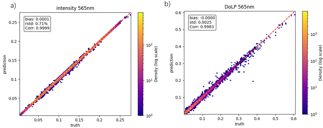
Figure 2. Scatter plot of intensity and DoLP at 565 nm from NN forward model. The bias of both intensity and DoLP is close to zero. The rstd of intensity is 0.7% and the std of DoLP is 0.0025. Both of them are below the instrument measurement noise, which suggests the NN forward model is good enough to replace the full physical model (RemoTAP) in estimating goodness-of-fit.
