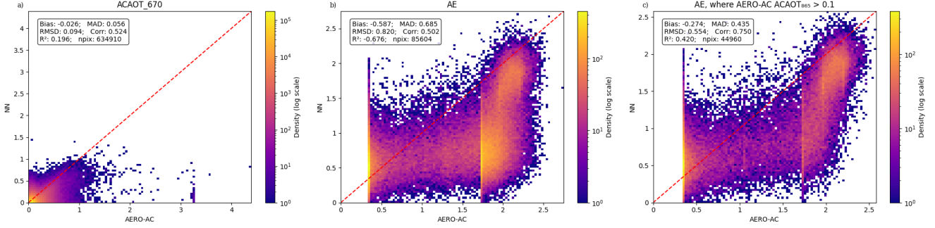
Figure 7. Comparison of ACAOT_{670} (panel a) and AE (panel b) between PARASOL-NN and AERO-AC. AE from both PARASOL-NN and AERO-AC is filtered with ACAOT_{550} > 0.2 ( ACAOT_{550} from AERO-AC is calculated with unfiltered AE and ACAOT_{670} ). Panel c shows the AE comparison with an additional filter: ACAOT_{865} > 0.1 (from AERO-AC). Note the AE given by PARASOL-NN is between 440 nm and 670 nm while that by AERO-AC is between 670 nm and 865 nm.
