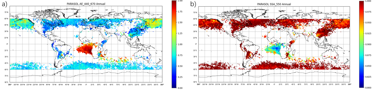
Figure 9. Annual AE_{440-670} (panel a) and SSA_{550} (panel b) average on each 1^\circ \times 1^\circ grid in 2008. The AE and SSA are calculated where ACAOT_{550} > 0.2 . The ACA events in the western coast of mid-Africa have a distinctive feature than others, that the aerosols have a large AE (smaller particles) and a smaller SSA (more absorbing).
