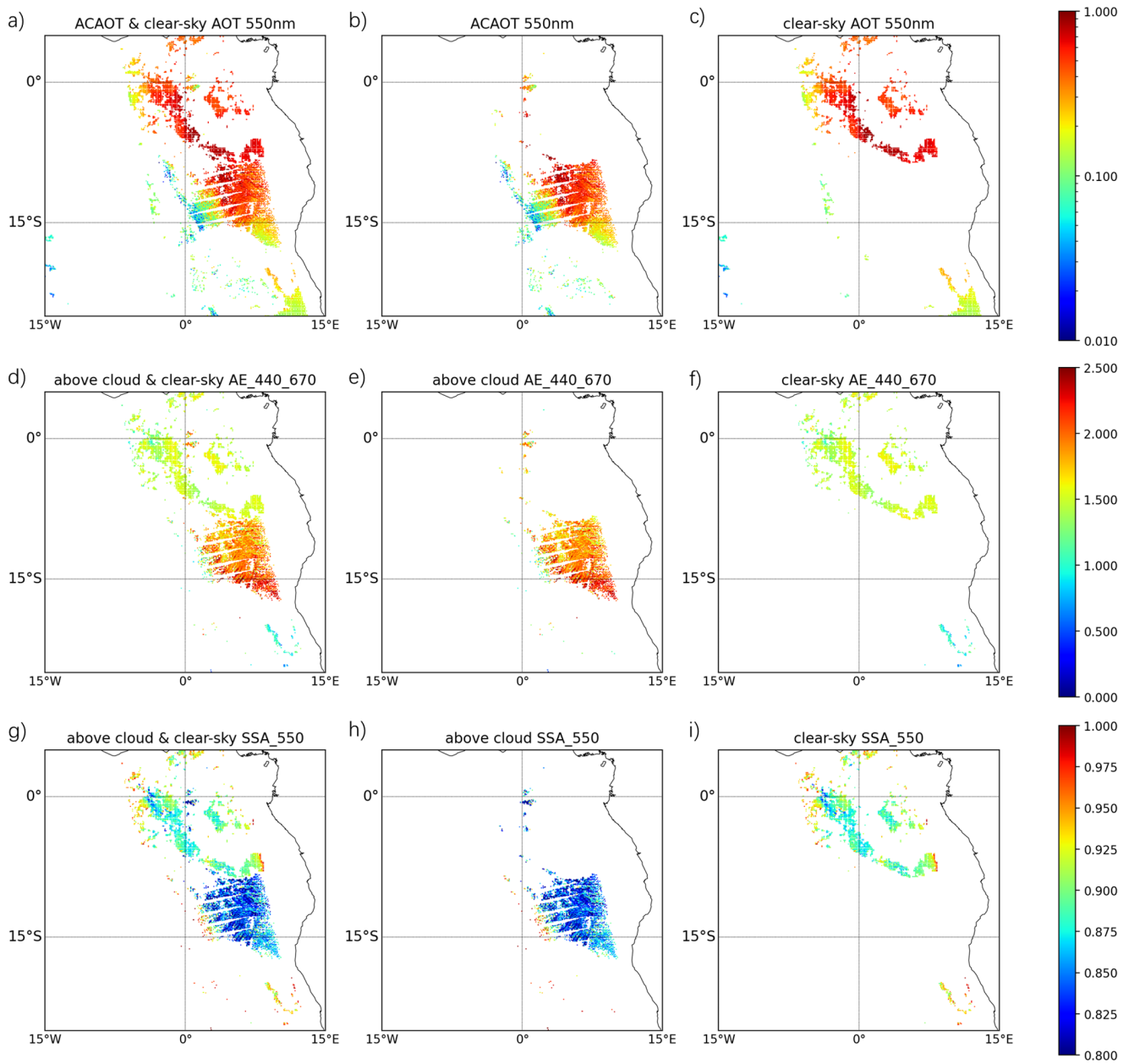
Figure 5. ACAOT 550 and clear-sky AOT 550 (a, b, c), AE 440–670 (d, e, f) and SSA 550 (g, h, i) in mid-Africa, 4 Aug 2008. The left column (a, d, g) shows both the ACA and the clear-sky aerosol retrievals. The middle column (b, e, h) is the ACA retrievals and the right column (c, f, i) is the clear-sky aerosol retrievals. In this case, the ACA (mostly smoke) has a larger AE 440–670 and smaller SSA 550 than the adjacent clear-sky aerosols (smoke and sea salt).
