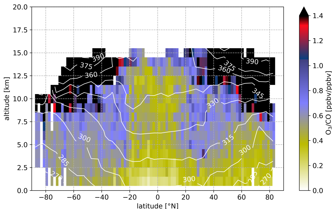
Figure 3. Same as Figure 2, for the O_3 – CO ratio.
