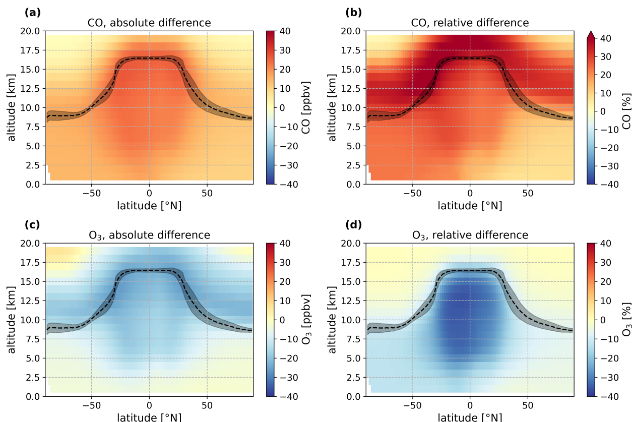
Figure 7. Relative and absolute differences of CO and O 3 caused by excluding LNO x emissions in the global 3D model EMAC (without LNO x ), shown on annual averaged zonal distributions. In a) and c) the absolute differences (Eq. 2) of the gas concentration are shown and in b) and d) the relative difference (Eq. 3) in percentage normalized to the background concentration in the particular area are displayed for CO (a, b) and O 3 (c, d). The black dashed lines and shaded area indicate the mean height of the tropopause layer and its standard deviation, respectively, by taking the zonal and annual average.
