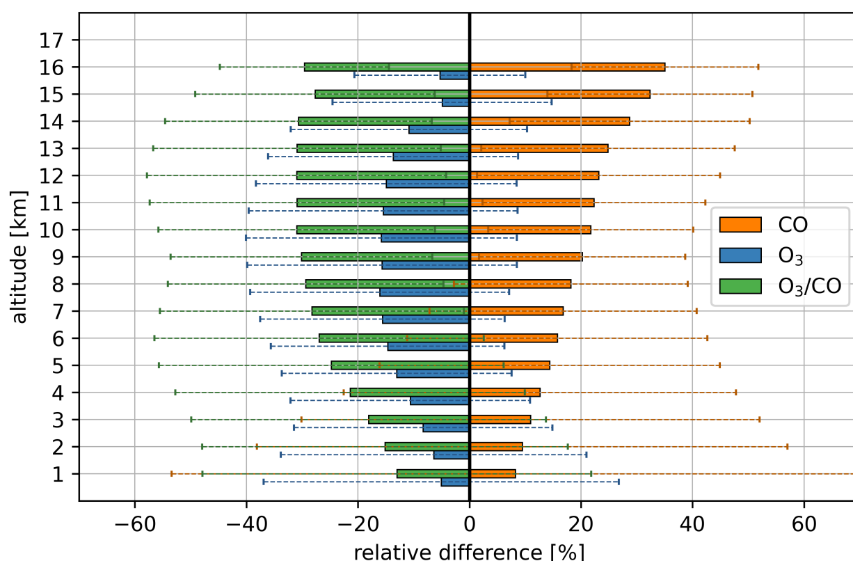
Figure 10. The mean relative differences in O_3 (blue bars), CO (orange bars), and their ratio (green bars) averaged over all longitudes, the northern subtropics ranging from 23.3^\circ N – 40^\circ N , and for each kilometer, with exclusion of stratospheric values selected by O_3 values higher than 100 ppbv. This mean includes an average over all months. The error bars show the standard deviation and represent the meridional variability of the relative differences. Calculated using Eq. 3.
