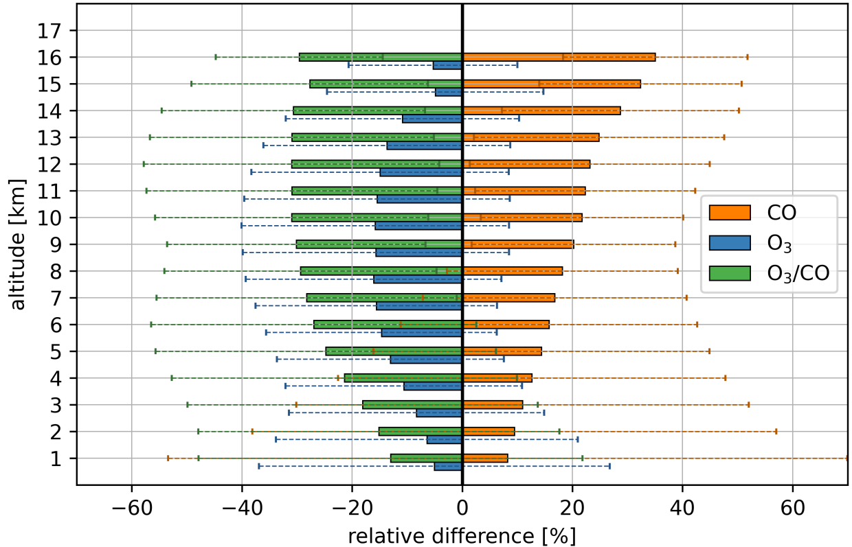
Figure 10. The mean relative differences in \text{O}_3 (blue bars), \text{CO} (orange bars), and their ratio (green bars) averaged over all longitudes, the northern subtropics ranging from 23.3^\circ \text{N} - 40^\circ \text{N} , and for each kilometer, with exclusion of stratospheric values selected by \text{O}_3 values higher than 100 ppbv. This mean includes an average over all months. The error bars show the standard deviation and represent the meridional variability of the relative differences. Calculated using Eq. 3.
