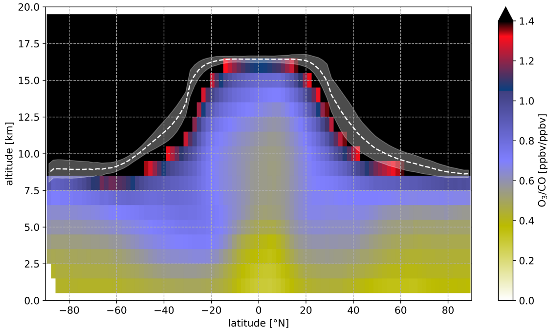
Figure 5. The median annual zonal distribution of the \text{O}_3 - \text{CO} ratio calculated from the EMAC model data (REF). All data points are averaged over 1 km of altitude and 1.875^\circ of latitude. The scale has been adjusted to display tropospheric values. The white dashed lines indicate the tropopause layer height with its standard deviation shaded in white.
