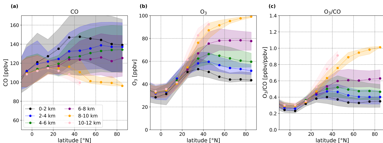
Figure 8. Same as Figure 6, for the model simulation without \text{LNO}_x .
