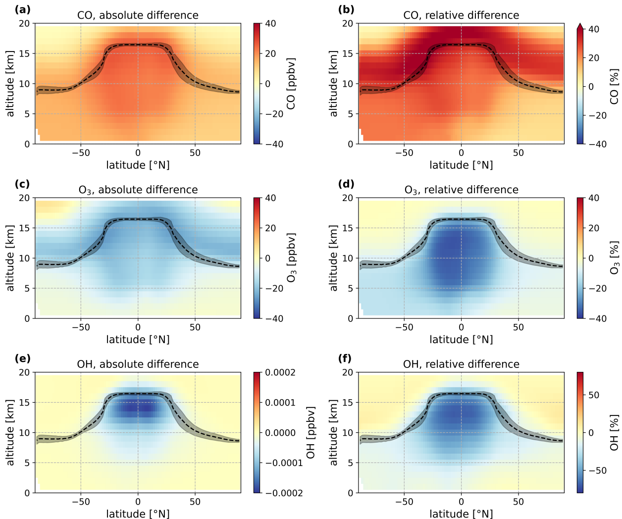
Figure 7. Relative and absolute differences of CO (a, b), O 3 (c, d), and OH (e, f) caused by excluding LNO x emissions in the global 3D model EMAC, shown on annual averaged zonal mean distributions. On the left side (a, c, e) the absolute differences (Eq. 2) of the gas concentration are shown and on the right side (b, d, f) the relative differences (Eq. 3) in percentages normalized to the background concentrations. Note the scales for OH differ from CO and O 3 . The black dashed lines and shaded area indicate the mean height of the tropopause layer and its standard deviation, respectively, by taking the zonal and annual average.
