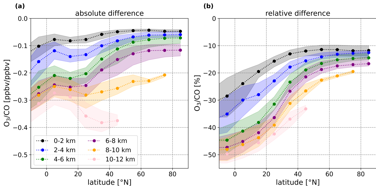
Figure 9. Same as Figure 6, but for the absolute differences (a) and relative differences (b) of the O_3 - CO ratio between the base run and the sensitivity run without LNO_x .
