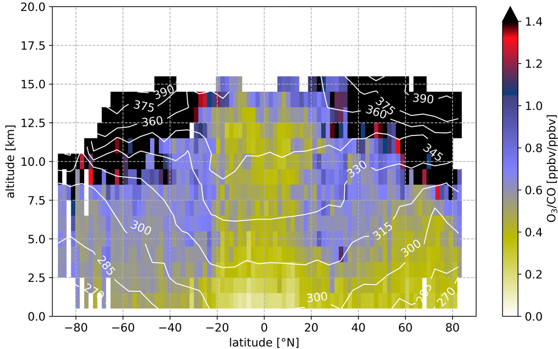
Figure 3. Same as Figure 2, for the \text{O}_3 – CO ratio, but without hatching and \Theta shown as white lines.
