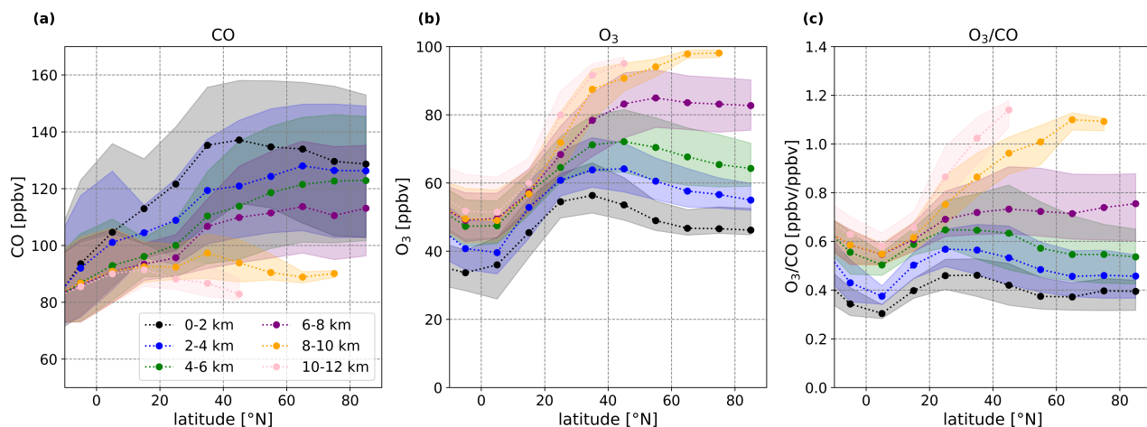
Figure 6. Northern hemispheric zonal gradients of CO (a), O_3 (b), and the O_3 - CO ratio (c) from the EMAC model data (REF), averaged over 10^\circ of latitude and 2 km of altitude. Dots represent medians and shaded areas denote the 25 th and 75 th percentiles. Before the calculations, only tropospheric data was selected based on the chemical definition of the tropopause by Prather et al. (2011) at 100 ppbv of O_3 .
