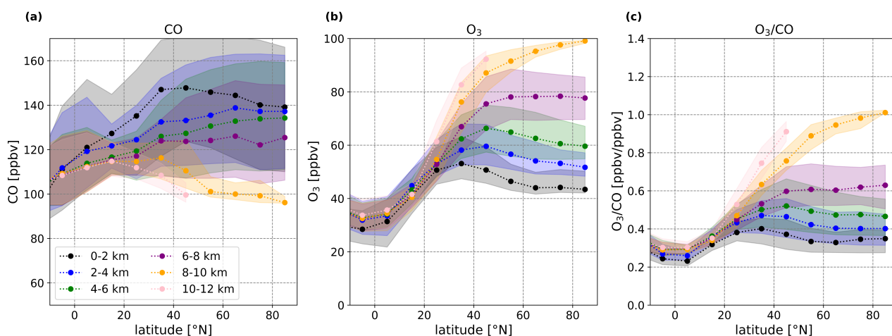
Figure 8. Same as Figure 6, for the model simulation without LNO x .
