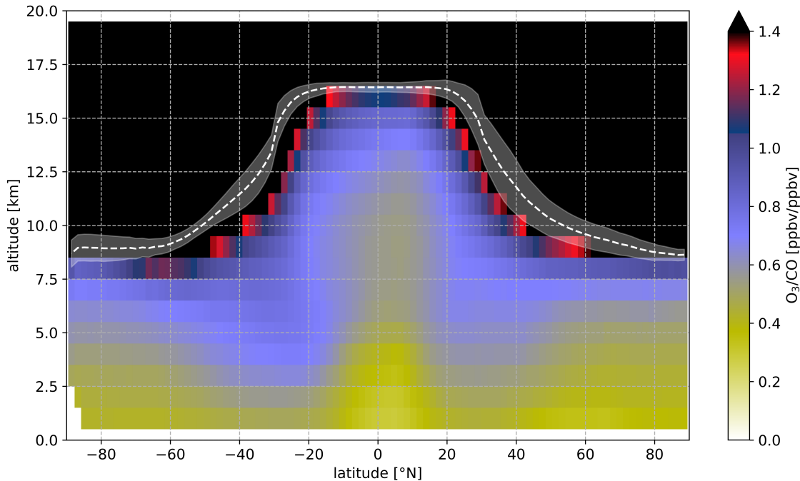
Figure 5. The median annual zonal distribution of the \text{O}_3 –CO ratio calculated from the EMAC model data (REF). All data points are averaged over 1 km of altitude and 1.875^\circ of latitude. The scale has been adjusted to display tropospheric values. The white dashed lines indicate the tropopause layer height with its standard deviation shaded in white.
