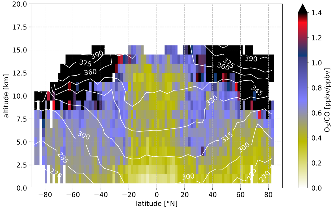
Figure 3. Same as Figure 2, for the O_3 – CO ratio, without the hatching and \Theta shown in white lines.
