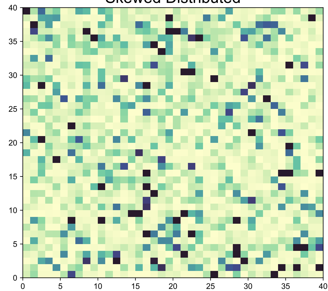
Skewed Distributed
