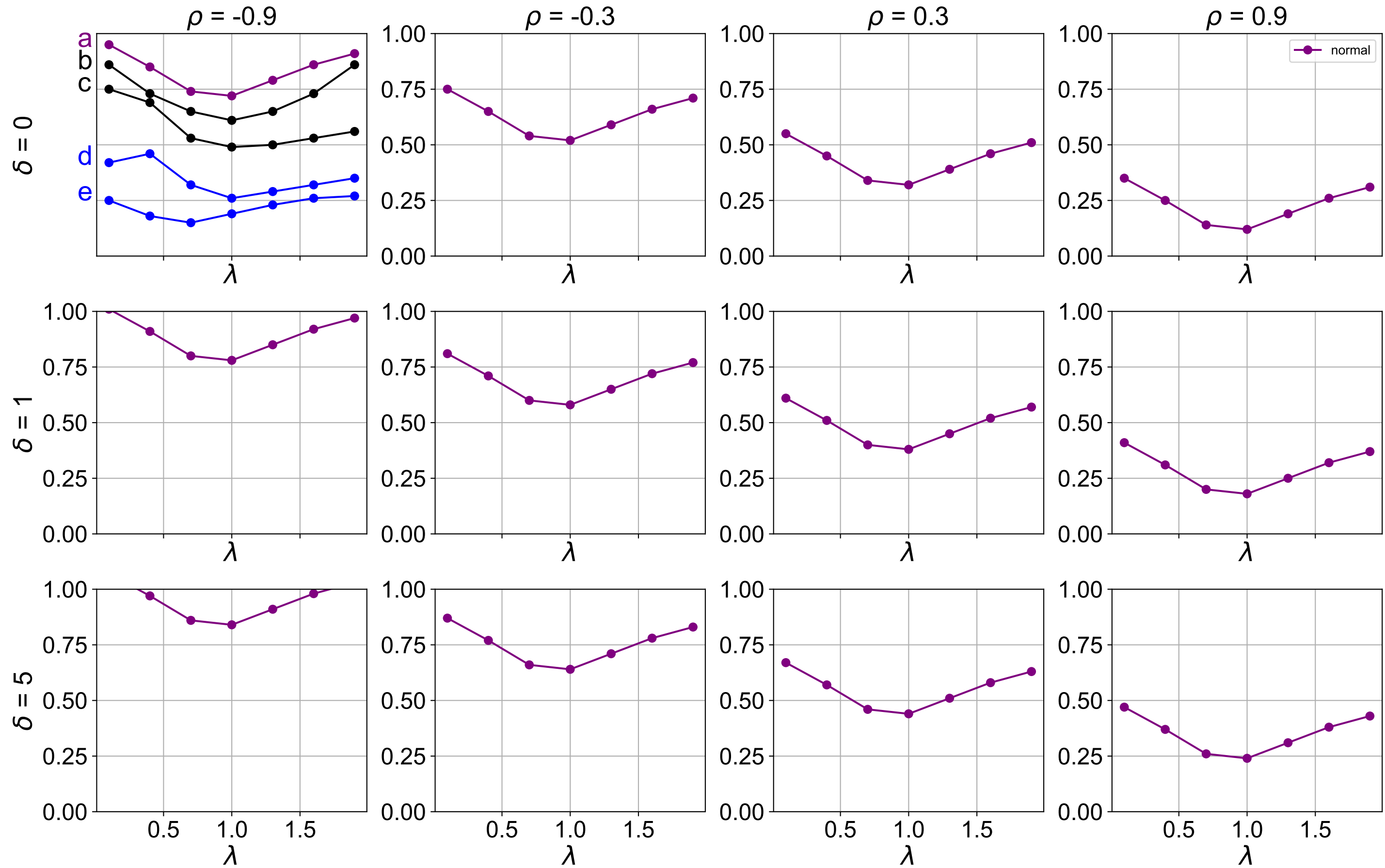
Metric Behavior
