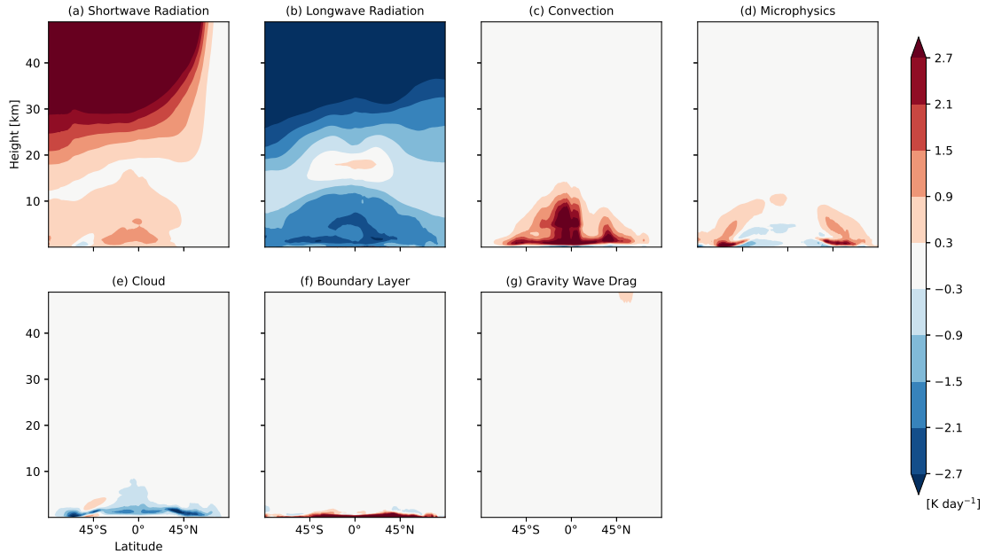
Figure 11. Latitude-height cross sections of contributions to a breakdown of the model physics temperature tendency (shown in Fig. 10(ac)) from to the individual parametrizations, (a) shortwave radiation, (b) longwave radiation, (c) convection, (d) microphysics, (e) cloud, (f) boundary layer, and (g) gravity wave drag [K day -1 ] in CNTL from initial conditions to T+120h averaged over the 90 cases.
