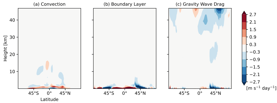
Figure 7. Latitude-height cross sections of contributions to a breakdown of the model physics zonal-wind tendency (shown in Fig. 6(ac)) from to the individual parametrizations, (a) convection, (b) boundary layer, and (c) gravity wave drag [ \text{m s}^{-1} \text{ day}^{-1} ] in CNTL from initial conditions to T+120h averaged over the 90 cases.
