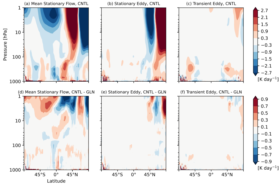
Figure 9. Latitude-height cross sections of contributions to a breakdown of the resolved processes (shown in Fig. 8 (b, e) from ) to the individual terms of the zonal-mean thermal budget equation [ \text{K day}^{-1} ] written in Eq. (3) (i.e., from left to right, (a, d) the mean stationary flow term, (b, e) the stationary eddy heat flux term, and (c, f) the transient eddy heat flux term) from initial conditions to T+120h averaged over the 90 cases (a-c) in CNTL, and (b-d-f) their differences between CNTL and GLN. Note that the colour scales in (a-c) and (b-d-f) are different.
