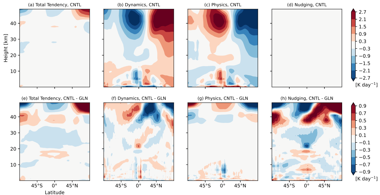
Figure 10. Latitude-height cross sections of zonal-mean (a, e) total tendency of temperature, and their breakdown into model tendencies of model (b, f) dynamics, (c, g) physics, and (d, h) nudging [ \text{K day}^{-1} ] from initial conditions to T+120h averaged over the 90 cases (aa-d) in CNTL, and (be-h) their differences between CNTL and GLN. Temperature tendency due to nudging in CNTL is completely null. Note that the colour scales in (aa-d) and (be-h) are different.
