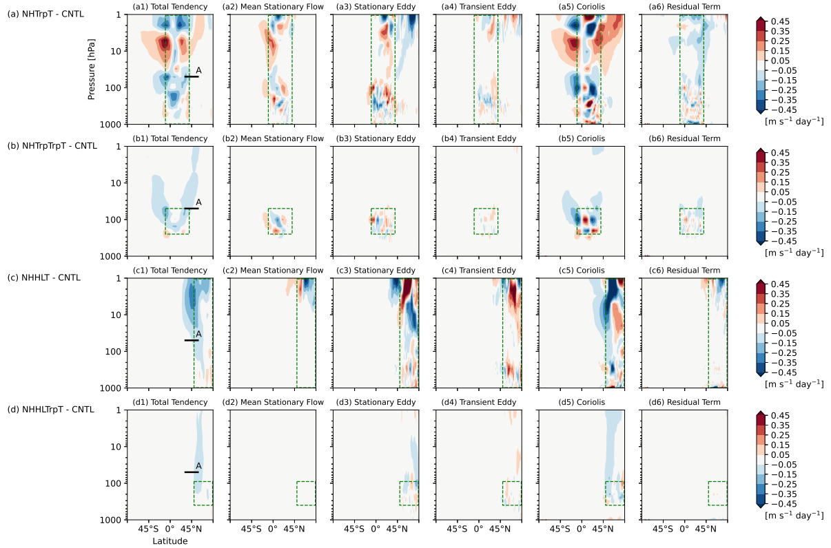
Figure 16. Latitude-height cross sections of differences in zonal-mean (a1–d1) total tendency of zonal wind, and budget contributions from the the individual terms of the zonal-mean zonal momentum budget equation (i.e., from left to right, (a2–d2) the mean stationary flow advection term, (a3–d3) the stationary eddy momentum flux term, (a4–d4) the transient eddy momentum flux term, (a5–d5) the Coriolis term, and (a6–d6) the residual term) [ \text{m s}^{-1} \text{ day}^{-1} ] written in Eq. (2) from initial conditions to T+120h averaged over the 90 cases in (a) NHTrpT minus CNTL, (b) NHTrpTrpT minus CNTL, (c) NHHLT minus CNTL, and (d) NHHLTrpT minus CNTL. Green dashed boxes indicate the temperature-nudging domain including interfacing transition zones and layers. The black horizontal line A, the same as that in Fig. 1(e), are inserted for reference. Note that the colour scale is different from that in Fig. 4.
