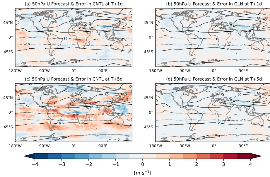
Figure 3. Spatial distributions of zonal wind errors [ \text{m s}^{-1} ] at 50 hPa at a forecast lead time of (a, b) Day 1 and Day 5 (from top to bottom, c, d) Day 5 averaged over the 90 cases from 1 Dec. 2018 to 28 Feb. 2019 in (a, c) CNTL, and (b, d) GLN. Contour indicates the forecasts, and colour indicates mean errors against the MetUM analysis.
