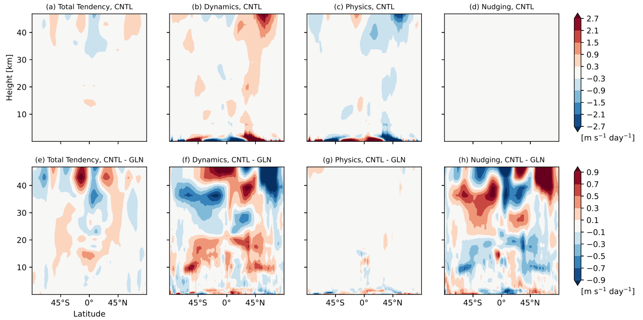
Figure 6. Latitude-height cross sections of zonal-mean (a, e) total tendency of zonal wind, and their breakdown into model tendencies of model (b, f) dynamics, (c, g) physics, and (d, h) nudging [ \text{m s}^{-1} \text{ day}^{-1} ] from initial conditions to T+120h averaged over the 90 cases (aa–d) in CNTL, and (be–h) their differences between CNTL and GLN. Zonal wind tendency due to nudging in CNTL is completely null. Note that the colour scales in (aa–d) and (be–h) are different.
