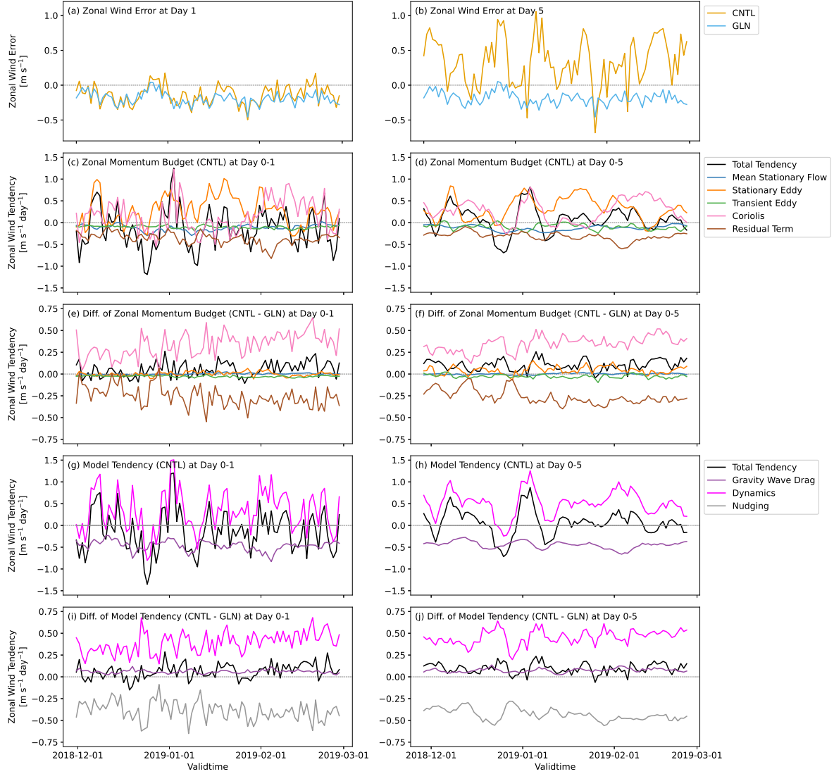
Figure 12. Timeseries area-averaged over the NH mid-latitude (30°N–60°N) at 50 hPa depicted by the line A in Fig. 1(c) of (a, b) zonal wind errors against the MetUM analyses [ \text{m s}^{-1} ], (c, d) zonal momentum budget in CNTL [ \text{m s}^{-1} \text{ day}^{-1} ], (e, f) differences in the zonal momentum budget (CNTL minus GLN) [ \text{m s}^{-1} \text{ day}^{-1} ], (g, h) individual model physics, dynamics, and nudging tendencies in CNTL [ \text{m s}^{-1} \text{ day}^{-1} ], and (i, j) differences in the individual model physics, dynamics, and nudging tendencies (CNTL minus GLN) [ \text{m s}^{-1} \text{ day}^{-1} ]. Left column shows Day 1 forecasts: (a) the errors at a T+24h forecast lead time, and (c, e, g, i) temporal changes from initial conditions to T+24h. Right column shows Day 5 forecasts: (b) the errors at a T+120h forecast lead time, and (d, f, h, j) temporal changes from initial conditions to T+120h. Note that the nudging tendency in (g, h) is completely null, and physics parametrization tendencies of the convection scheme and the boundary layer scheme are omitted in (g–j) because they are negligibly small in this case.
