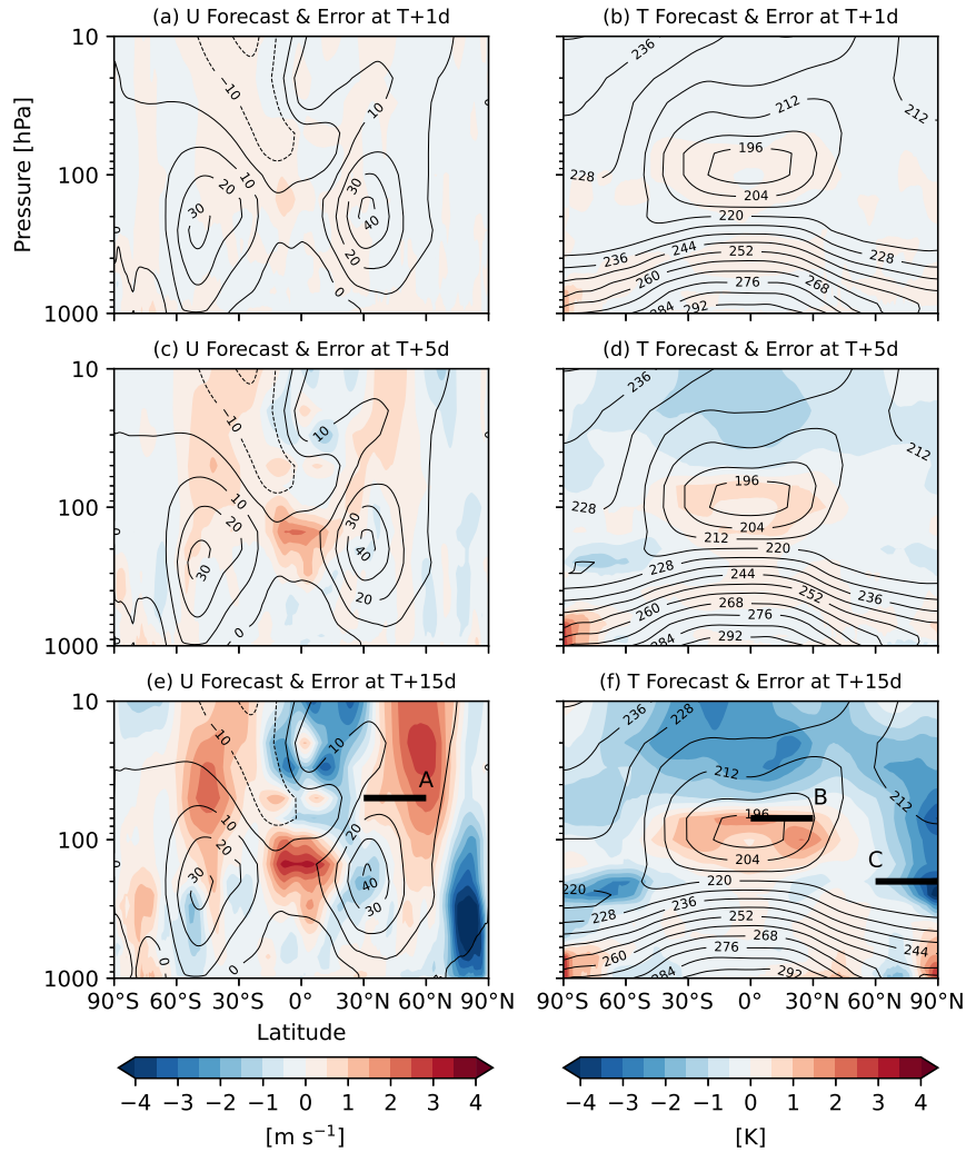
Figure 1. Zonal-mean errors of the CNTL forecast at a forecast lead time of (a, b) Day 1, (c, d) Day 5, and Day 15 (from top to bottom, e, f) Day 15 averaged over the 90 cases from 1 Dec. 2018 to 28 Feb. 2019 in (a, c, e) zonal wind velocity [ \text{m s}^{-1} ], and (b, d, f) temperature [K]. Contour indicates the forecasts, and colour indicates mean errors against the MetUM analysis. The black horizontal lines A, B, and C are inserted for later reference (Figs. 2, 12, 13, and 14; see the text in detail).
