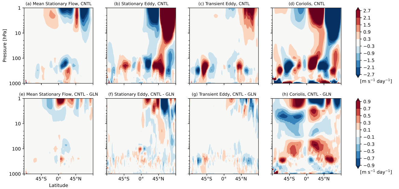
Figure 5. Latitude-height cross sections of contributions to a breakdown of the resolved processes (shown in Fig. 4(b, e) from ) to the individual terms of the zonal-mean zonal momentum budget equation [ \text{m s}^{-1} \text{ day}^{-1} ] written in Eq. (2) (i.e., from left to right, (a, e) the mean stationary flow advection term, (b, f) the stationary eddy momentum flux term, (c, g) the transient eddy momentum flux term, and (d, h) the Coriolis term) from initial conditions to T+120h averaged over the 90 cases (aa–d) in CNTL, and (be–h) their differences between CNTL and GLN. Note that the colour scales in (aa–d) and (be–h) are different.
