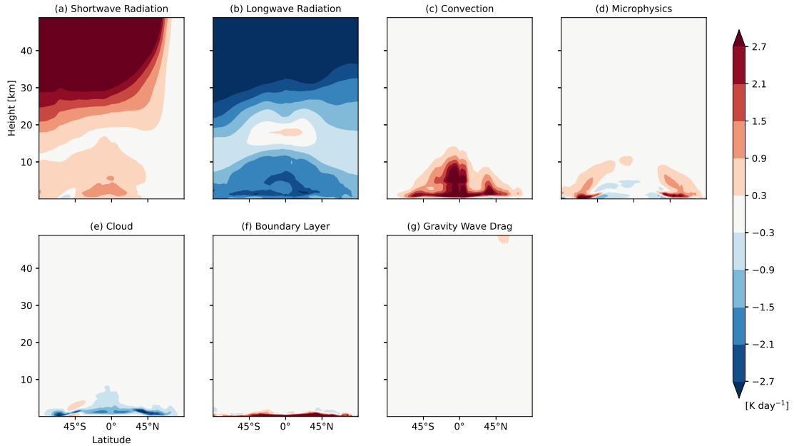
Figure 11. Latitude-height cross sections of contributions to a breakdown of the model physics temperature tendency (shown in Fig. 10( ac )) from to the individual parametrizations, (a) shortwave radiation, (b) longwave radiation, (c) convection, (d) microphysics, (e) cloud, (f) boundary layer, and (g) gravity wave drag [K day -1 ] in CNTL from initial conditions to T+120h averaged over the 90 cases.
