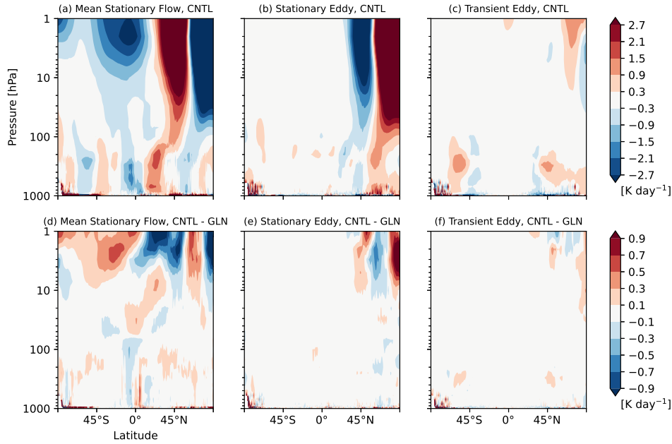
Figure 9. Latitude-height cross sections of contributions to a breakdown of the resolved processes (shown in Fig. 8(b, e) from ) to the individual terms of the zonal-mean thermal budget equation [ \text{K day}^{-1} ] written in Eq. (3) (i.e., from left to right, (a, d) the mean stationary flow term, (b, e) the stationary eddy heat flux term, and (c, f) the transient eddy heat flux term) from initial conditions to T+120h averaged over the 90 cases (a-c) in CNTL, and (d-f) their differences between CNTL and GLN. Note that the colour scales in (a-c) and (d-f) are different.
