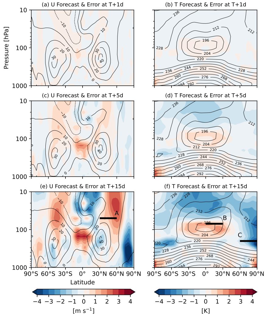
Figure 1. Zonal-mean errors of the CNTL forecast at a forecast lead time of (a, b) Day 1, (c, d) Day 5, and Day 15 (from top to bottom, e, f) Day 15 averaged over the 90 cases from 1 Dec. 2018 to 28 Feb. 2019 in (a, c, e) zonal wind velocity [ \text{m s}^{-1} ], and (b, d, f) temperature [K]. Contour indicates the forecasts, and colour indicates mean errors against the MetUM analysis. The black horizontal lines A, B, and C are inserted for later reference (Figs. 2, 12, 13, and 14; see the text in detail).
