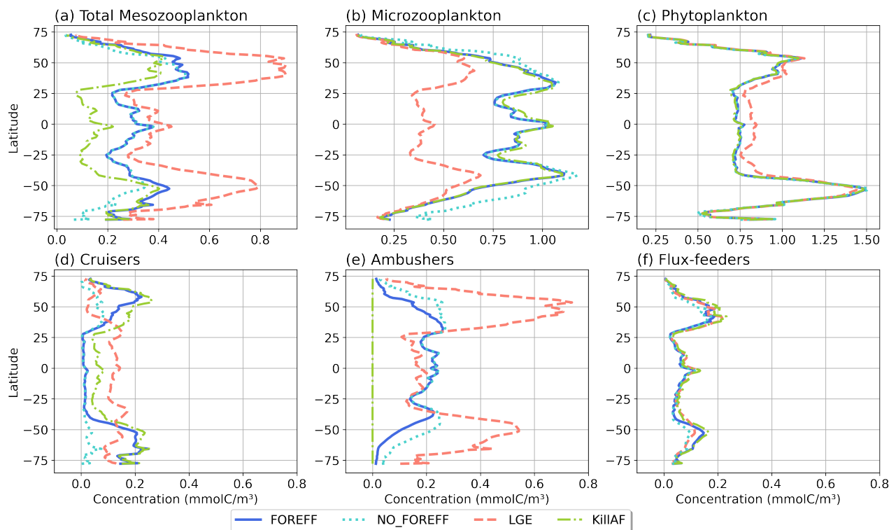
Figure 8. Annual and zonal (averaged over 150 m depth) mean biomass of (a) total mesozooplankton, (b) microzooplankton, (c) phytoplankton, (d) cruisers, (e) ambushers and (f) flux-feeders for the different experiments (in \text{mmolC/m}^3 ): FOREFF in dark blue line, NO_FOREFF in dotted blue is similar to FOREFF but with constant foraging effort, LGE (Low Growth Efficiency) in dashed pink corresponds to same growth rate for suspension feeders but lower growth efficiency for cruisers, and KILL_AF in dash and dotted green is similar to FOREFF but ambushers are removed.
