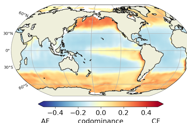
Figure 10. Mean annual codominance index for projections of the Community Weighted Mean (CWM) traits values for the global surface ocean of cruise-feeders (CF) and ambush feeders (AF). This map is based on the dataset for copepods functional groups defined by Benedetti et al. (2023).
