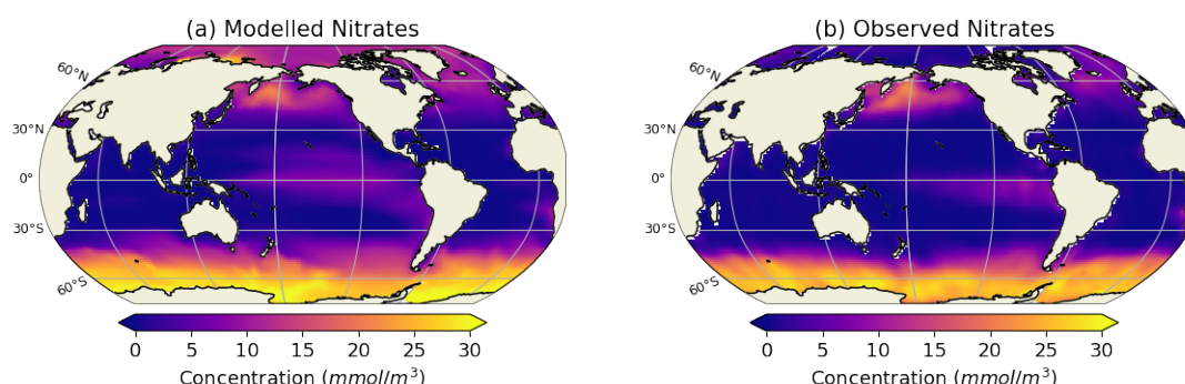
Figure A.2. Comparison between modelled and observed annual average surface nitrates. Observed surface nitrates are from World Ocean Atlas (Garcia et al., 2010b)
