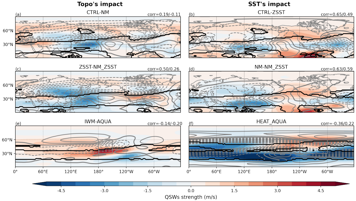
Figure 6. The same as Figure 4Fig. 3, except gray contour-for contours show transient eddies strength and black contour-for contours show stationary wavenumber 4 \leq Ks \leq 8 . The left correlation coefficients are calculated between QSW strength changes and transient eddies strength changes within 4 \leq Ks \leq 8 , while the right correlation coefficients are calculated over all gridboxes grid boxes between 15^\circ – 75^\circ N.
