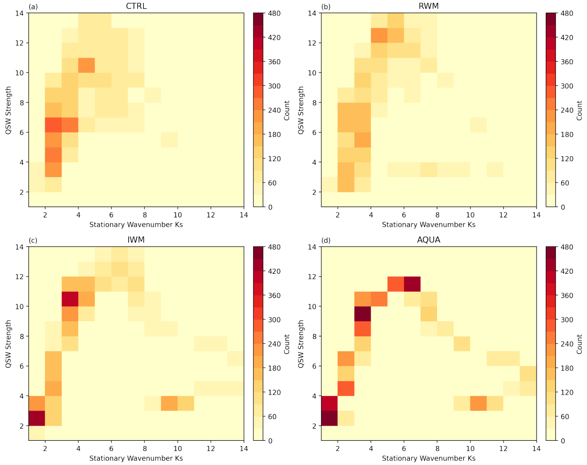
Figure 4. Heatmap showing the number of days during grid points in winter (DJF) climatology that stationary wavenumber Ks is x with a QSW strength of y in Northern Hemisphere . (a) shows the statistics in CTRL, (b) for RWM, (c) for IWM and (d) for AQUA
