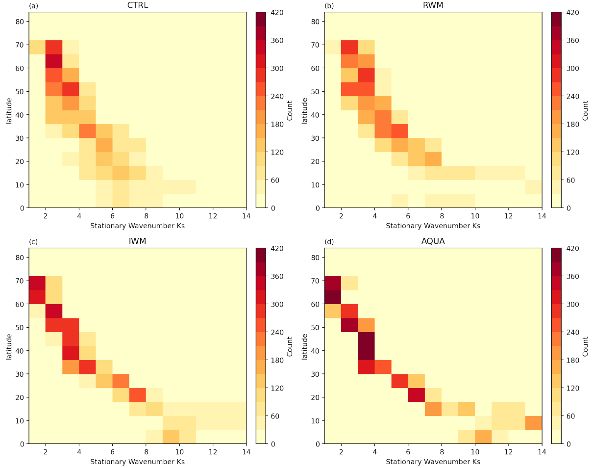
Figure A7. Heatmap shows the count of eases grid points that climatological stationary wavenumber Ks is x at latitude y . (a) shows the statistics in CTRL, (b) for RWM, (c) for IWM and (d) for AQUA
