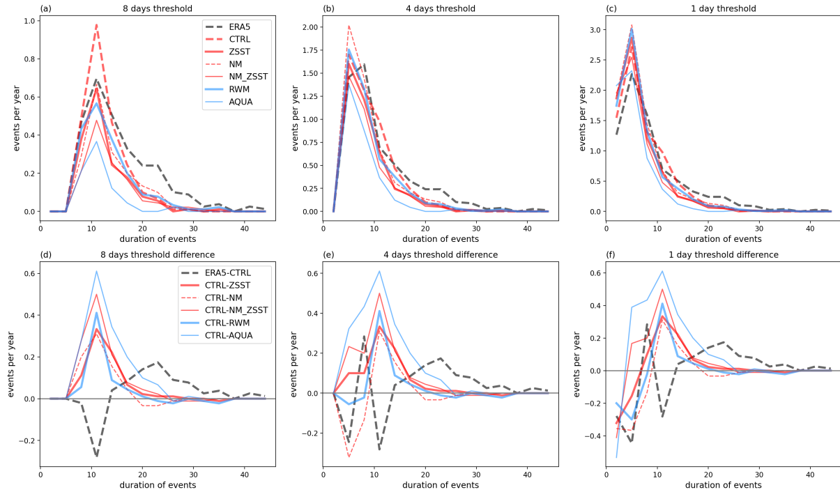
Figure 1. The duration-frequency distribution of QSW events across different experiments within the "North America" region, defined as the area between 60°W and 120°W. The first and second rows show row shows distributions for thresholds of (a) 8 days, (b) 4 days, and (c) 1 day on the QSW metric. In the first row, events are selected based on a fixed frequency, while in the second row, events are selected using a fixed amplitude threshold. The third row shows ERA5-CTRL, as well as the difference between the CTRL and other experiments (as CTRL - experiment) for thresholds of (d) 8 days, (e) 4 days, and (f) 1 day. Events are all selected using a fixed amplitude threshold. The lines are smoothed with 3-day bins on the x-axis. The color coding is as follows: ERA5 is shown in black, experiments with realistic land-ocean contrast are in red, experiments without land surfaces in blue. Dashed lines represent experiments with zonally asymmetric SSTs, while solid lines indicate those with zonally symmetric SSTs. Thick lines correspond to experiments that include topography, whereas thin lines represent experiments without topography.
