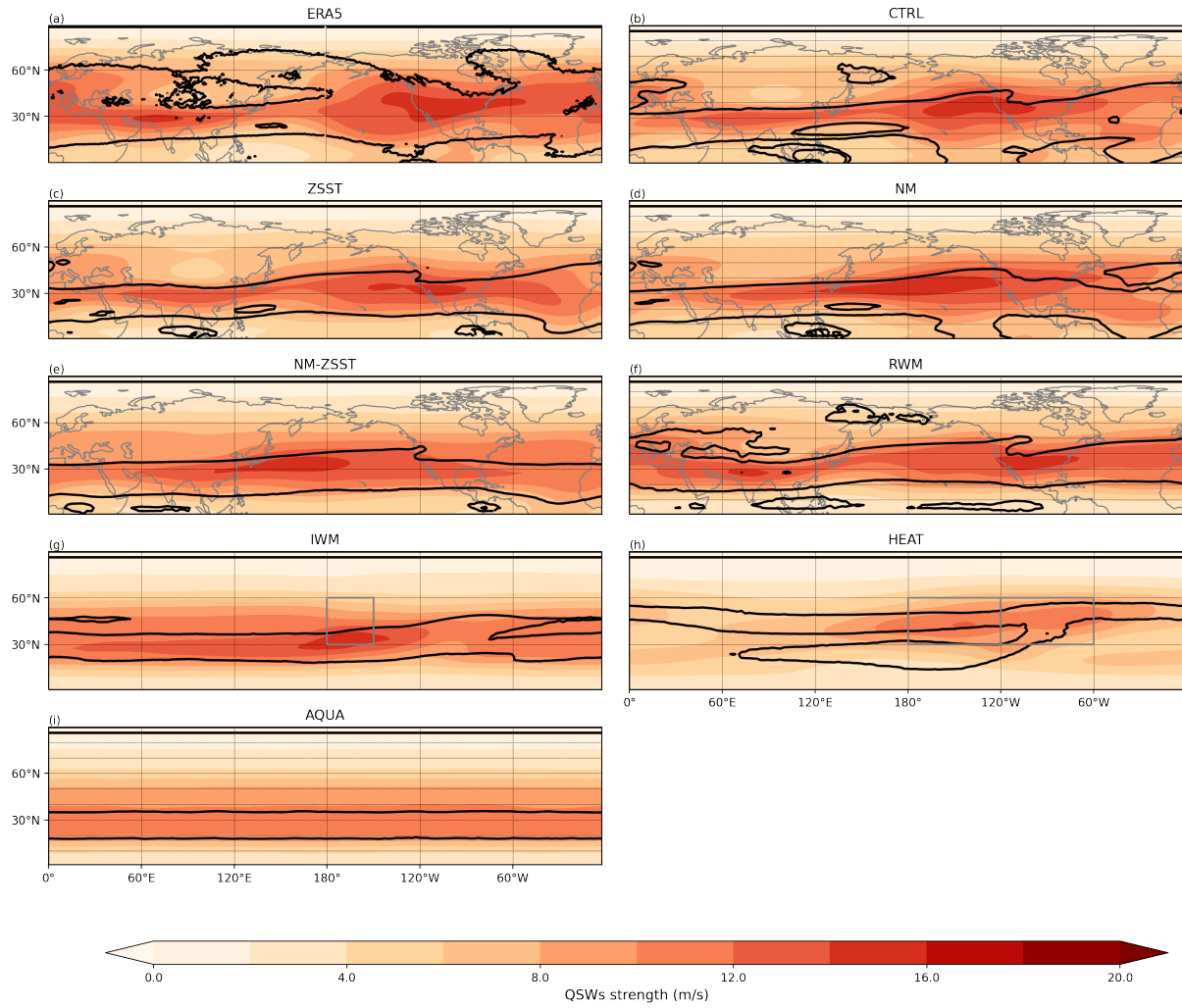
Figure A5. Climatological QSW strength in winter (shading) and stationary wavenumber Ks=4 and Ks=8 (contour). Other information is the same as Figure Fig. A3
