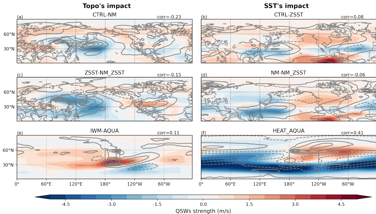
Figure 7. The same as Figure 4 Fig. 3, except for Eady growth rate at 700 hPa (contour; the interval is 0.1 per day).
