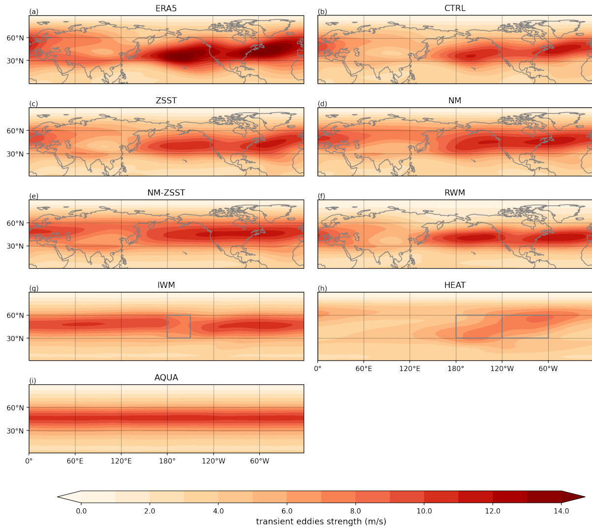
Figure A6. This figure shows climatological transient eddy strength. Other information is the same as Figure Fig. A3
