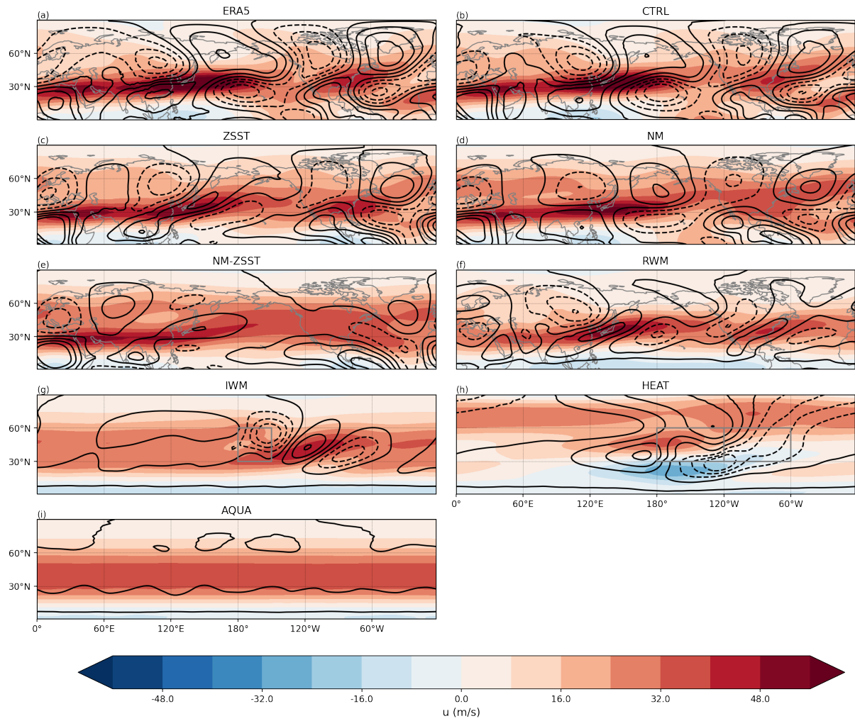
Figure A4. Climatological zonal wind in winter (shading) and climatological meridional wind (contour). Other information is the same as Figure Fig. A3
