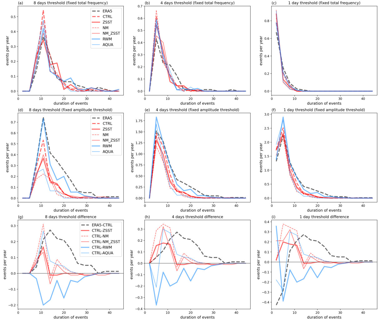
Figure A1. The same as Figure 1, except for This figure shows statistics in Europe (0-60°E). The first row is same as the first row in Fig. 1, and the third row is the same as the bottom row in Fig. 1. In the second row, the threshold for QSW events is determined based on event frequency, allowing it to vary across simulations in order to maintain a fixed event frequency across all simulations and ERA5.
