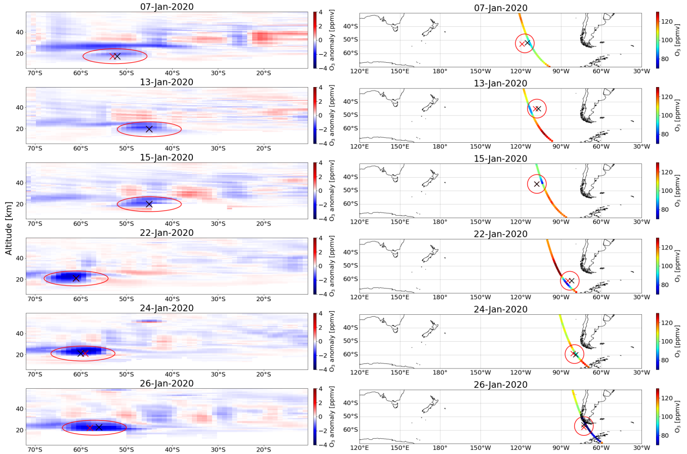
180 Figure 2: OMPS-LP ozone anomalies for selected days following the Australian fires, with a latitude/altitude plot (left column). OMPS-LP ozone observation concentration at the core vortex altitude from ECMWF IFS (right column). The circle represents the rough shape of the vortex (~1000 km diameter, in the panels). The red and black crosses show the center of the vortex according to the ECMWF-IFS reanalyses at 6UTC and 18UTC, respectively.
