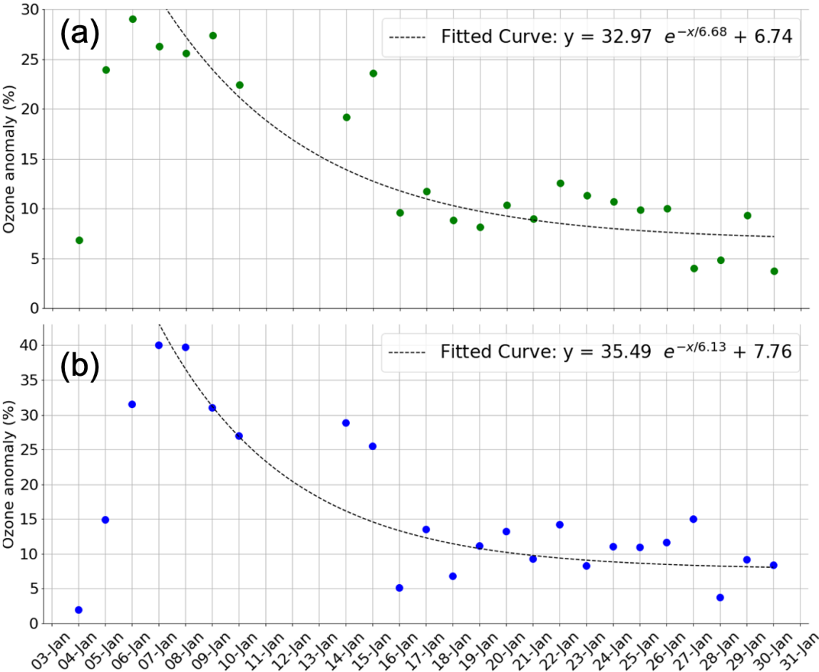
260 Figure 6: Temporal evolution of the partial stratospheric ozone column anomaly (percent reduction) for the in-vortex ozone mini-hole observed by IASI, using the spatial background method (see Fig. 4) (a) and using the temporal background method (see Fig. 5) (b). An exponential-decay fit is applied to the two time series and the fitted equation is in the respective panels (y is the ozone percent anomaly and x is time in days).
