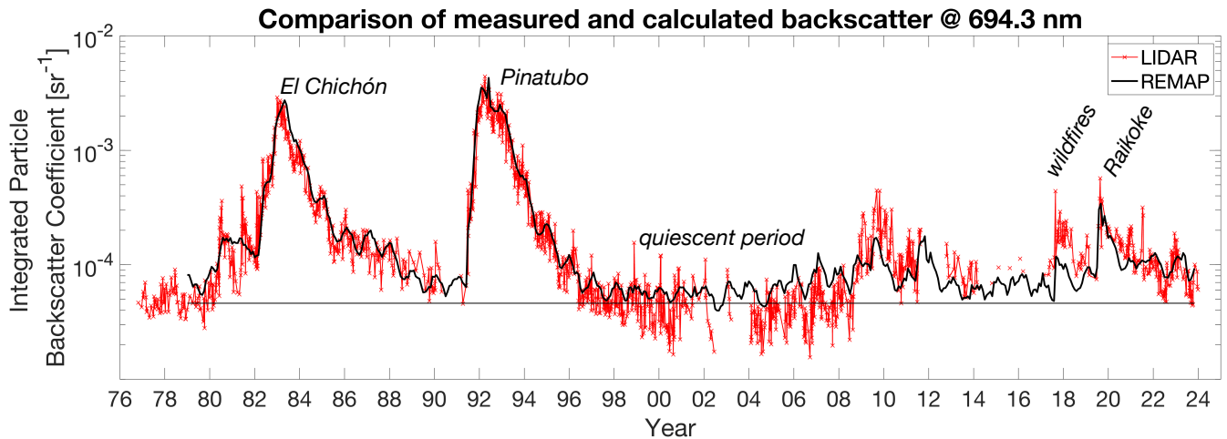
Figure 9. Integrated backscatter coefficients of stratospheric aerosol (integrated from 1 km above the tropopause to the upper end of the layer) over Garmisch-Partenkirchen, Germany (47.48° N, 11.06° E, 734 m asl). Red symbols and line: measured by the ground based LIDAR at 694.3 nm. Several significant events are marked: the volcanic eruptions of El Chichón 1982, Pinatubo 1991 and Raikoke 2019, an extended quiescent period in 1997-2004 and the British Columbia (BC) wildfires. From Trickl et al. (2023). Black line: zonal average monthly mean integrated backscatter coefficients for the latitude band 45° N to 50° N calculated from GloSSACv2.22 using REMAP with the parameterization \sigma(\beta_{1022}) (Eq. (4)).
