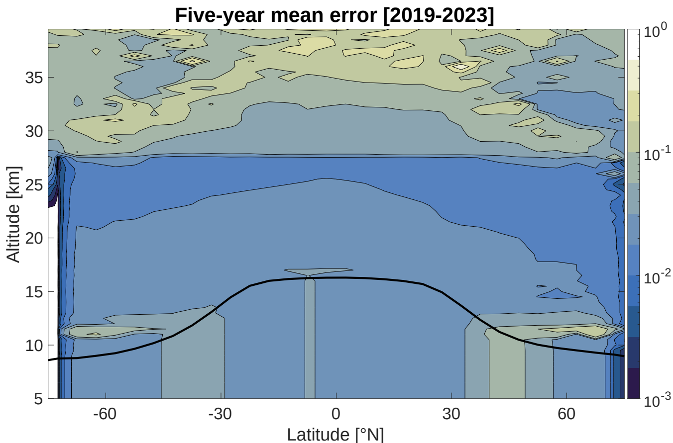
Figure 2. Latitude-altitude plot of the 5-year mean error from a retrieval of 6 SAGE III wavelengths where available and gaps filled with GloSSACv2.22. The black line indicates the average tropopause height. The Junge layer is discernible from the minimum error values. The distinct rise in error above 27 km at all latitudes comes from the observational data set GloSSACv2.22 itself, which includes a high-altitude climatology.
