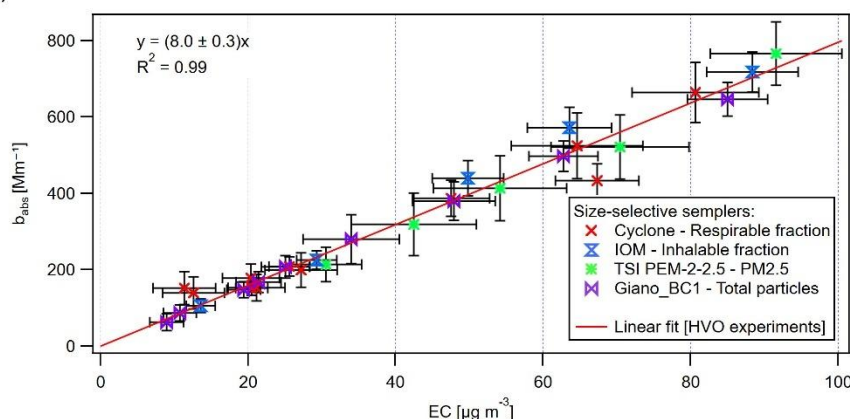
Figure 4 Absorption coefficient ( b_{\text{abs}} ) at 635 nm, measured by MWA vs. EC concentration ( \mu\text{g m}^{-3} ) for propane flame particles (a), commercial diesel exhaust particles (b) and HVO exhaust particles (c). For each classifier the corresponding particle size-selective sampling convention is also indicated. Linear fits (red lines) are plotted, with slopes representing the MAC values. The correlation coefficients ( R^2 ) for each fit are also provided.
