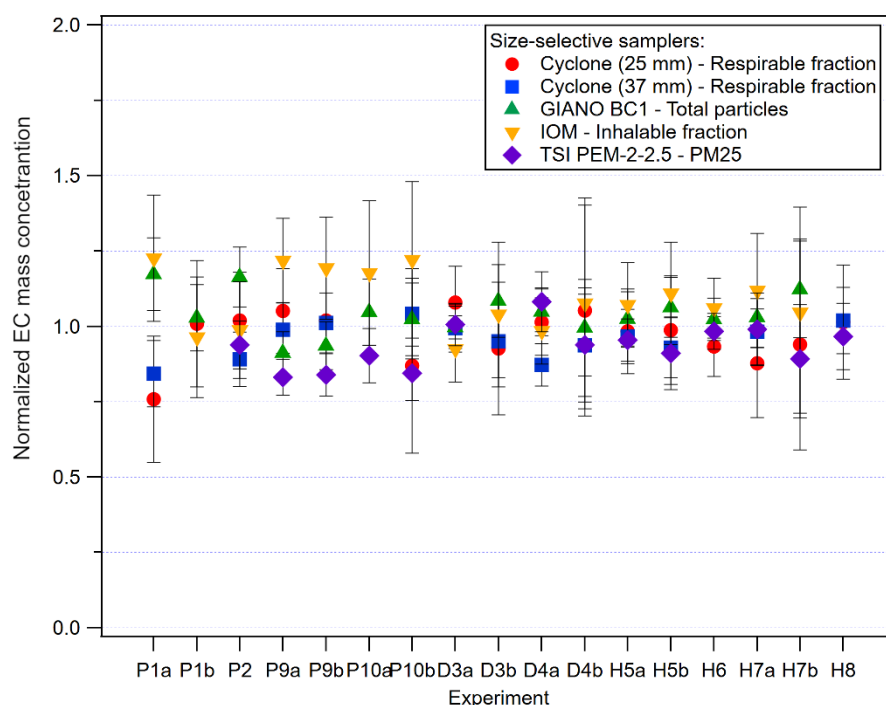
Figure 2 Normalized EC mass concentration across different experiments. All selectors operated simultaneously within the same time period. In order to help in the interpretation of data values have been normalized to a scaling factor equal to the mean value of each dataset (i.e. mean values of EC mass concentration retrieved from filters analysis during each experiment).
