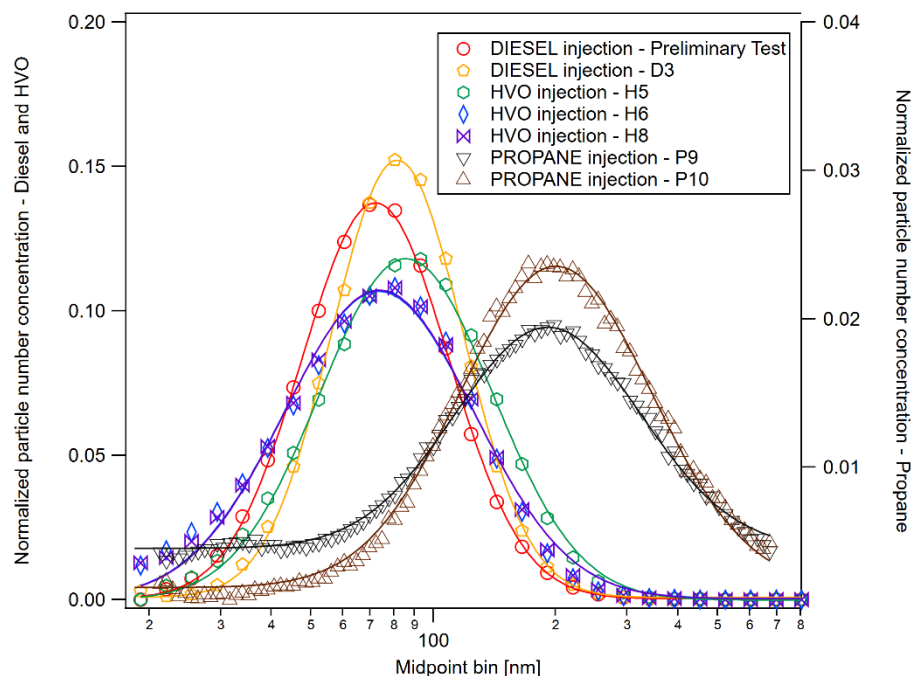
Figure 3 Number size distribution measured (markers) and fit extrapolated log-normal size distribution (lines) of generated aerosols just after the injection in ChAMBRé. Size data are normalized by the total number for each distribution.
