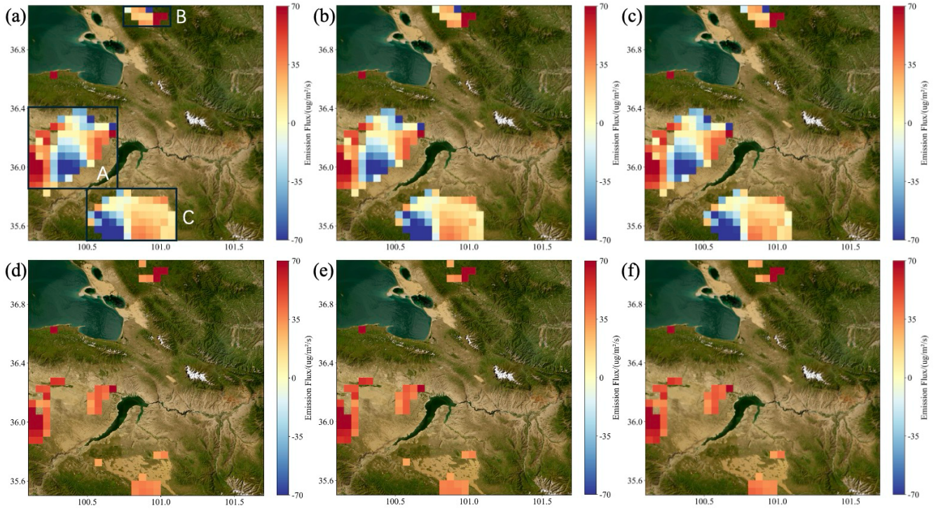
Figure 4: (a), (b), and (c) are maps of five-year emission averages calculated using TROPOMI XCH 4 , XCH 4 ±10%, and XCH 4 ±20% respectively; (d), (e) and (f) are maps of the five-year emission average obtained after the two-step filtering is applied corresponding to (a), (b), (c). All backgrounds are from Esri World Imagery.
