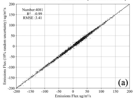
Emission VS Emission (XCH4±10%)
