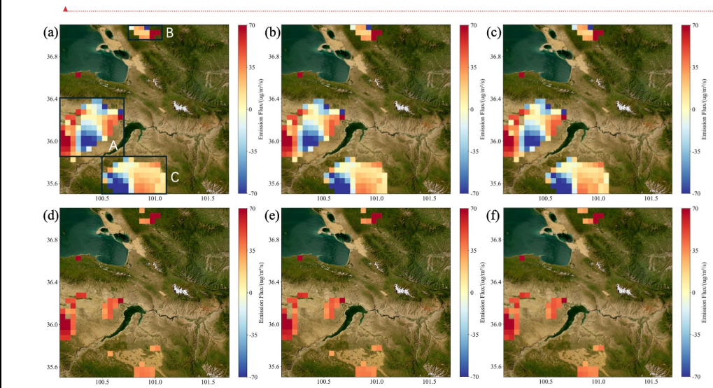
375 Figure 4: (a), (b), and (c) are maps of five-year emission averages calculated using TROPOMI XCH 4 , XCH 4 ±10%, and XCH 4 ±20% respectively; (d), (e) and (f) are maps of the five-year emission average obtained after the two-step filtering is applied corresponding to (a), (b), (c). All backgrounds are from Esri World Imagery.
