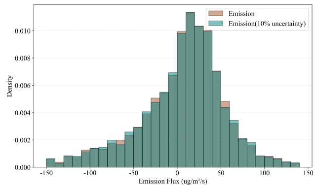
Figure 2: PDF of methane emissions from the Waliguan region calculated using TROPOMI \text{XCH}_4 and \text{XCH}_4 \pm 10\% based on the mass conservation model.
