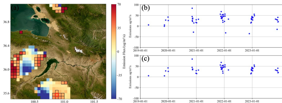
Figure 3: (a) Five-year emission mean calculated by TROPOMI \text{XCH}_4 , the mean of the grids in the black boxes are greater than the set threshold ( 12.4 \text{ ug/m}^2/\text{s} ) (background portion of image is from Esri World Imagery); (b) and (c) are the unfiltered and filtered emission time series of the red grid in (a).
