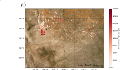
Figure 7: (a) Annual mean CH 4 emissions (kg/h/TROPOMI grid) on grids which overlap spatially with an emission observed by Cusworth (2021); (b) The red dots in the scatter plot represent the points where our emission results overlap with those of Cusworth (2021) in both space and time and the difference is within 2 times. The black dots represent our emission results that overlap in space but do not overlap in time. The gray bars indicate the error range. Backgrounds of (a) is from Esri World Imagery.
