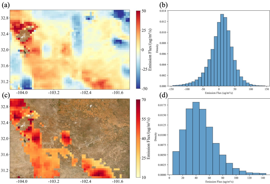
565 Figure 6: (a) Annual mean methane emission fluxes from the Permian Basin for 2019-2020, (b) PDF of the Permian Basin emission 570 fluxes for 2019-2020, (c) Annual mean methane emission fluxes from the Permian Basin after filtration in 2019-2020, (d) PDF of the 2019-2020 methane emission fluxes from the Permian Basin after filtration. Backgrounds of (a) and (c) are from Esri World Imagery.
