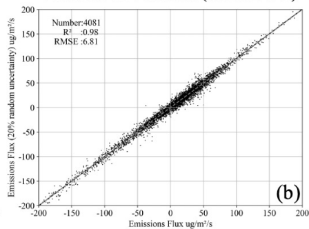
Emission VS Emission (XCH4±20%)
