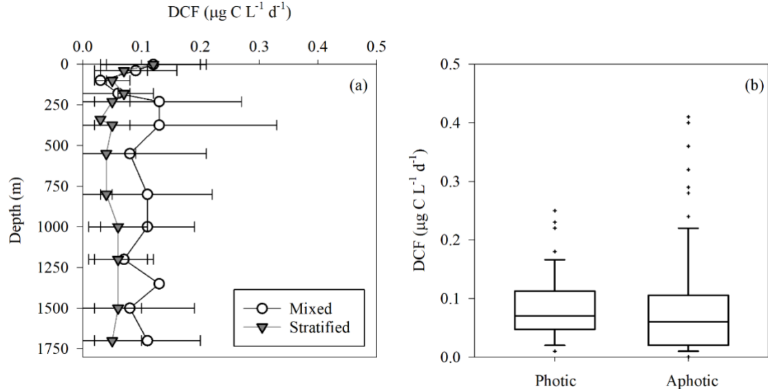
Figure 2: Dark carbon fixation rates in the southeastern Mediterranean Sea. Averaged vertical distribution of DCF in the offshore southeast Mediterranean Sea during the mixed (white) and stratified (gray) periods (a), and a box plot showing the DCF rates at the photic (0-180 m) and aphotic (>180 m) water depths (b).
