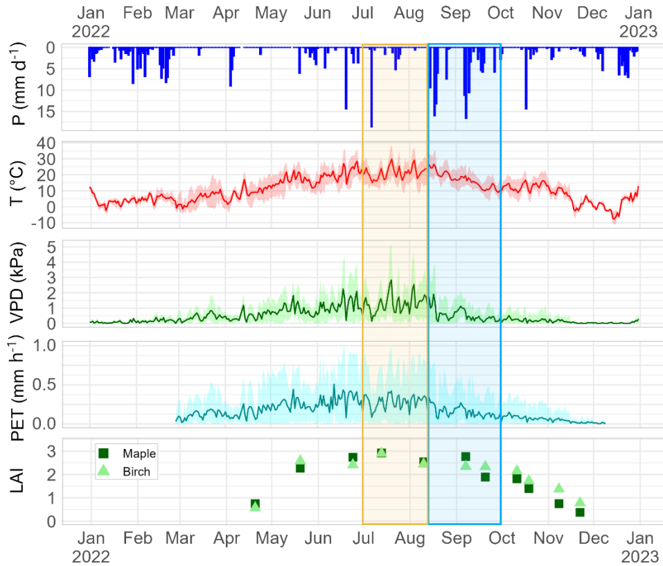
Figure 2: Hydroclimatic Context 2022: Precipitation [ \text{mm d}^{-1} ] is shown as daily sum. Temperature [ ^{\circ}\text{C} ], VPD [ \text{kPa} ] and PET [ \text{mm/h} ] are shown as daily mean values with daily min/max band. Leaf Area Index (LAI) is shown as daily mean values. Periods of interest are shown as an orange box (summer drought 01.07.-14.08.2022) and blue box (rewetting 15.08.-30.09.2022). Figure adapted from Ring et al. (2024).
