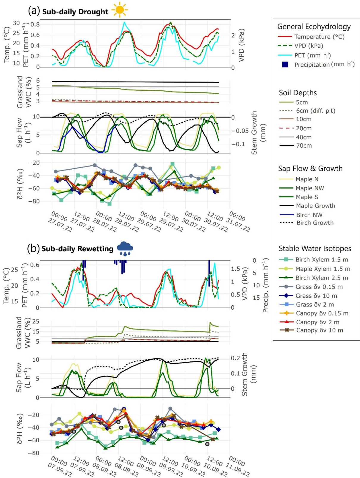
Figure 5: Sub-daily timeseries displaying diurnal variation of tree xylem water ( \delta_{\text{xt}} ) and atmospheric vapor ( \delta_v ) and measured ecohydrological variables during (a) drought conditions and (b) rewetting.
