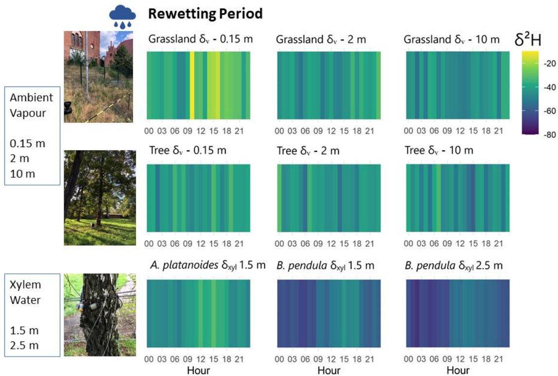
Figure 4: 24-h cycle heatmap of hourly median \delta^2\text{H} data of tree xylem water ( \delta_{\text{xyl}} ) and atmospheric vapor ( \delta_{\text{v}} ) during rewetting period 15.08.-30.09.2022. One in situ measurement loop took \sim 3.5\text{h} and unstable measurements were ruled out (cf. Method section). The hourly median shown for each hour of the day was calculated based on \sim 9.2 measurements).
