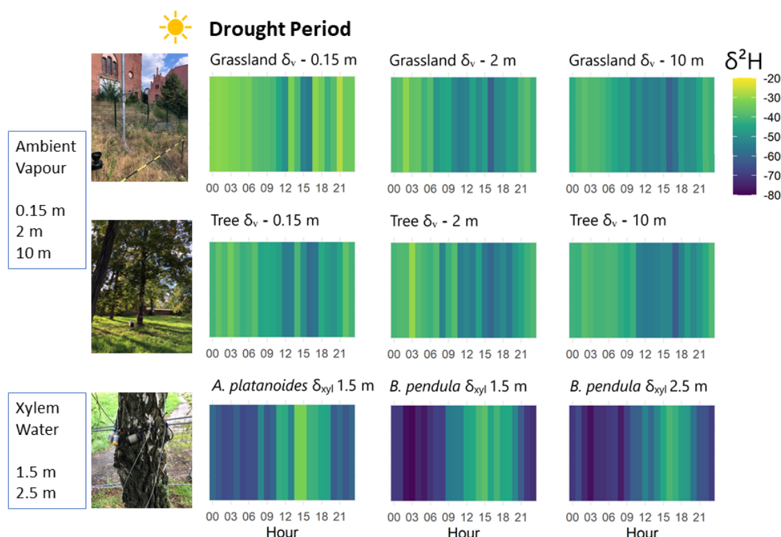
Figure 3: 24-h cycle heatmap of hourly median \delta^2H data of tree xylem water ( \delta_{xyl} ) and atmospheric vapor ( \delta_v ) during summer drought period 01.07.-14.08.2022. One in situ measurement loop took ~3.5 h and unstable measurements were ruled out (cf. Method section). The hourly median shown for each hour of the day was calculated based on ~8.6 measurements.
