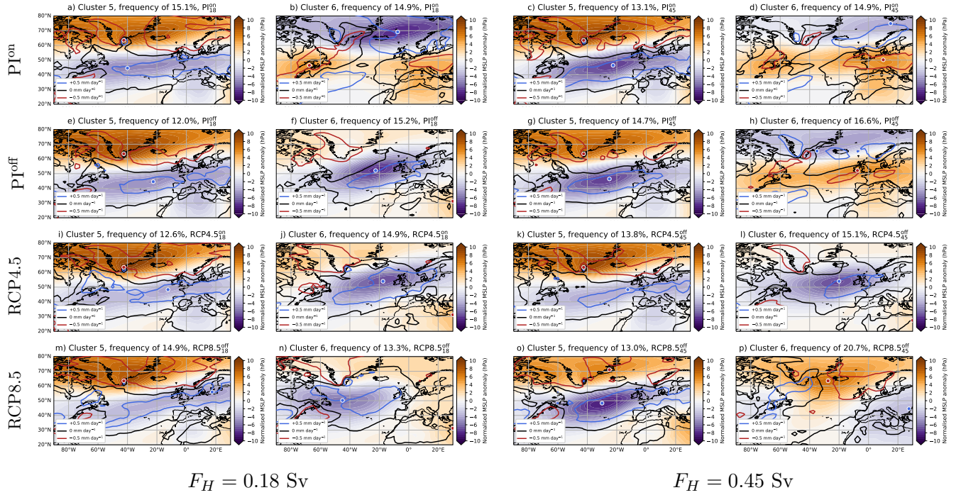
Figure A5. Similar to Figure 8, but now for clusters 5 and 6.
