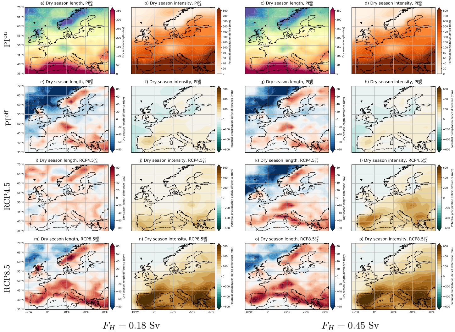
Figure 4. (First and third column): The dry season length and (second and fourth column): the dry season intensity. For the PI^{off} , RCP4.5 and RCP8.5 scenarios, the dry season length and intensity are displayed as the difference compared to their PI^{on} scenario.
