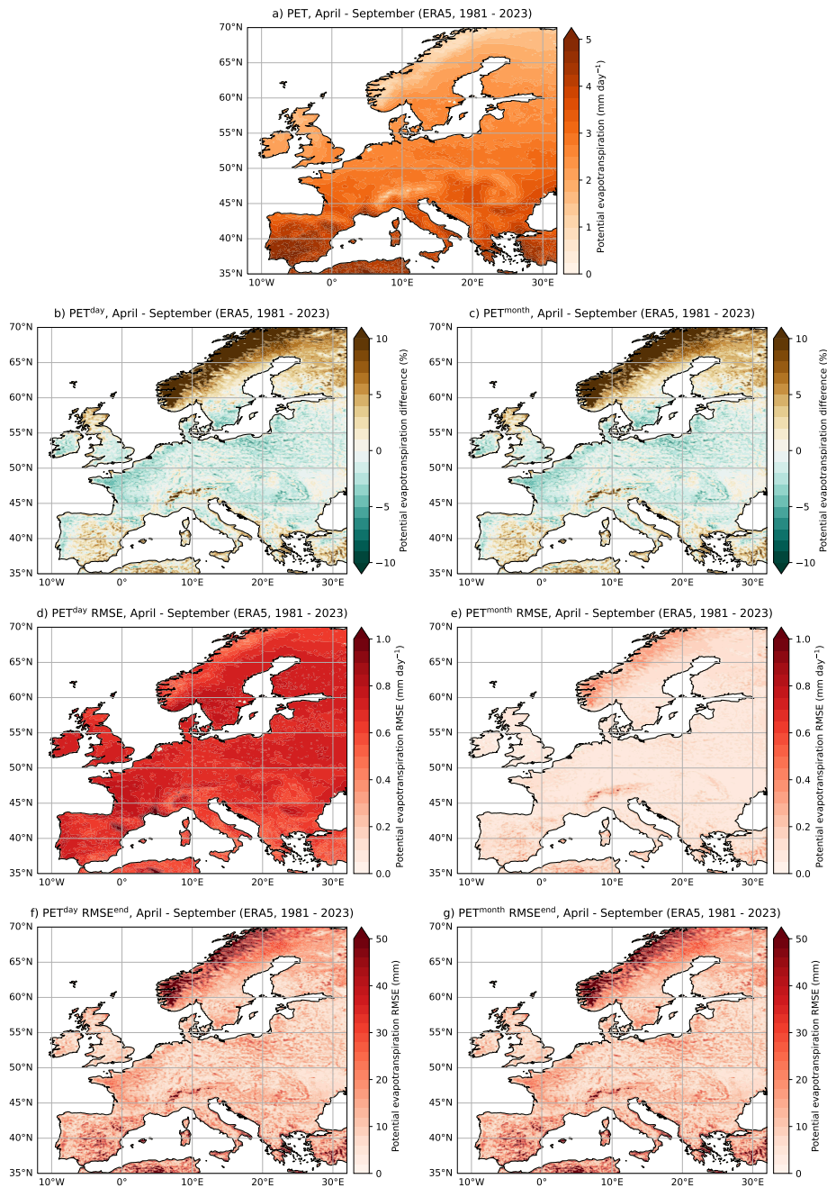
Figure A1. (a): The hourly-averaged PET (i.e., truth) for the growing season (April – September) in ERA5 (1981 – 2023). (b & c): Similar to panel a, but now the PET^{\text{day}} and PET^{\text{month}} expressed as the relative difference from PET. (d & e): The root-mean-square error (RMSE) for PET^{\text{day}} and PET^{\text{month}} against the hourly-averaged PET. For example, the local and daily RMSE was determined as RMSE = \sqrt{\frac{1}{T} \sum_{t=1}^T \left( PET^{\text{day}}(t) - \overline{PET}(t) \right)^2} , with T the number of days and \overline{PET} the daily-averaged PET (from hourly averages). (f & g): The RMSE at the end of the growing season by integrating hourly-averaged PET, PET^{\text{day}} and PET^{\text{month}} over the growing season (e.g., PET^{\text{end}} = \int_{1 \text{ Apr}}^{30 \text{ Sep}} PET(t') dt' ). For example, the local and daily RMSE at the end of the growing season was then determined as RMSE^{\text{end}} = \sqrt{\frac{1}{Y} \sum_{t=1}^Y \left( PET^{\text{day,end}}(t) - PET^{\text{end}}(t) \right)^2} , with Y the number of years.
