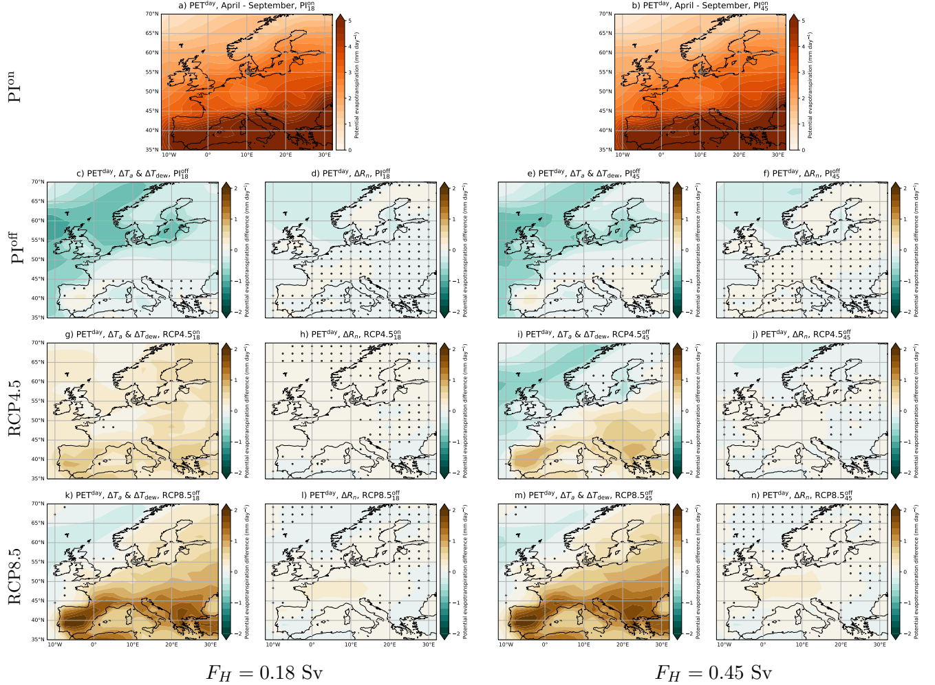
Figure 6. (a & b): The PET^{\text{day}} rates during the growing season (April – September) for PI^{\text{on}} . (c – n): The PET^{\text{day}} differences during the growing season (April – September) for PI^{\text{off}} , RCP4.5 and RCP8.5. The PET^{\text{day}} responses are decomposed into a temperature contribution (i.e., \Delta T_a & \Delta T_{\text{dew}} , first and third column) and net surface radiation contribution (i.e., \Delta R_n , second and fourth column). The markers indicate non-significant ( p \geq 0.05 , two-sided Welch's t-test) differences.
