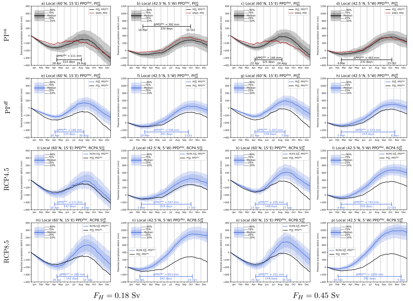
Figure A3. Similar to Figure 3, but now for 60°N and 15°E (Sweden) and 42.5°N and 5°W (Spain). Note the different vertical ranges between the two locations.
