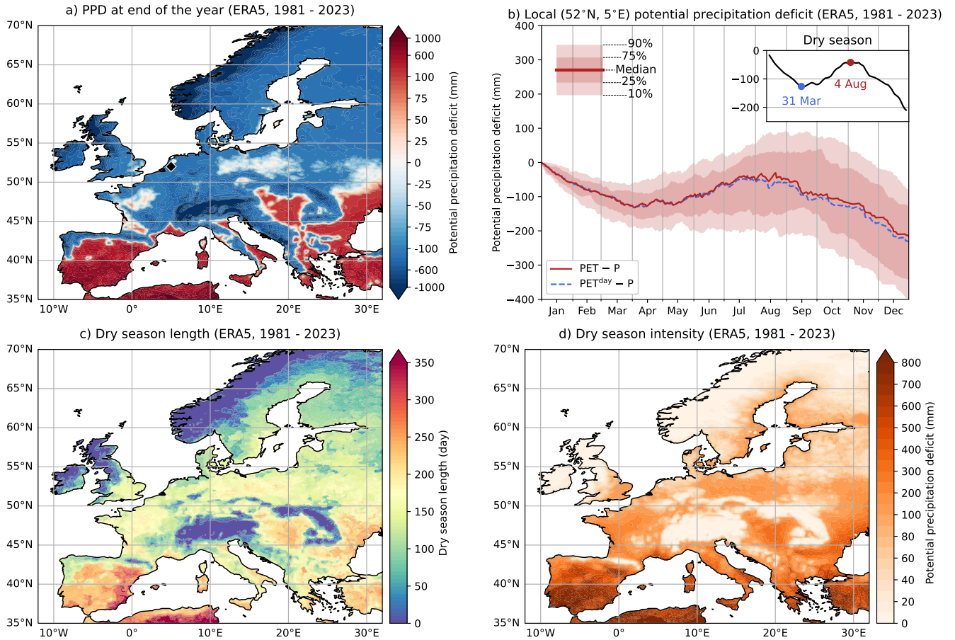
Figure 2. (a): The climatological potential precipitation deficit (PPD) at the end of the year for ERA5 (1981 – 2023). The PPD was determined using daily-averaged hourly-averaged PET and precipitation rates( determined from hourly-averages ). Here we show the median PPD over the available 43-year period. (b): The local PPD at 52°N and 5°E (the Netherlands, diamond marker in panel a). The inset shows the dry season, which is derived from the climatological median PPD smoothed with a 15-day moving average. The climatological dry season at 52°N and 5°E starts on 31 March (PPD = –127 mm) and ends on 4 August (PPD = –42 mm), with a dry season intensity of 85 mm. The median PPD day is also shown (blue dashed curve). Spatial patterns of (c): the dry season length and (d): the dry season intensity.
