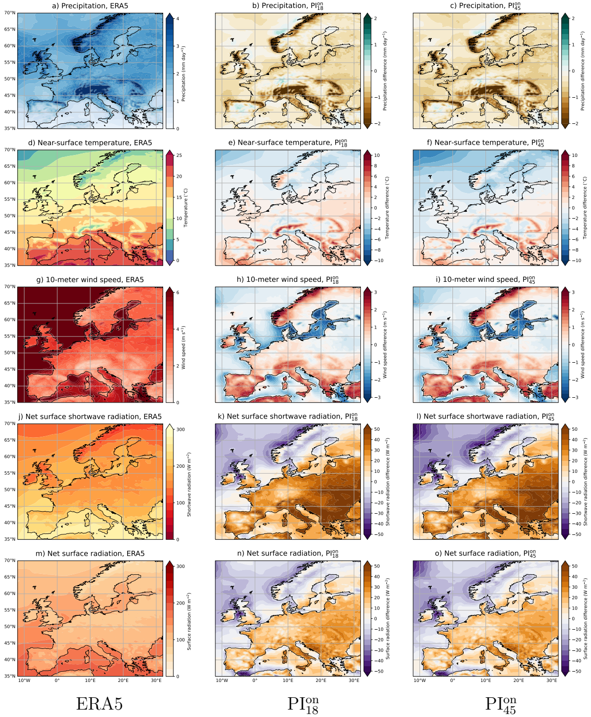
Figure A2. The precipitation, near-surface (2-meter) temperatures, 10-meter wind speed, net surface shortwave radiation, and net surface radiation for ERA5 (1981 – 2023), PI_{18}^{on} and the two AMOC-on scenarios PI_{45}^{on} . The climate variables are determined over the growing season (April – September). For the AMOC-on PI_{45}^{on} scenarios, the climate variables are displayed as the difference compared to ERA5.
