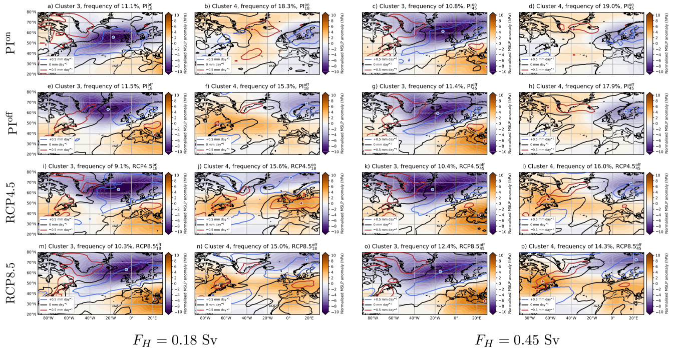
Figure A4. Similar to Figure 78, but now for clusters 3 and 4.
