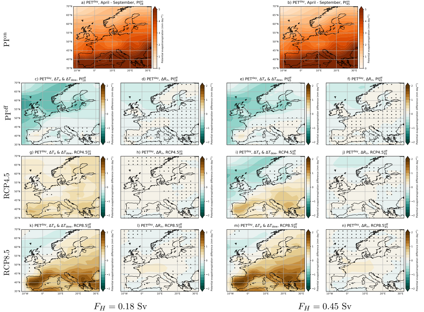
Figure 6. (a & b): The PET day rates during the growing season (April – September) for AMOC-on PI on . (c – n): The PET day differences during the growing season (April – September) for AMOC-off PI off , RCP4.5 and RCP8.5. The PET day responses are decomposed into a temperature contribution (i.e., \Delta T_a & \Delta T_{\text{dew}} , first and third column) and net surface radiation contribution (i.e., \Delta R_n , second and fourth column). The markers indicate non-significant ( p \geq 0.05 , two-sided Welch's t-test) differences.
