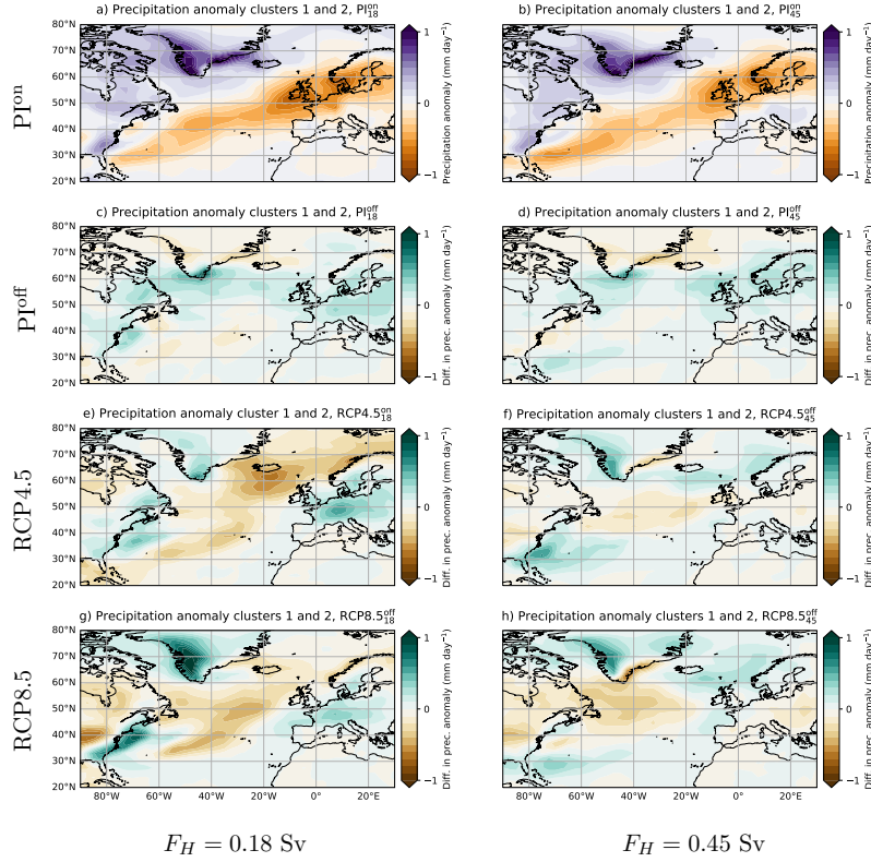
Figure 9. The precipitation anomaly patterns from the k -means clustering algorithm for P_{1,2}^{ref} ( AMOC_{on}PI_{on}^{ref} ) and \Delta P_{1,2} ( AMOC_{off}PI_{off}^{ref} , RCP4.5 and RCP8.5).
