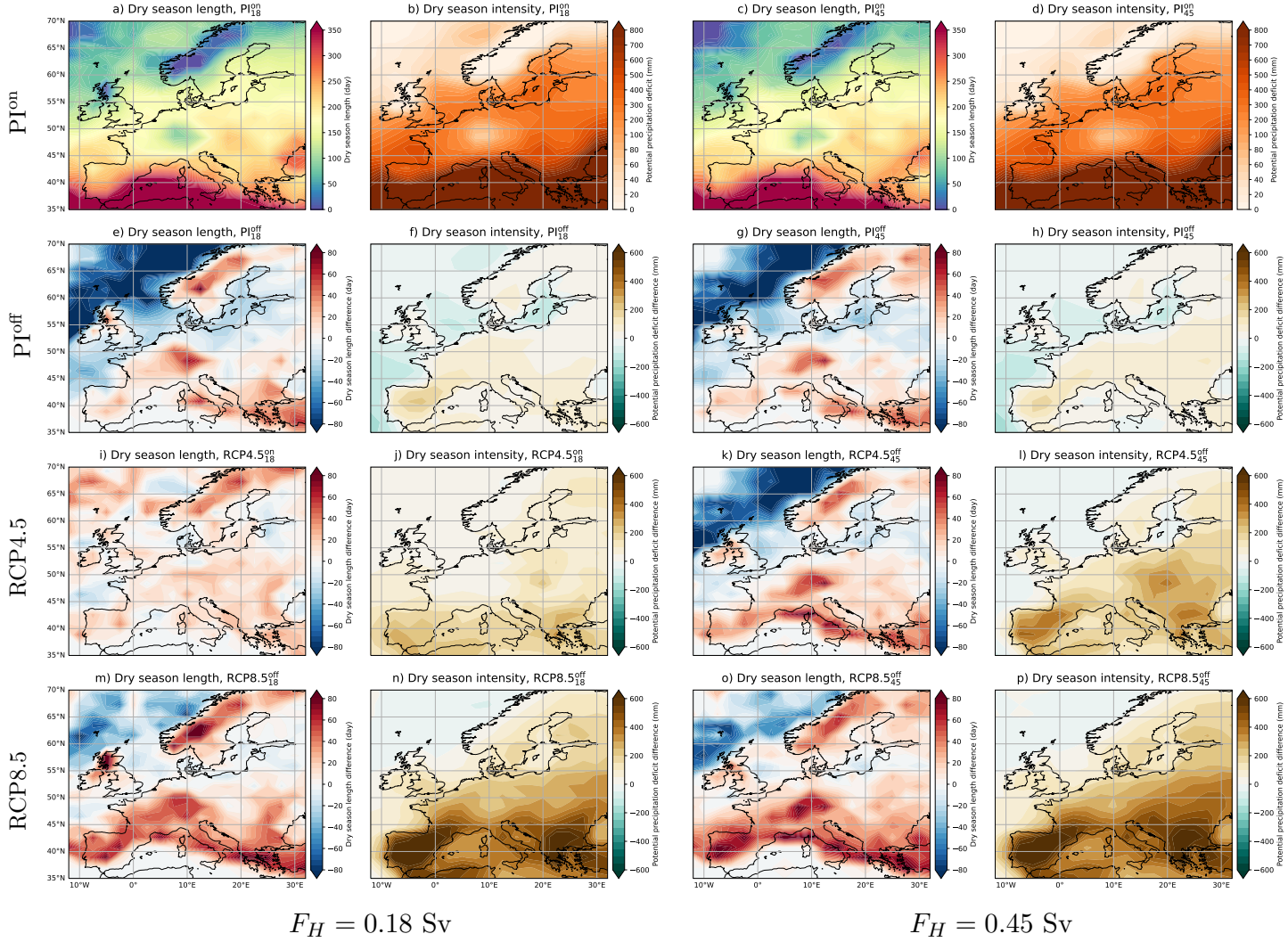
Figure 4. (First and third column): The dry season length and (second and fourth column): the dry season intensity. For the AMOC off \text{PI}^{\text{off}} , RCP4.5 and RCP8.5 scenarios, the dry season length and intensity are displayed as the difference compared to their AMOC on reference \text{PI}^{\text{on}} scenario.
