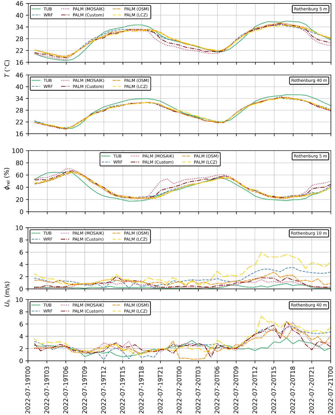
Figure 17. Comparison of WRF and PALM results of temperature T , relative humidity \phi_{\text{rel}} and horizontal wind speed U_h against measurements from the TUB tower at “Rothenburgstraße” (located in nested domain).
