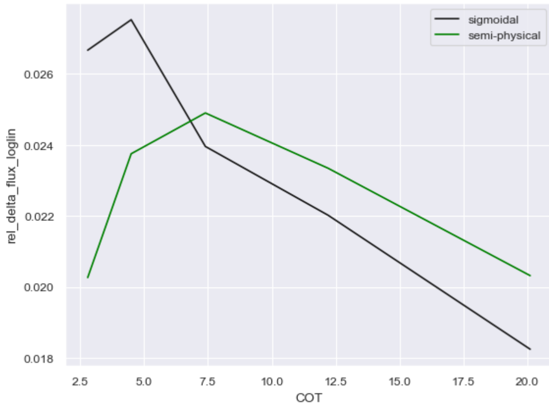
Fig 1.: Relative Flux deviation for different tau
