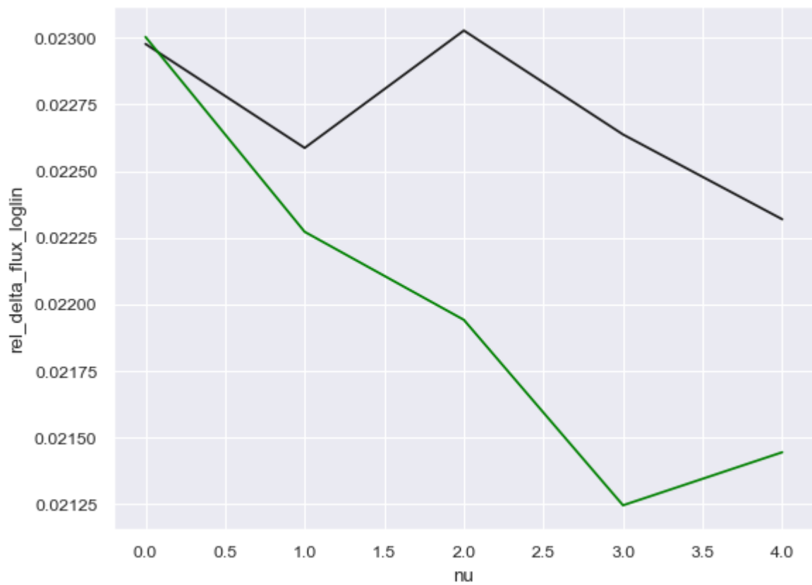
Fig 2.: Relative Flux deviation for different nu
