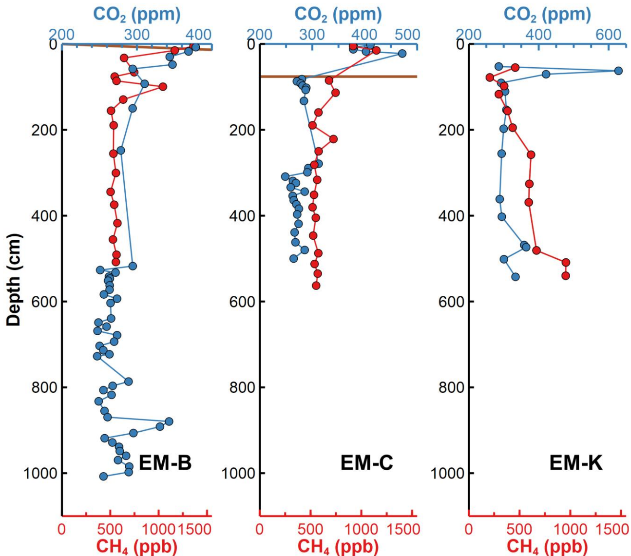
225 Figure 3. Vertical profiles of CO 2 and CH 4 concentrations in Elephant Moraine blue ice. The CO 2 concentration was measured by a dry-extraction system in SNU. The CH 4 concentration was measured by a wet-extraction system in SNU. Brown lines indicate the dust band identified in the EM-B and EM-C ice cores. The dust band in EM-B has a dip of 59°, whereas the dust band in EM-C is parallel to the surface (Jang et al., 2017).
