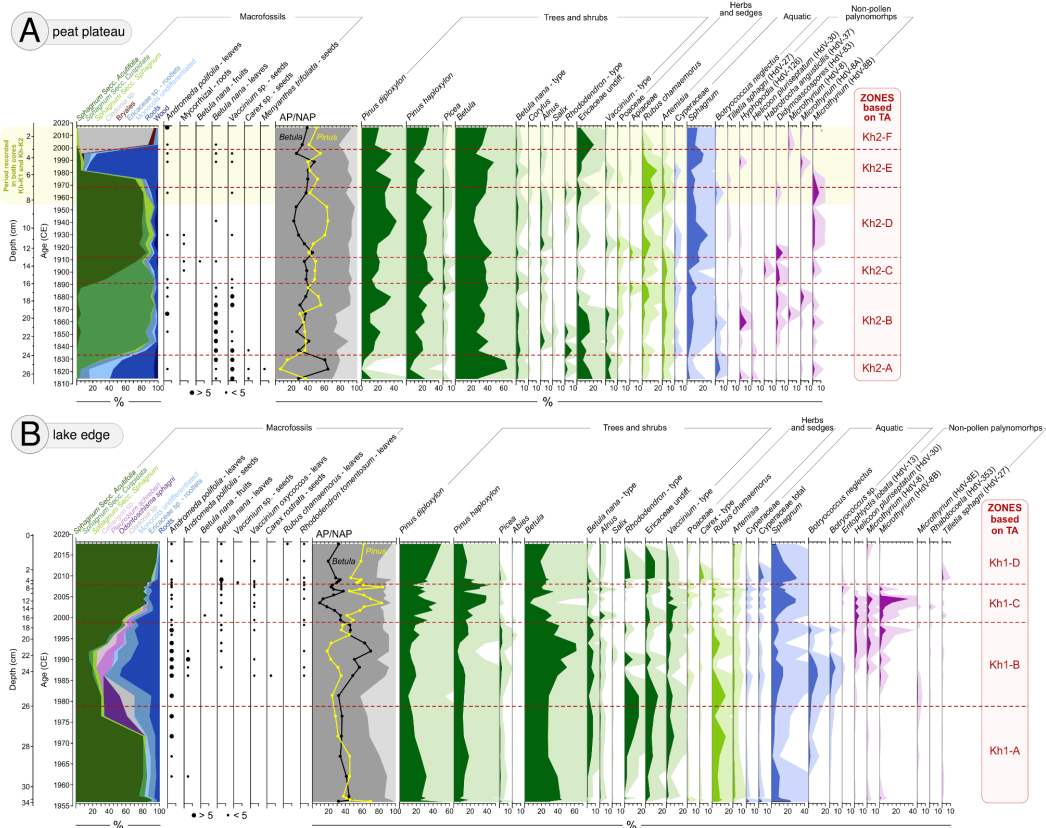
Figure 5 Macrofossils and pollen diagram with 5× exaggeration from peat cores: A) Kh-K2 and B) Kh-K1. The subfossil vegetative fragments and carpological remains are represented as either present or absent in each sample. Zonation based on testate amoebae CONISS was added to the graph.
