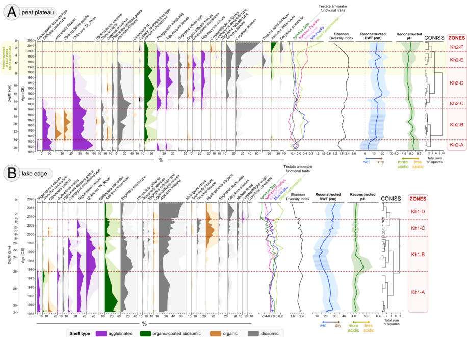
Figure 3 Testate amoebae (TA) diagram (abundance >3%) with 5× exaggeration for peat cores: A) Kh-K2 and B) Kh-K1. TA species are grouped by shell type, as indicated by the colour legend below the plot. The diagram includes community-weighted TA functional traits, Shannon Diversity Index, reconstructed depth to water table (DWT) based on Halaš et al. (2023), and reconstructed pH based on Qin et al. (2021). Shaded areas for DWT and pH represent bootstrap reconstruction errors. The hatching on the DWT indicates a reconstruction potentially affected by error due to the presence of >25% of a new TA species. Species are sorted by weighted average (WA). Zonation was based on testate amoebae CONISS.
