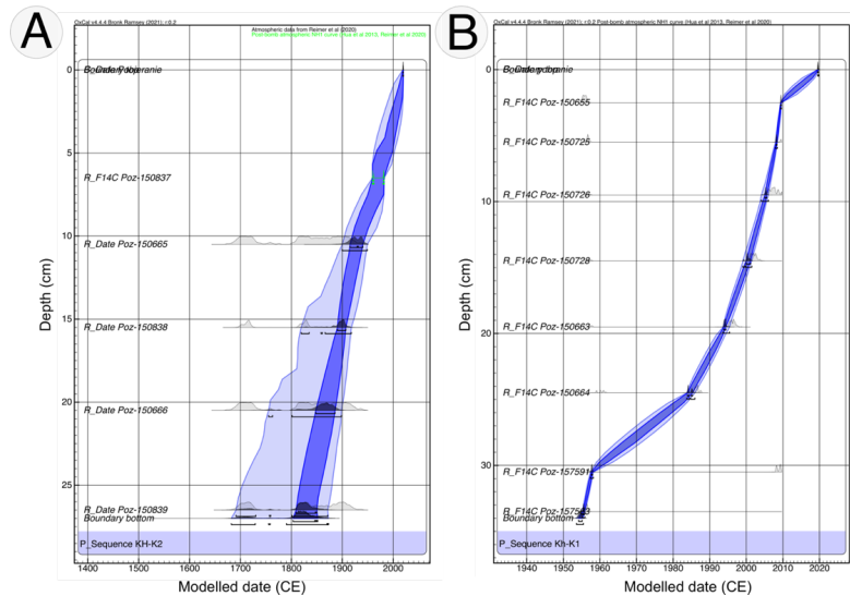
Figure 2 Age-depth models based on C^{14} dating for core A) Kh-K2 and B) Kh-K1. The dark and light blue areas provide the 1\sigma and 2\sigma calibrated age range, respectively.
