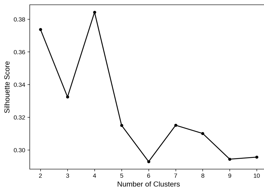
Figure 1 Silhouette Score for different number of clusters in testate amoebae samples from the Kh-K1 core. The highest silhouette score is observed at four clusters.
