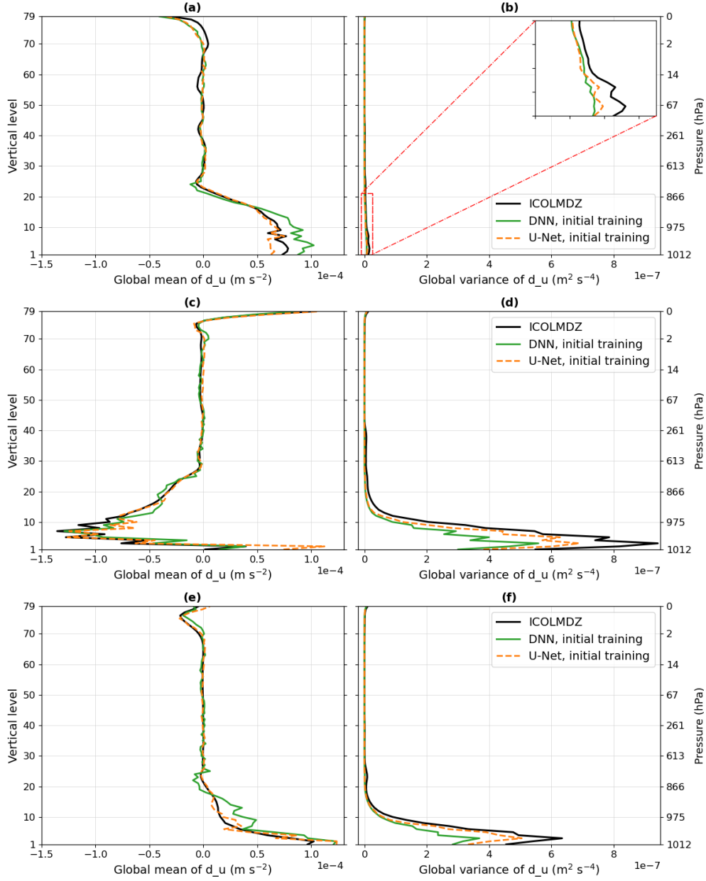
Figure 5. Global vertical profiles of the zonal wind tendency d_u of the mean (left) (a-c-e) and the variance (right) (b-d-f) for the test subset, obtained with the initial approach. Figures (a) and (b) correspond to the tropics ( \phi \in [25^\circ \text{ S}; 25^\circ \text{ N}] ), figures (c) and (d) represent the subtropical regions ( \phi \in [45^\circ \text{ S}, 25^\circ \text{ S}] \cup [25^\circ \text{ N}, 45^\circ \text{ N}] ) and figures (e) and (f) are the high latitudes ( \phi \in [90^\circ \text{ S}, 45^\circ \text{ S}] \cup [45^\circ \text{ N}, 90^\circ \text{ N}] ). The data from the ICOLMDZ simulation are represented by the black curves. The blue-green curves come from the DNN and the dashed orange curves represent the U-Net, for the initial training.
