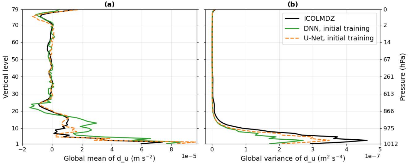
Figure 3. Global vertical profiles of the zonal wind tendency d_u of the mean (left) (a) and the variance (right) (b) for the test subset. Figures (a) and (b) show, obtained with the results of the initial training, while figures (c) and (d) correspond to the second training where physical knowledge is added. In these figures, the black curves represent the reference data from the ICOLMDZ simulation. The blue and green curves correspond to predictions made by DNNs the DNN while the dashed orange and red curves represent the results obtained using U-Nets the U-Net.
