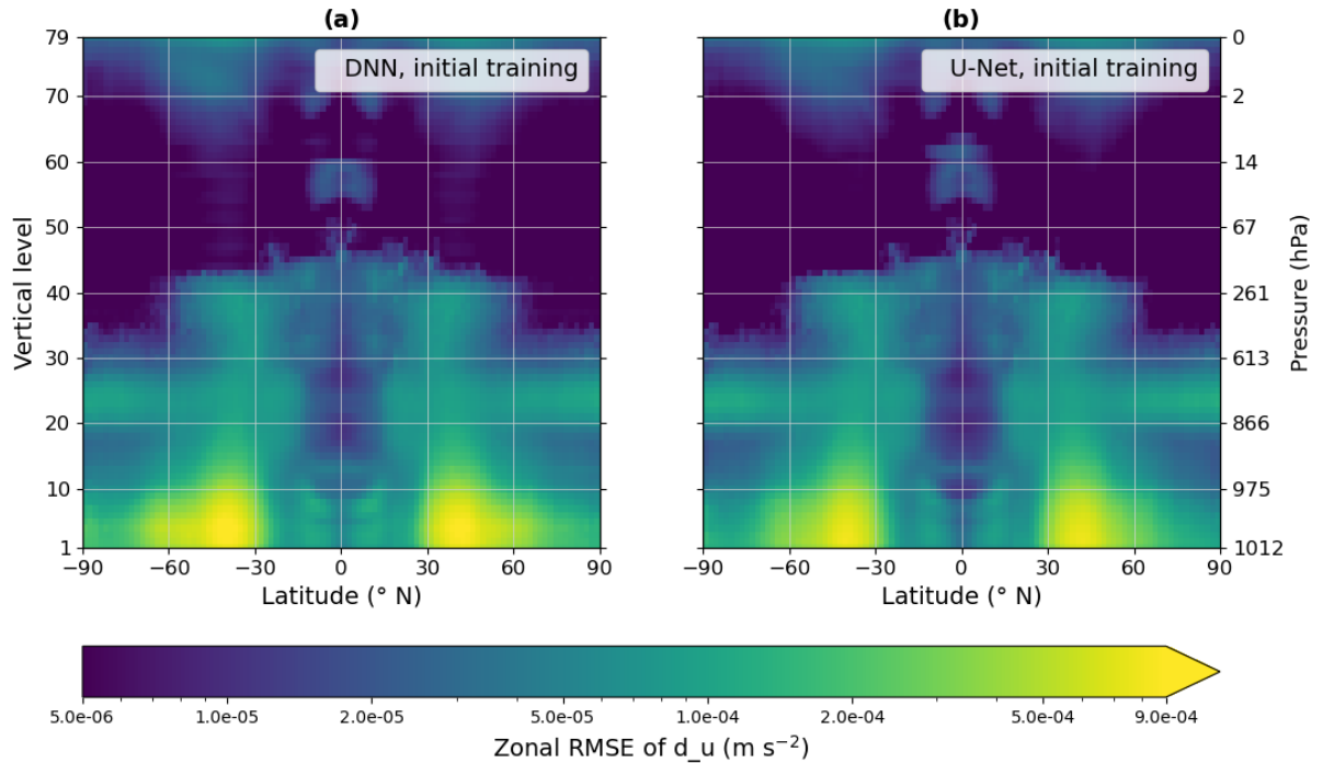
Figure 4. Cross-sections of the zonal RMSE of the zonal wind tendency d_u for the test subset. Figures (a) and (b) show the results, from the DNN (a) and from the U-Net respectively, from (b) with the initial approach in both cases, whereas figures (c) and (d) are the results of the DNN and the U-Net, with laplacians. Figures (e) and (f) are respectively the zonal RMSE differences between DNN with laplacians (e) and DNN without them (a), and U-Net with laplacians (d) and U-Net without them (b). The colorbar displays data on a logarithmic scale.
