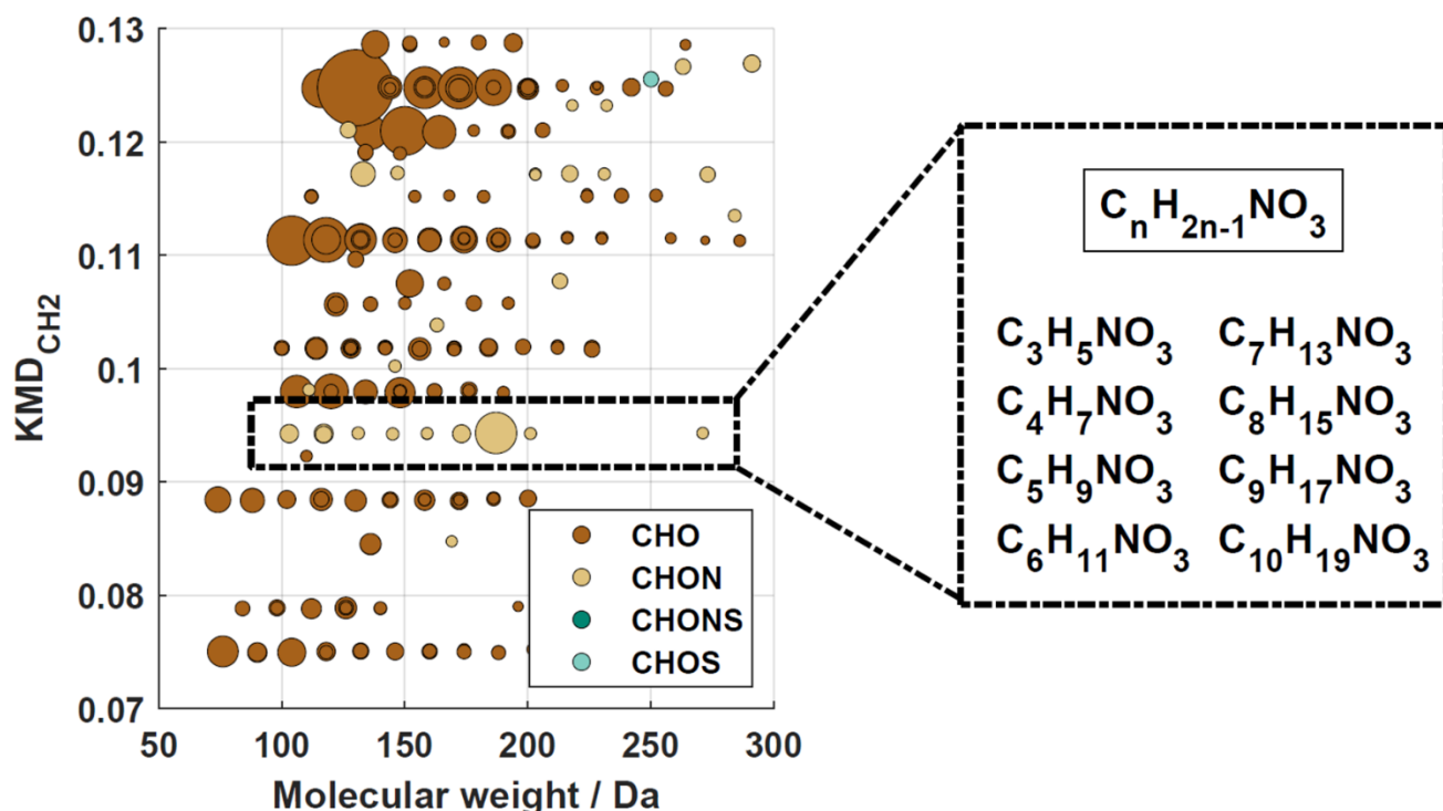
720 Figure 7: Kendrick mass defect diagram for the dry season 2018. The size of the data points represents the signal intensity of the corresponding peak. The four subgroups are distinguished with different colors. The dashed box highlights a homologous series of CHON compounds with a molecular formula of C n H 2n-1 NO 3 with n = (3 – 17), potentially related to biomass burning emissions.
