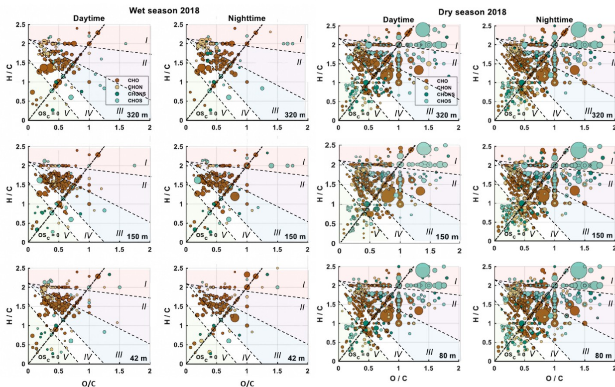
Figure 3: Van Krevelen plots from the wet season 2018 (left panel) and dry season 2018 (right panel) during daytime and nighttime at 42 m, 150 m, 320 m height and 320 m height and dry season 2018 (right panel) during daytime and nighttime at 80 m, 150 m, and 320 m height. Included are only molecular formulae that were present in more than one of the samples, respectively. The background signals are subtracted. The size of the data points represents the signal intensity of the corresponding peak. The four subgroups CHO, CHON, CHONS and CHOS are distinguished with different colors. Compounds located on the black dashed line have an average carbon oxidation state of 0 ( OSC = 0 ). The VK diagram was divided into five areas: I for very highly oxidized organic compounds, II for highly oxidized compounds, III for intermediately oxidized compounds, IV for oxidized unsaturated organic compounds and V for highly unsaturated organic compounds. The five areas were defined according to Zhang et al., 2021. Area (I) is mainly characterized by CHOS molecules with at least one sulfate functional group and C4 and C5 backbones. Area (II) is dominated by highly oxidized compounds representing aged OA and biomass burning products. Area (III) shows mainly aliphatic species. Area (IV) is dominated by unsaturated hydrocarbons with low oxygen content and aromatic structures while area (V) shows mainly combustion related species.
