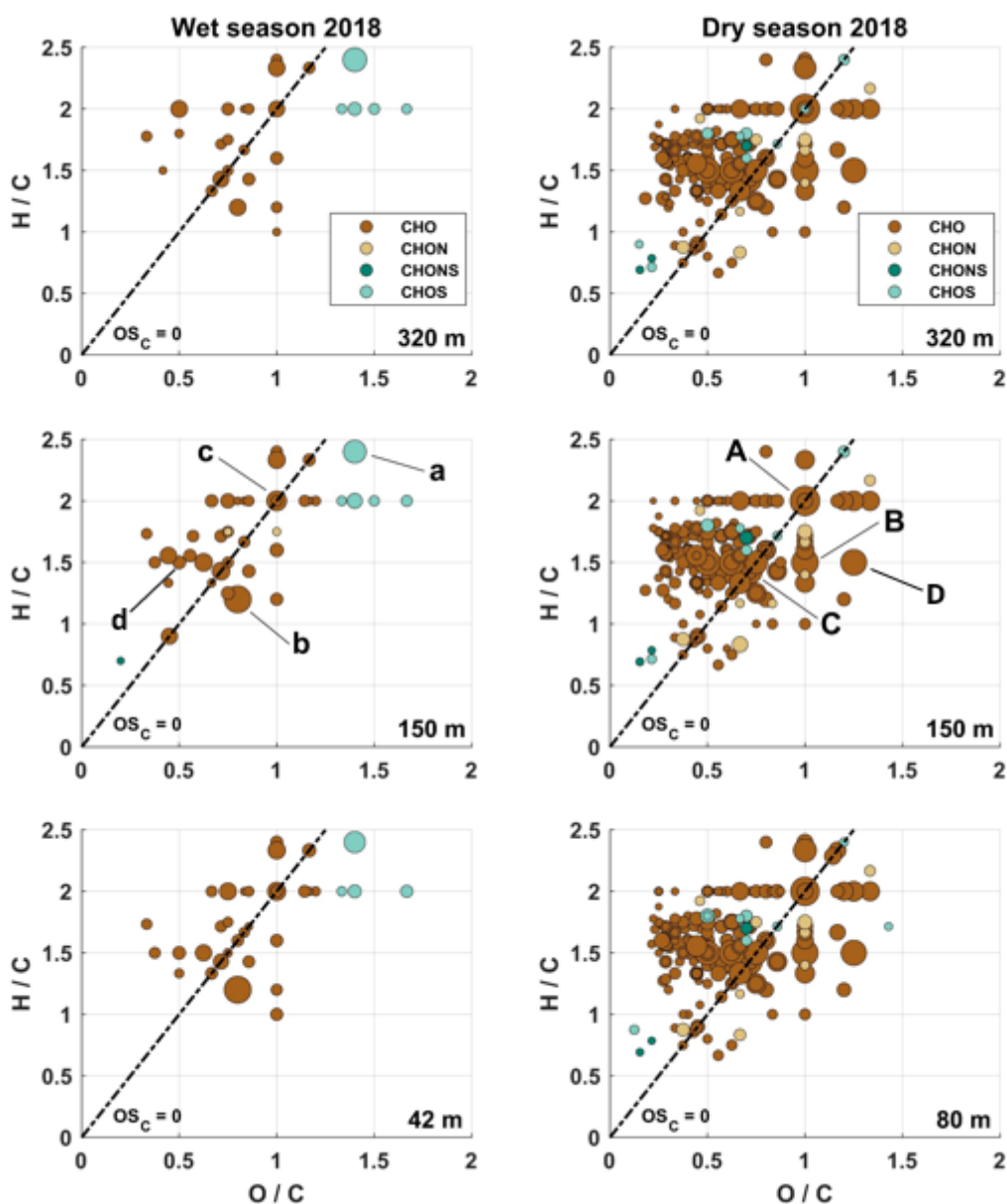
Figure 1: Van Krevelen plots from the wet season 2018 (left panel; sampling heights: 320 m, 150 m, 42 m) and the dry season 2018 (right panel; sampling heights: 320 m, 150 m, 80 m). Included are only molecular formulae that were present in more than 75% of the samples, respectively. The size of the data points represents the signal intensity of the corresponding peak. The four subgroups are distinguished with different colors. Compounds located on the black dashed line have an average carbon oxidation state of 0 (OSC = 0). The labels a-d and A-D correspond to the most intense signals further characterized in Table II.
