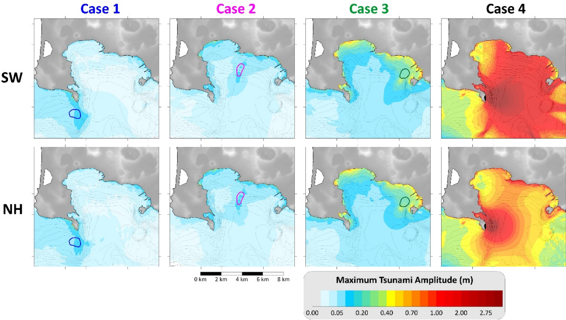
383 Figure 8. Maximum water amplitude on each node of the computational grid for the four scenarios considered: each of them are 384 simulated through the shallow-water (SW) and the Boussinesq (NH) approach. The coloured boundaries report the initial position 385 of the respective landslide source.
