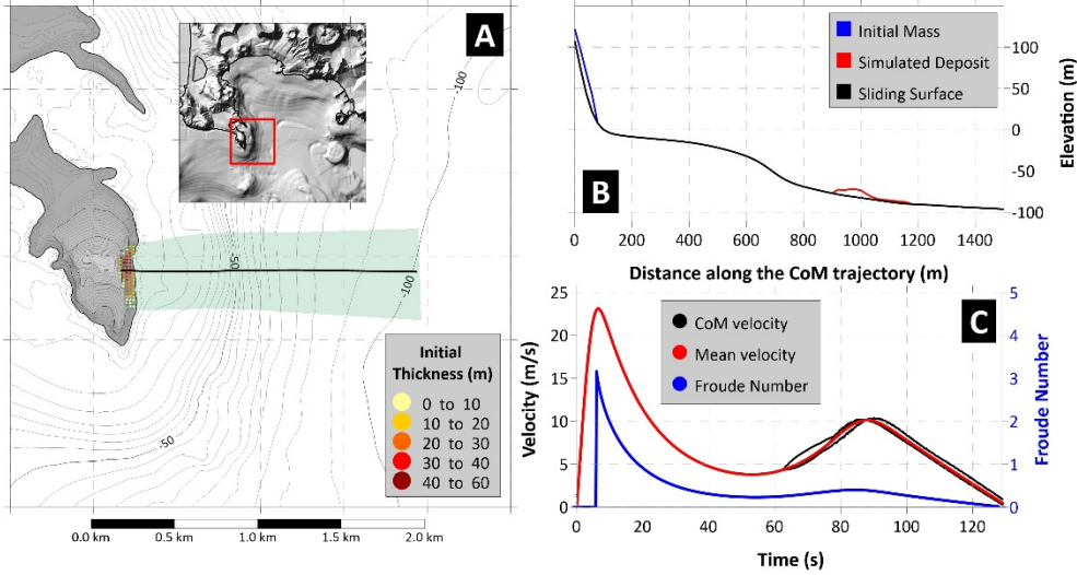
356 357 Figure 7. Panel A) Map of the initial sliding mass for Scenario 4, with initial thickness shown by the yellow-red scale. The black line 358 marks the CoM predefined trajectory. The area swept by the sliding motion is highlighted in green. Panel B) Landslide profile along 359 the CoM trajectory: in black the undisturbed sliding surface; in blue the initial mass; in red the simulated deposit. Panel C) Sliding 360 velocity (red for average, black for each CoM) and Froude Number (in blue) time histories.
