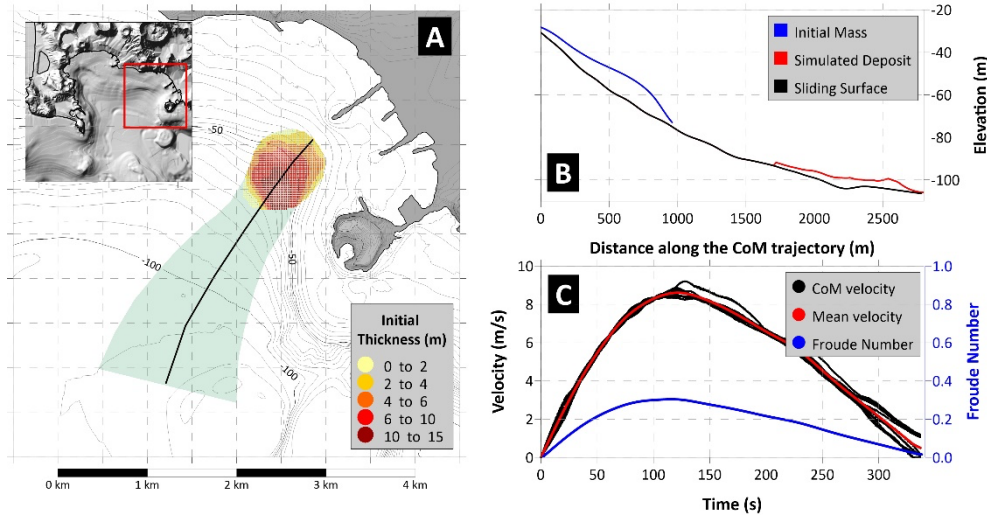
337 Figure 6. Panel A) Map of the initial sliding mass for Scenario 3, with initial thickness shown by the yellow-red scale. The black line 338 marks the CoM predefined trajectory. The area swept by the sliding motion is highlighted in green. Panel B) Landslide profile along 339 the CoM trajectory: in black the undisturbed sliding surface; in blue the initial mass; in red the simulated deposit. Panel C) Sliding 340 velocity (red for average, black for each CoM) and Froude Number (in blue) time histories.
