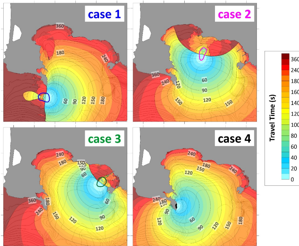
442 443 Figure 11. Travel time, in seconds, of the tsunamis generated by the four landslide scenarios here hypothesized. The position of the 444 initial mass is marked by the respective coloured boundaries.
