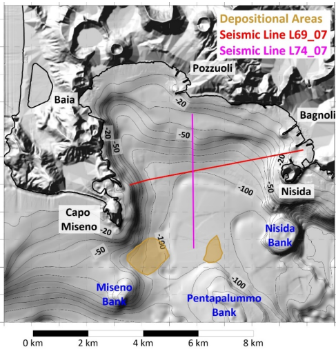
233 234 Figure 2. Morphological map of the Gulf of Pozzuoli. Black labels denote the main coastal toponyms, blue ones the submarine 235 volcanic edifices. The brown contours mark the recognized depositional areas; the red and magenta lines report the seismic line 236 called L69_07 and L74_07 respectively. Such features are retrieved from Aiello et al. (2012).
