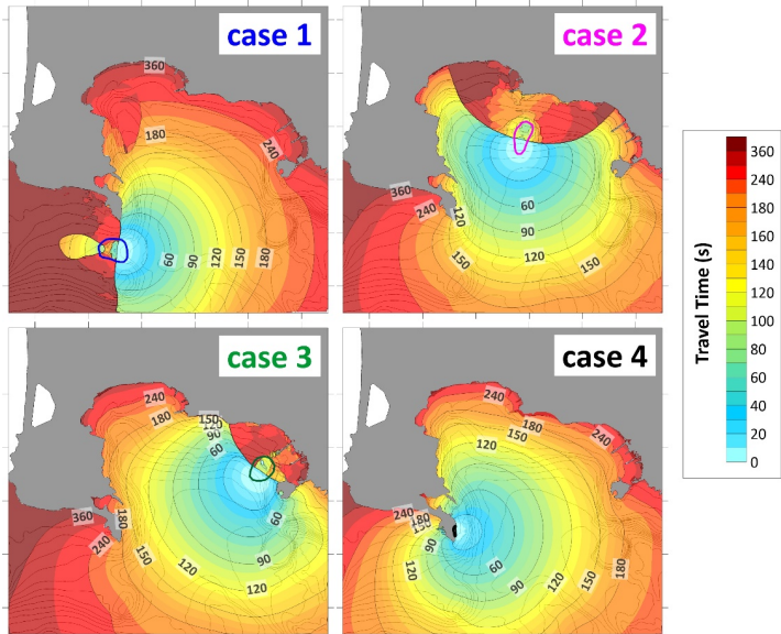
458 Figure 11. Travel time, in seconds, of the tsunamis generated by the four landslide scenarios here hypothesized. The position of the 459 initial mass is marked by the respective coloured boundaries. 460
