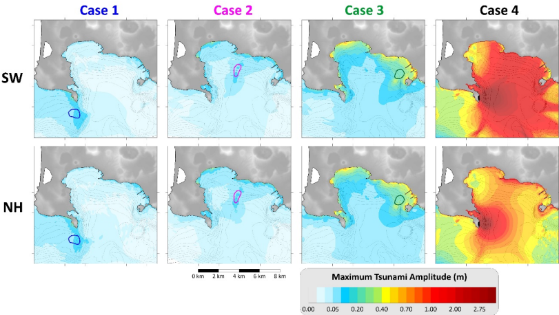
397 398 Figure 8. Maximum water amplitude on each node of the computational grid for the four scenarios considered: each of them are 399 simulated through the shallow-water (SW) and the Boussinesq (NH) approach. The coloured boundaries report the initial position 400 of the respective landslide source.
