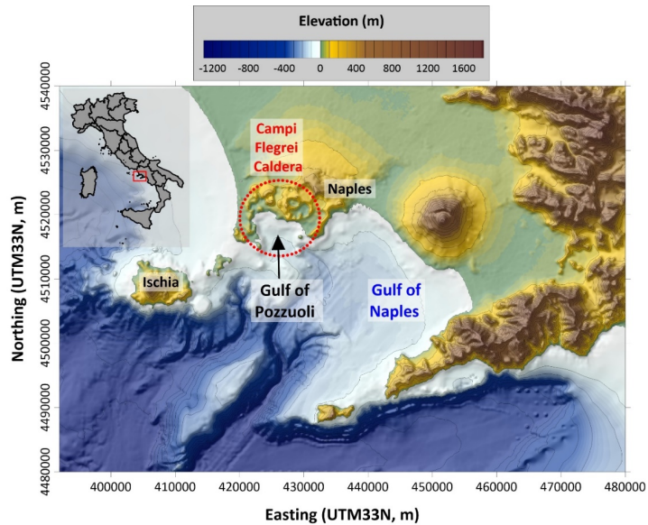
82 83 Figure 1. Morphological map of the Gulf of Naples (South Italy). The red-dashed circle delimits approximately the Campi Flegrei 84 caldera, involving a subaerial part (west of Naples) and a submarine portion (Gulf of Pozzuoli).
