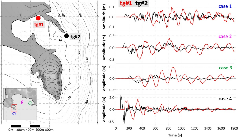
540 541 542 Figure 12. Virtual tide gauges at the entrance (in black) and inside (in red) the Bacoli Bay. On the left, their location; on the right, the comparison between the marigrams for the scenarios here simulated.
