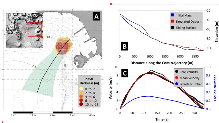
535 Figure 6. Panel A) Map of the initial sliding mass for Scenario 3, with initial thickness shown by the yellow-red scale. The black line 536 marks the CoM predefined trajectory. The area swept by the sliding motion is highlighted in green. Panel B) Landslide profile along 537 the CoM trajectory: in black the undisturbed sliding surface; in blue the initial mass; in red the simulated deposit. Panel C) Sliding 538 velocity (red for average, black for each CoM) and Froude Number (in blue) time histories.
