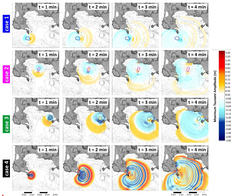
Figure 10. Propagation sketches at 1 minute intervals of the four landslide-tsunami scenarios investigated (NH approach). The yellow-red scale marks the positive values (sea level increase), the cyan-blue scale is for negative ones (sea level sinking). The coloured contours represent the respective initial landslide boundary.
