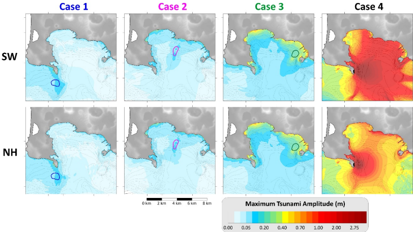
600 Figure 8. Maximum water amplitude on each node of the computational grid for the four scenarios considered: each of them are 601 simulated through the shallow-water (SW) and the Boussinesq (NH) approach. The coloured boundaries report the initial position 602 of the respective landslide source.
