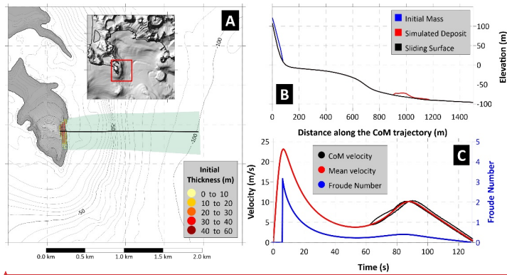
567 Figure 7. Panel A) Map of the initial sliding mass for Scenario 4, with initial thickness shown by the yellow-red scale. The black line 568 marks the CoM predefined trajectory. The area swept by the sliding motion is highlighted in green. Panel B) Landslide profile along 569 the CoM trajectory: in black the undisturbed sliding surface; in blue the initial mass; in red the simulated deposit. Panel C) Sliding 570 velocity (red for average, black for each CoM) and Froude Number (in blue) time histories.
