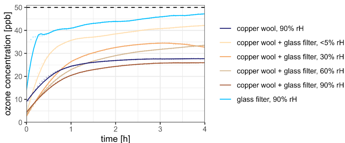
285 Figure 4. Progression of the ozone concentration downstream of the copper wool and clean glass filters at different relative humidity levels and an input ozone concentration of 50 \pm 3 ppb (dashed horizontal line) and a flow rate of 80 mL/min per filter over the course of 4 hours, representing a typical sampling duration. Only copper wool (dark blue graph) and only clean glass filters (light blue line) were used as reference.
