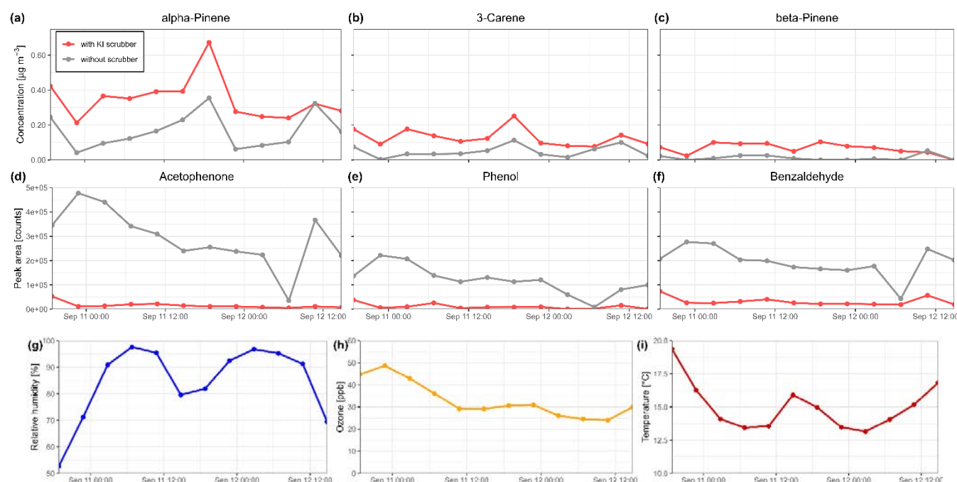
Figure 7. Temporal variations in monoterpene concentrations (a – c), peak areas of Tenax degradation products (d – f) and environmental parameters (g – i) across the sampling period, using a potassium iodide ozone scrubber (red) and without the scrubber (grey). The results demonstrate that the ozone scrubber enhances the measured concentrations of forest monoterpenes and reduces the formation of degradation products of the sorbent material, indicating effective prevention of reactions of adsorbed monoterpenes and sorbent material with ozone.
