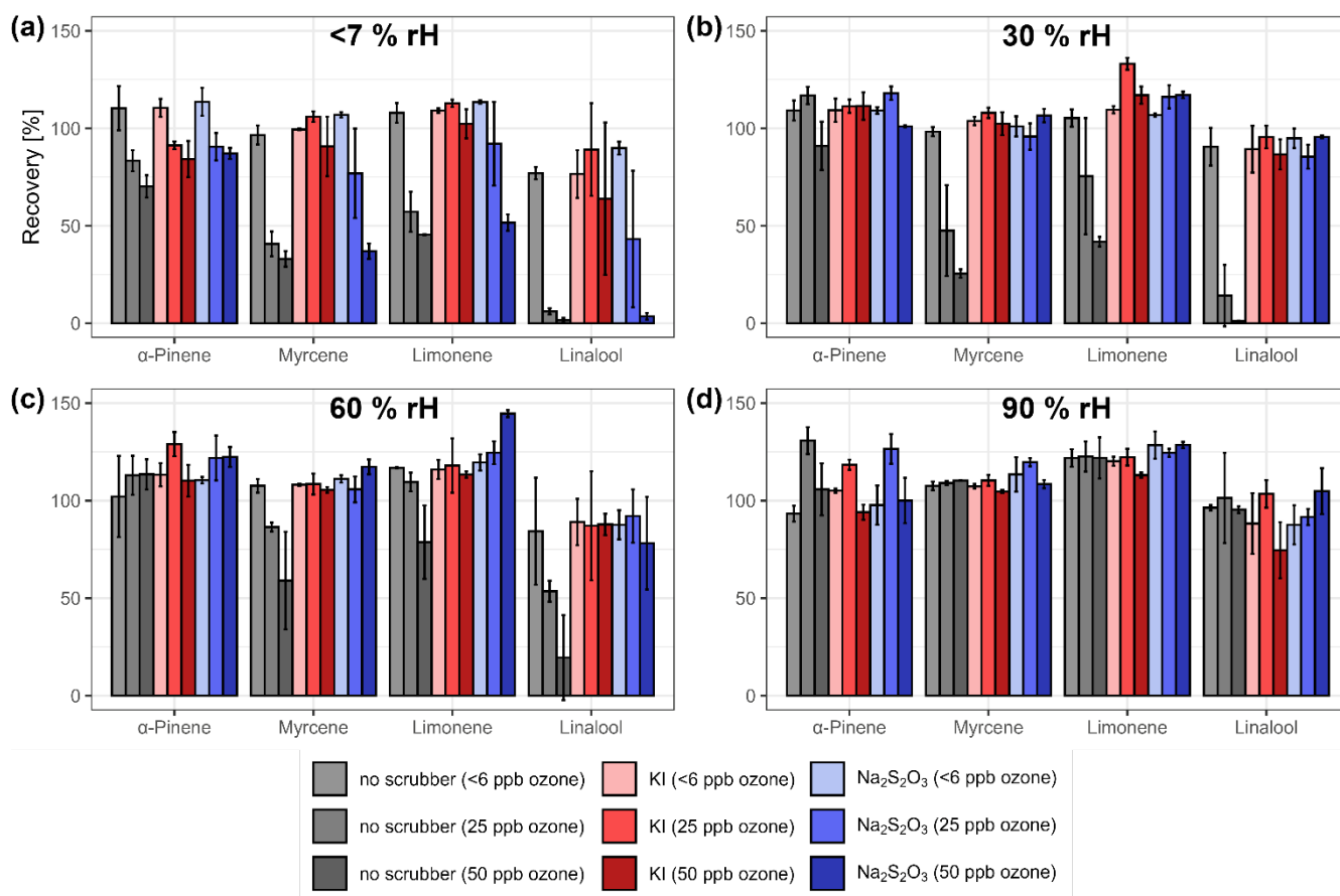
Figure 5. Mean recovery rates ( \pm standard deviation) of \alpha -Pinene, Myrcene, Limonene and Linalool for the load-and-flush approach at relative humidity levels of (a) <7 %, (b) 30 %, (c) 60 % and (d) 90 %. Grey bars represent unfiltered samples, red bars potassium iodide filters and blue bars sodium thiosulfate filters.
