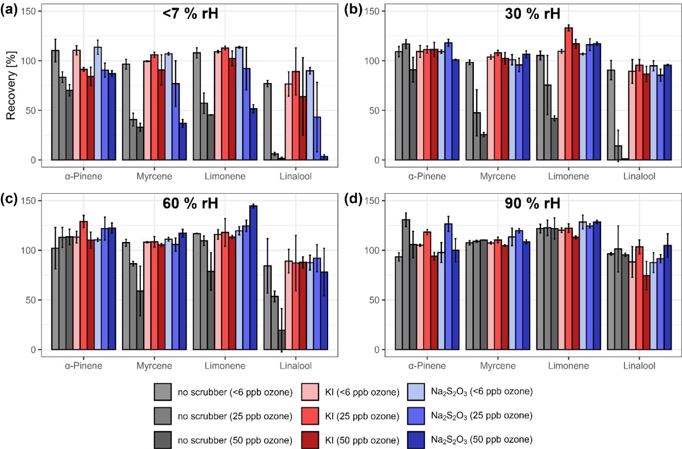
350 Figure 5. Mean recovery rates (± standard deviation) of α-Pinene, Myrcene, Limonene and Linalool for the load-and-flush approach at relative humidity levels of (a) <7 %, (b) 30 %, (c) 60 % and (d) 90 %. Grey bars represent unfiltered samples, red bars potassium iodide filters and blue bars sodium thiosulfate filters.
