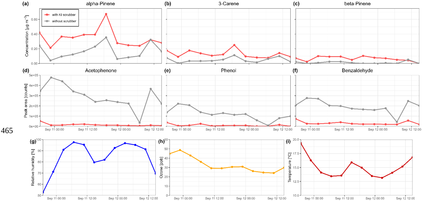
470 Figure 7. Temporal variations in monoterpene concentrations (a – c), peak areas of Tenax degradation products (d – f) and environmental parameters (g – i) across the sampling period, using a potassium iodide ozone scrubber (red) and without the scrubber (grey). The results demonstrate that the ozone scrubber enhances the measured concentrations of forest monoterpenes and reduces the formation of degradation products of the sorbent material, indicating effective prevention of reactions of adsorbed monoterpenes and sorbent material with ozone.
