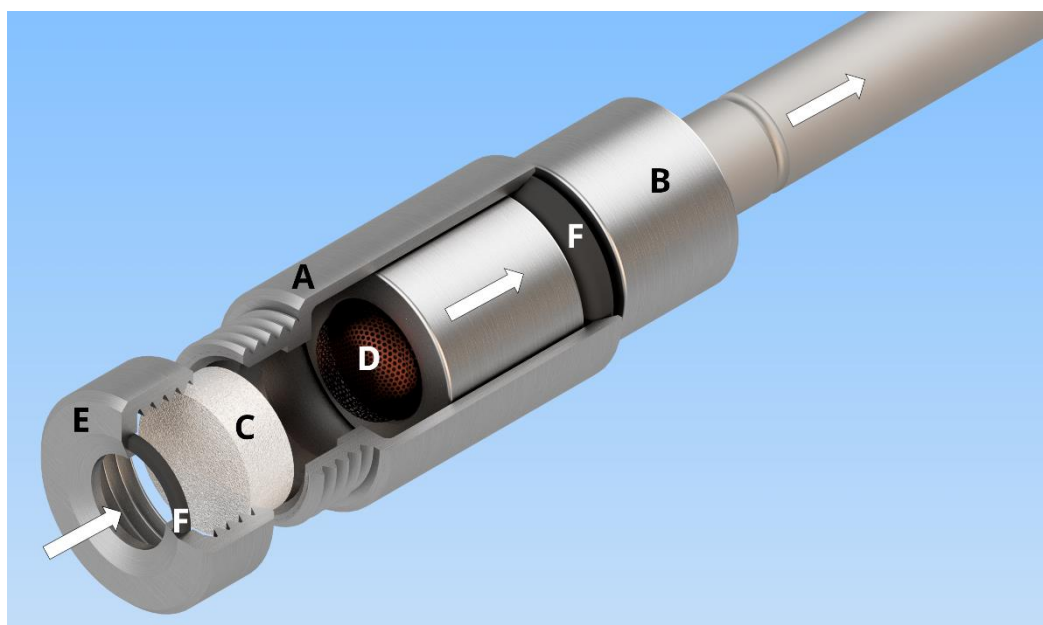
120 Figure 1. Schematic layout of the ozone scrubber. The scrubber housing (A) was designed to fit on a commonly used diffusion-locking cap (B). Sample air flows from the left to the right, passing both a loaded glass filter as ozone scrubber (C) and copper wool (D). A screw cap (E) facilitates the quick and easy exchange of the filter. Two O-rings (F), located between the screw cap and the filter and between the housing and the diffusion-locking cap, prevent sampled air from bypassing the filter. Arrows indicate the direction of the air flow through the ozone filter.
