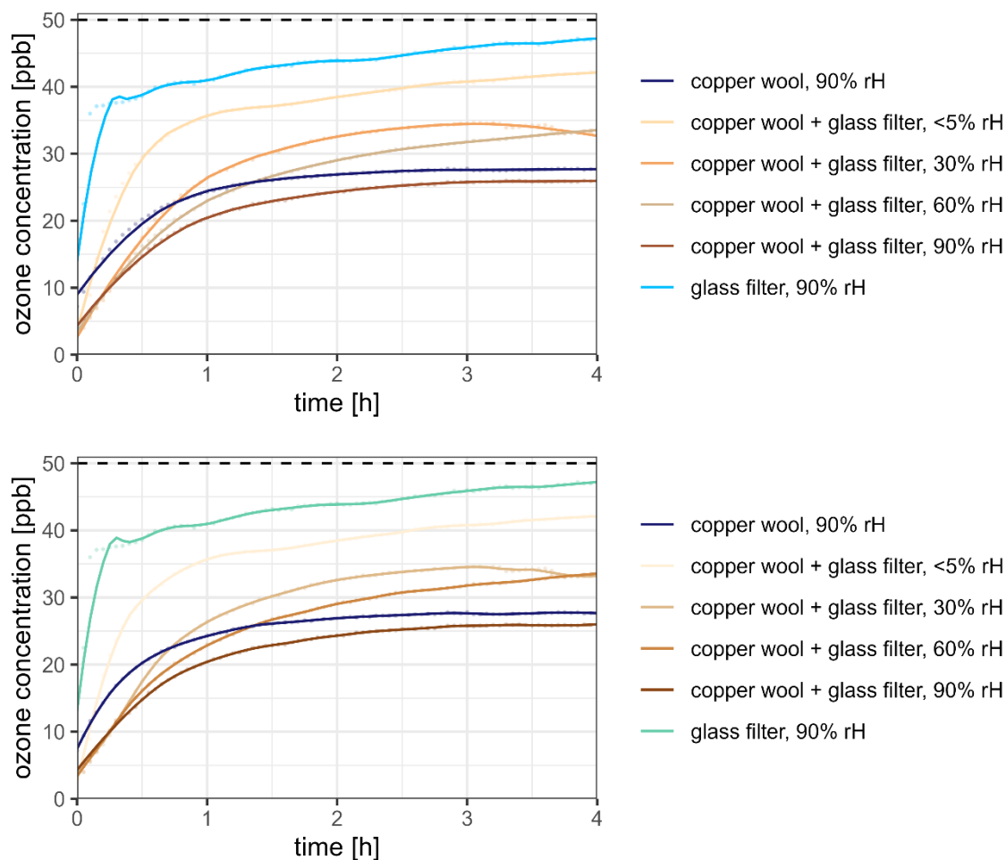
Figure 4. Progression of the ozone concentration downstream of the copper wool and clean glass filters at different relative humidity levels and an input ozone concentration of 50 \pm 3 ppb (dashed horizontal line) and a flow rate of 80 mL/min per filter over the course of 4 hours, representing a typical sampling duration. Only copper wool (dark blue graph) and only clean glass filters (light blue line) were used as reference.
