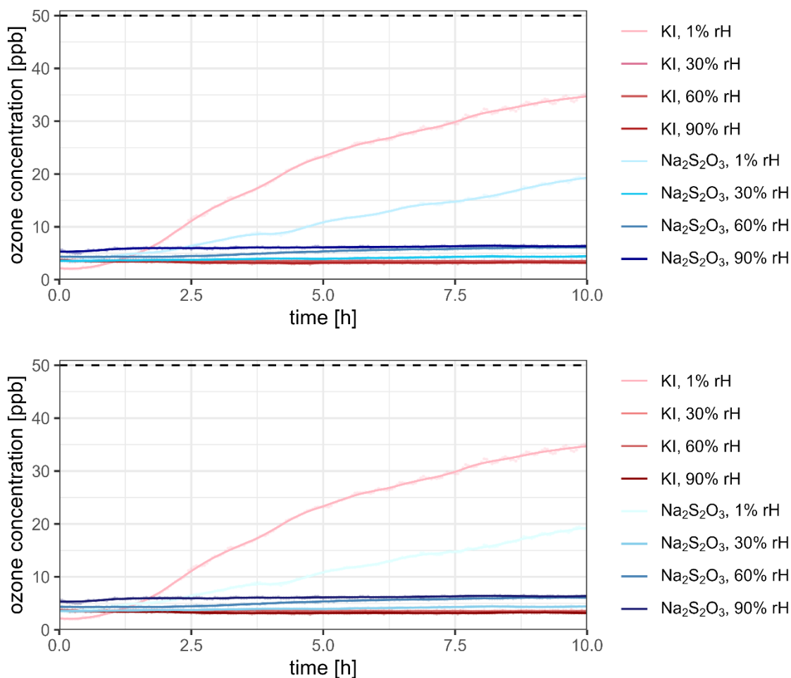
Figure 2. Progression of the ozone concentration downstream of the ozone scrubbers at different relative humidity levels and an input ozone concentration of 50 \pm 3 ppb (dashed horizontal line) and a flow rate of 80 mL/min per filter. Potassium iodide (KI, red graphs) and Sodium thiosulfate (Na 2 S 2 O 3 , blue graphs) were used as scrubber materials.
