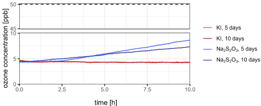
275 Figure 3. Progression of the ozone concentration downstream of the ozone scrubbers at 60% relative humidity and an input ozone concentration of 50 \pm 3 ppb (dashed horizontal line) and a flow rate of 80 mL/min per filter, over the course of 10 hours. Potassium iodide (KI, red graphs) and Sodium thiosulfate ( \text{Na}_2\text{S}_2\text{O}_3 , blue graphs) scrubbers were stored under environmental conditions for 5 and 10 days before the breakthrough tests.
