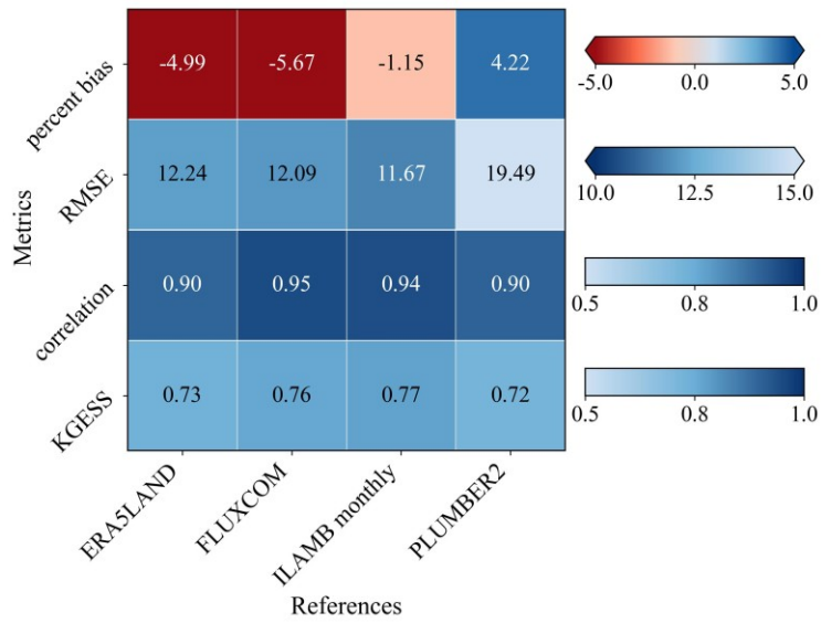
535 Figure 9: Evaluation of latent heat flux simulated by CoLM2024 using various metrics with different reference datasets.
