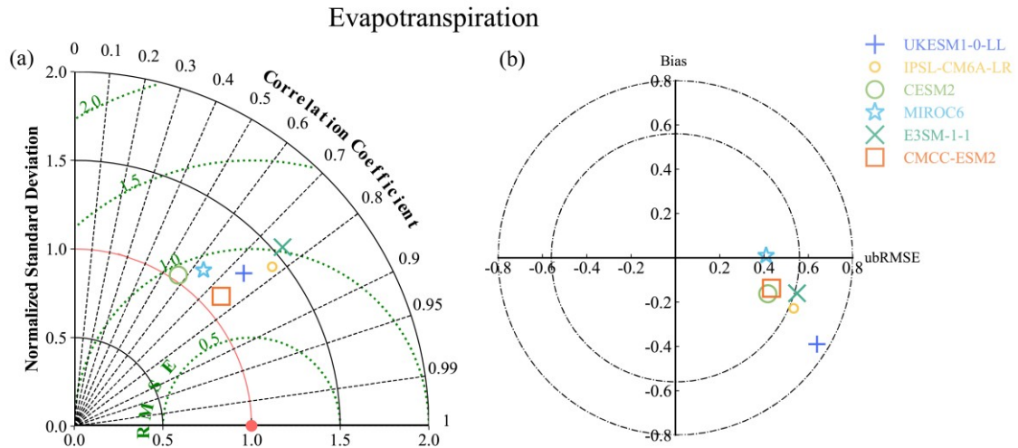
540 Figure 10: The Taylor (a) and target diagram (b) for comparing evapotranspiration among the six models in LS3MIP.
