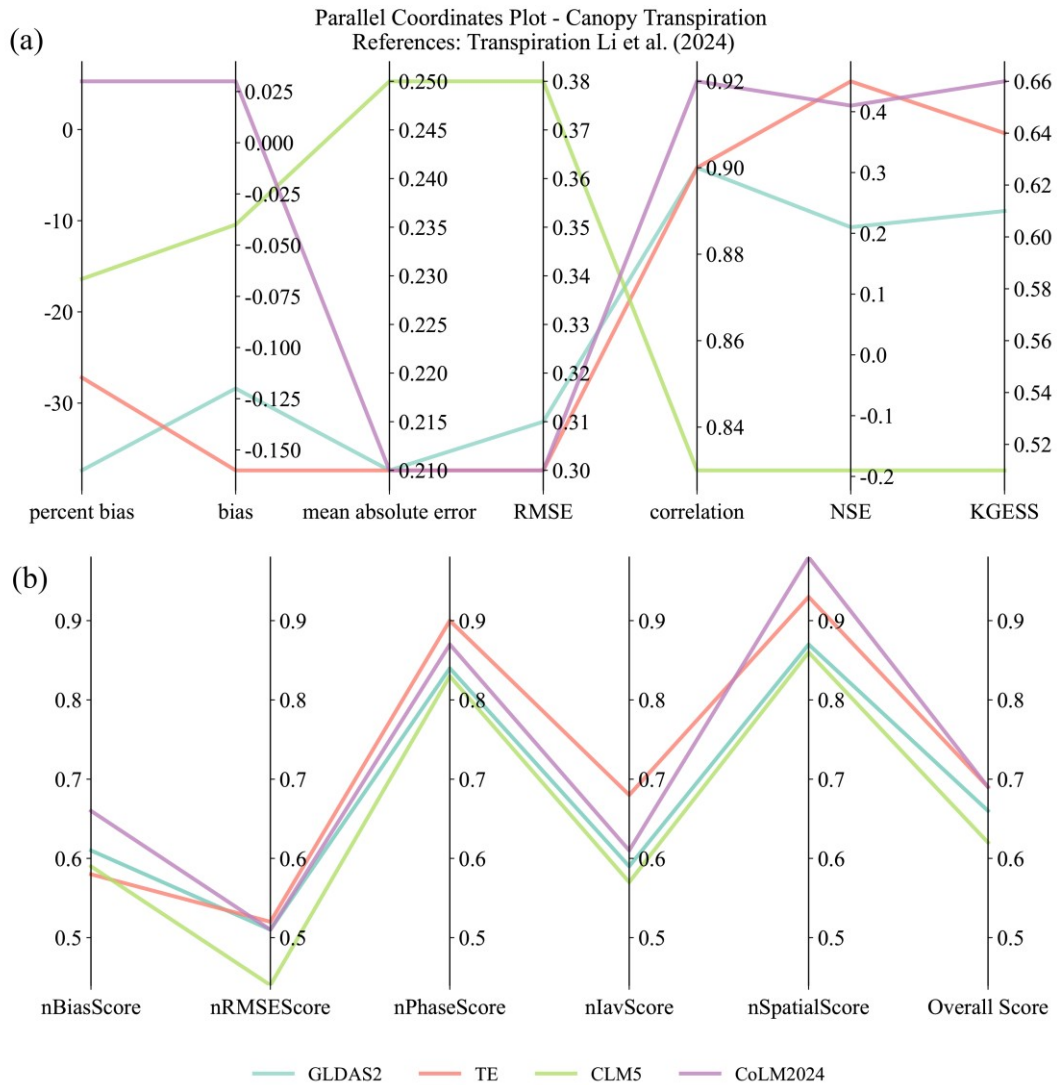
480 Figure 7: Evaluation of canopy transpiration using various (a) metrics and (b) score indexes for GLDAS2, TE, CLM5, and CoLM2024.
