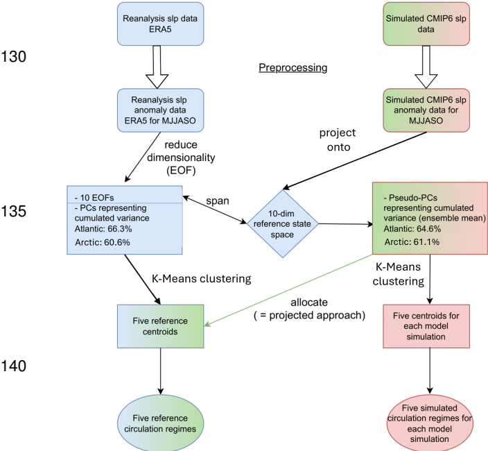
145 Figure 1. Chart flow of computation of atmospheric circulation regimes. The blue pathway indicates the approach to calculate reference circulation regimes. The red pathway shows the procedure to calculate simulated circulation regimes, the green pathway represents the projected regimes.
