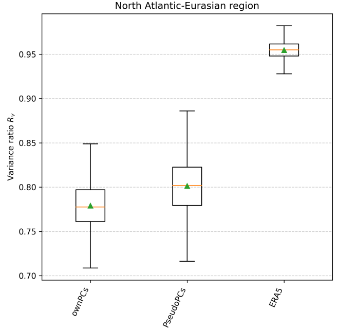
Figure A1. Variance ratio for Common circulation regime data projected onto reference state space (Pseudo PCs) and its own state space (own PCs) as well as ERA5. The box plots refer to the distribution of 15-yr bootstraps ( n=1000 ) of each model and show mean (triangle), median (horizontal line), first and third quartile (boxes) and 10 and 90 percentiles (bars).
