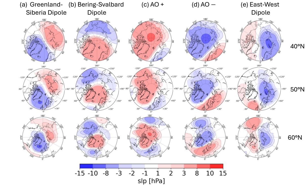
Figure D1. Reference circulation regimes ERA5 for the Arctic region in the historical time period 1985-2014 for different constraints calculated by the KME algorithm in the extended boreal summer season from May to October
