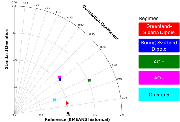
Figure 10. Taylor diagram comparing the future common simulated regimes for the CMIP6 ensemble for SSP5-8.5 and the period 2070–2099 to the corresponding reference regimes from ERA5 reanalysis in the historical period (1985–2014), for the Arctic region. Spatial regime patterns determined with K-Means clustering
