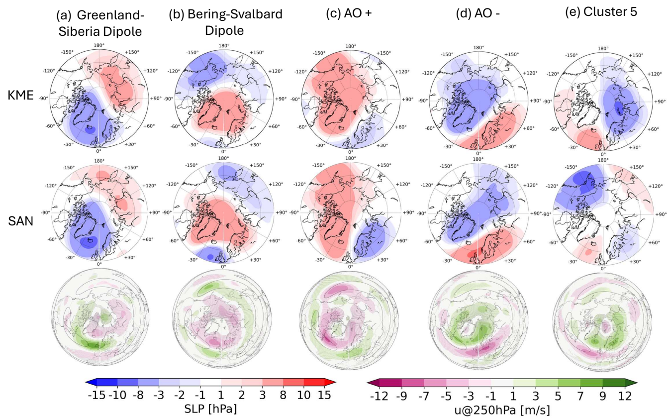
Figure 8. Reference circulation regimes for the Arctic region in the historical time period (1985-2014) from the ERA5 reanalysis dataset, calculated by the K-Means Clustering ( KME ) and simulated annealing and diversified randomisation clustering ( SAN ) algorithms. In the lower row the zonal wind anomaly composites for KME regimes at 250 hPa are shown, the SAN wind composites indicate similar anomalies except for Cluster 5.
