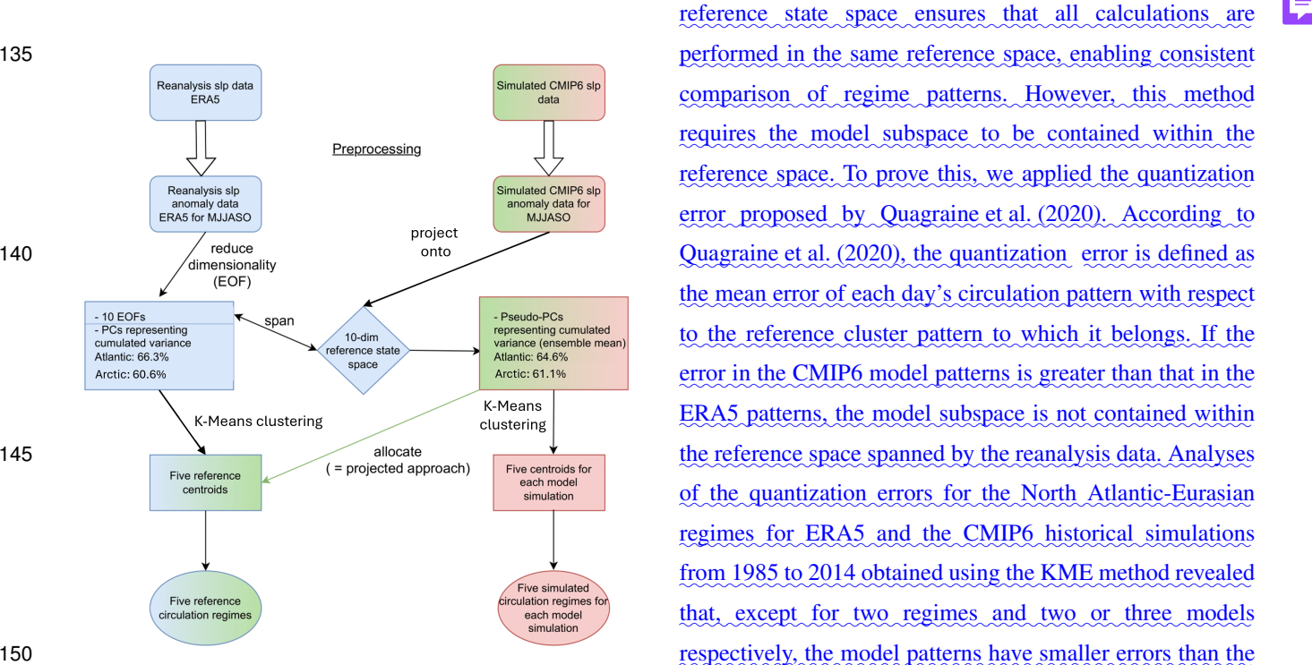
Figure 1. Chart flow of computation of atmospheric circulation regimes. The blue pathway indicates the approach to calculate reference circulation regimes. The red pathway shows the procedure to calculate simulated circulation regimes, the green pathway represents the projected regimes.
