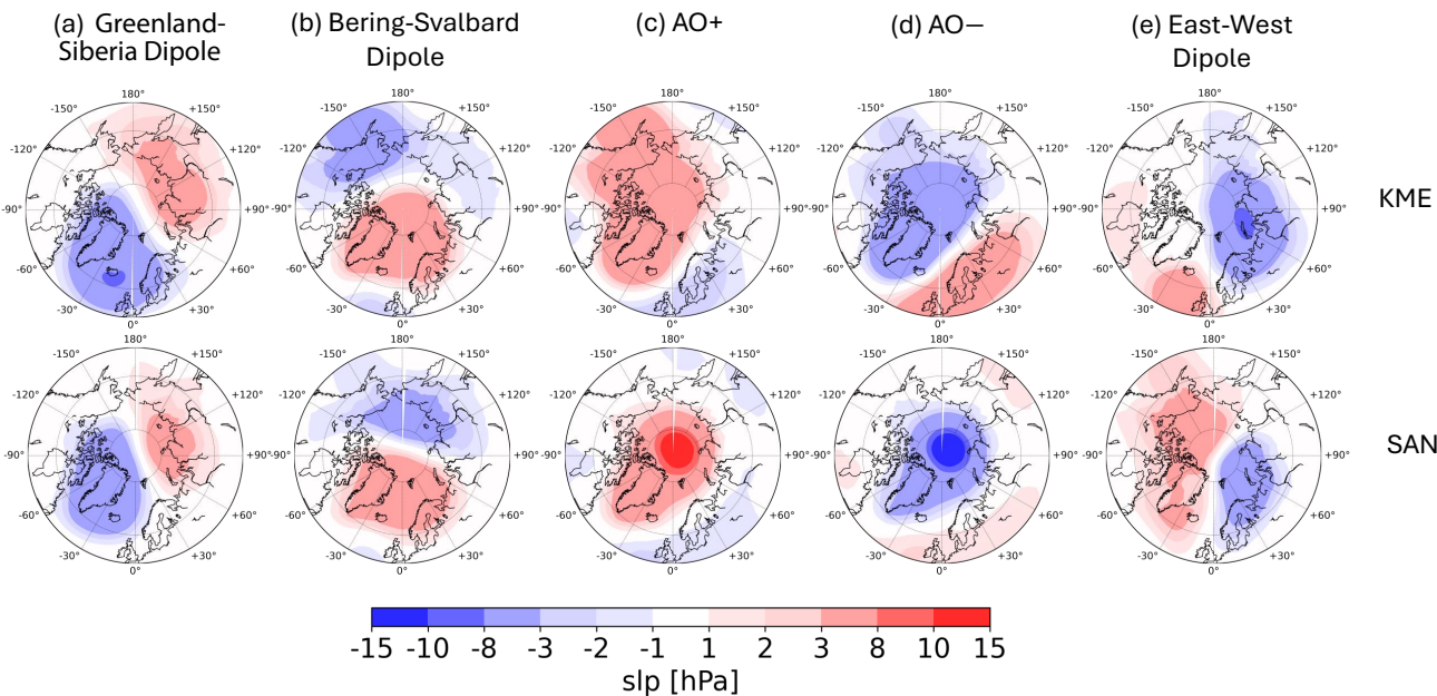
Figure 7. Reference circulation regimes for the Arctic region in the historical time period (1985-2014) from the ERA5 reanalysis dataset, calculated by the K-Means Clustering ( KME ) and simulated annealing and diversified randomisation clustering ( SAN ) algorithms.
