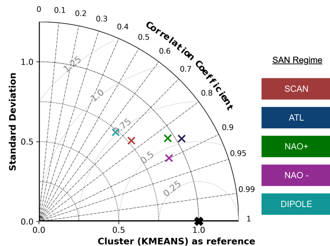
Figure 3. Taylor diagram analysis of circulation regimes computed by KME and SAN algorithms in the historical period for the North Atlantic-Eurasian region in extended boreal summer season from May to October. The reference circulation regimes computed from ERA5 reanalysis data with KME is marked as black cross, the colored crosses represent the SAN regimes.
