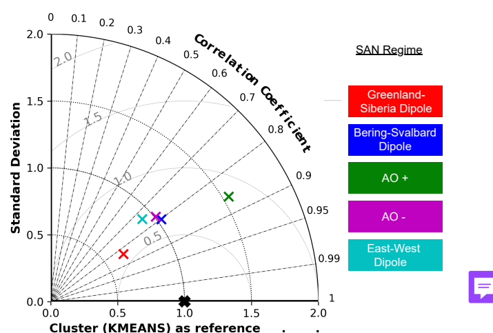
Figure 8. Taylor diagram analysis of circulation regimes computed by KME and SAN algorithms in the historical period for the Arctic region in extended boreal summer season from May to October. The reference circulation regimes computed from ERA5 reanalysis data with KME is marked as black cross. The colored crosses represent the respective regime calculated from SAN algorithm.
