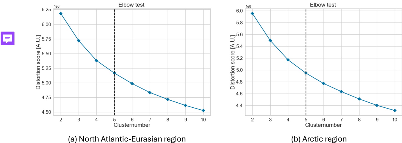
Figure B1. Distortion score of the dataset considered for the respective region. The row specifies the investigated region, the column shows the results for different numbers of clusters
