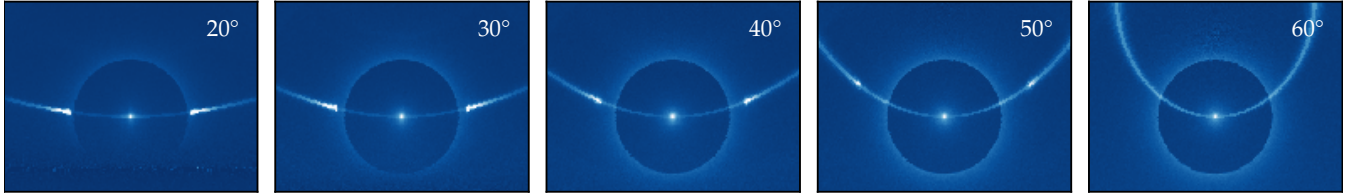
Figure 9. Sundogs for increasing solar elevations, calculated with CrystalTrace.
