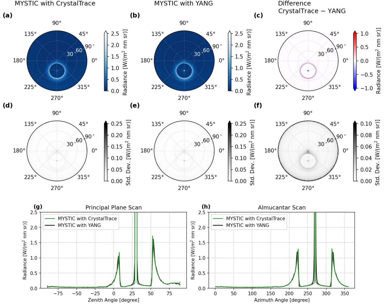
Figure 7. Comparison of simulated radiances for a cirrus cloud of optical thickness 1 with randomly oriented ice crystals using optical properties of the YANG database and CrystalTrace for \text{AR} = 14.4 with D = 10^4 \mu\text{m} at a wavelength of 550 nm. The simulations were performed with 4 \times 10^7 photons at a solar zenith angle of \theta_0 = 30^\circ and azimuth angle \phi_0 = 270^\circ , without atmospheric background. The top panel shows a polar projection of the simulated radiances with MYSTIC using (a) CrystalTrace and (b) the YANG look-up table to solve for the ice crystal single scattering properties. Panel (c) shows the difference between CrystalTrace and YANG and (d) – (f) show the corresponding standard deviation. The bottom panel displays cross sections through the polar plots along the principal (zenith angle transect along \phi = \phi_0 ) (g) and almucantar plane (azimuth angle transect along \theta = \theta_0 ) (h). Here, the MYSTIC radiances are computed using CrystalTrace are indicated by the green line and YANG in black.
