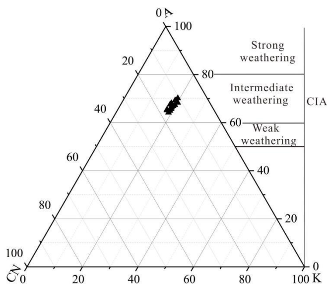
Figure 9. Ternary plots of Al_2O_3 - ( CaO^* + Na_2O )- K_2O (A-CN-K) in molar proportions that reflecting the intensity of weathering (based map from (Nesbitt and Young 1982)). Here CaO^* denotes the CaO content specifically within the silicate component.
