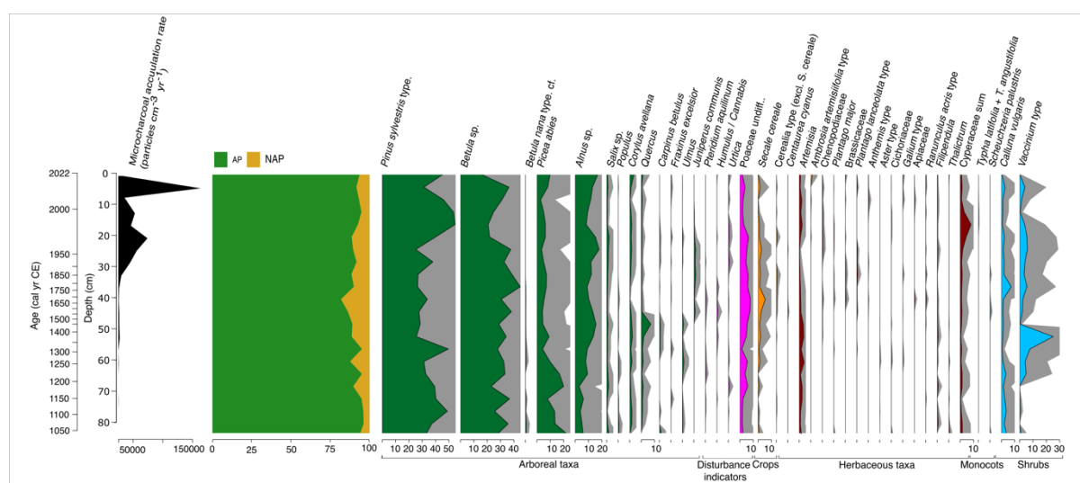
Figure 11. Stratigraphic plot illustrating the relative abundance of selected pollen taxa from core VAR1, as well as microcharcoal (expressed as the total number of counted fragments). Relative abundances of arboreal taxa are shaded green, disturbance indicators in pink, crops in orange, herbaceous taxa in brown and shrubs in teal. Grey shading represents 5x exaggeration. Only taxa with a minimum abundance of 2% are shown.
