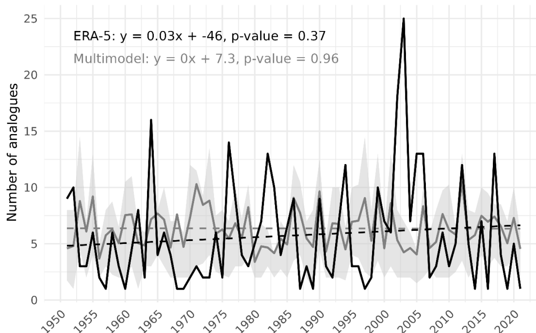
Figure A5. Annual frequency of analogue days based on geopotential height at 500 hPa (Z500) from 1950 to 2021, comparing ERA5 (black line) and the EURO-CORDEX multi-model ensemble (gray line with shading representing the inter-model spread across 25 EURO-CORDEX models based on 25th and 75th percentiles, respectively). Linear regression fits are shown for both ERA5 (dashed black line) and the multi-model ensemble (dashed gray line).
