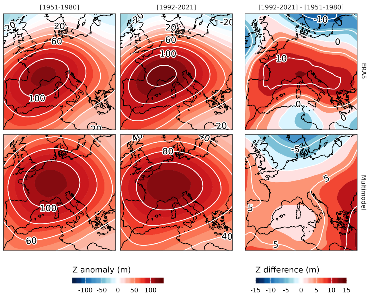
Figure A3. Geopotential height flow conditioned anomalies at 500 hPa (Z500) for the periods 1951–1980 (a, d) and 1992–2021 (b, e), and the differences between the two periods ([1992–2021] - [1951–1980], c, f). Panels (a–c) show ERA5-based reconstructions, while panels (d–f) display results from the top 5 EURO-CORDEX models, selected based on their analogue quality (Fig. S4).
