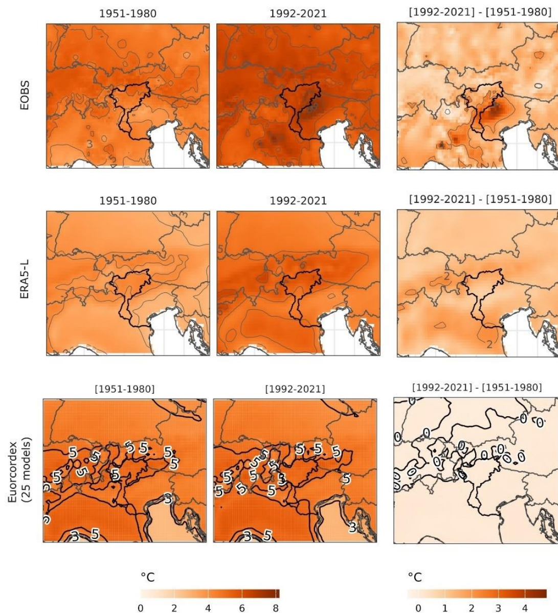
520 Figure A2. Spatial comparison of flow conditioned daily maximum temperature anomalies (TX) reconstructed for the periods 1951–1980 and 1992–2021, and the differences between these periods ([1992–2021] - [1951–1980]), based on three datasets: E-OBS (top row), ERA5-Land (middle row), and EURO-CORDEX ensemble mean (bottom row). The first two columns represent temperature anomalies for the two periods, while the third column shows the difference in anomalies.
