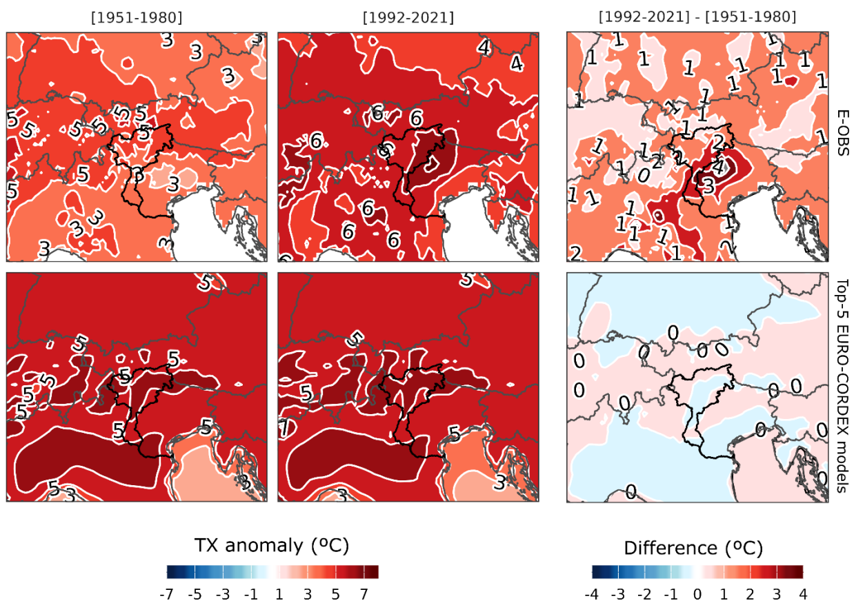
Figure A6. Same as Figure A3, but for TX. The observed reconstruction is derived from E-OBS.
